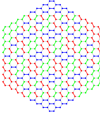
Figure 3.3: A Plane Partition can be seen as a dimer model in a hexagonal grid.
