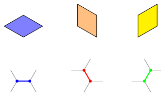
Figure 3.3 shows the translation of Figure 3.2 into a dimer configuration.
