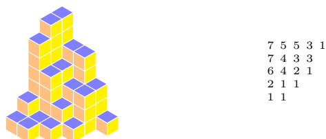
Figure 3.1: We can see a plane partition (PP) either as a stack of unit cubes pushed into a corner (at the left) either as array of decreasing numbers (at the right).
