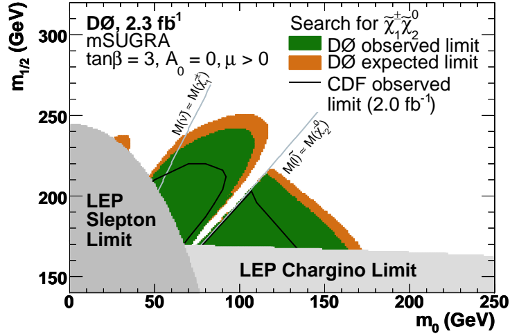
Figure 1.2: Region in the m_0 - m_{1/2} plane excluded by the D0 analyses (green), by LEP searches for charginos (light grey) and sleptons (dark grey) [13], and by CDF (black line) [14]. The assumed minimal supergravity parameters are A_0 = 0 GeV, \tan\beta = 3 and \mu > 0 [15].
