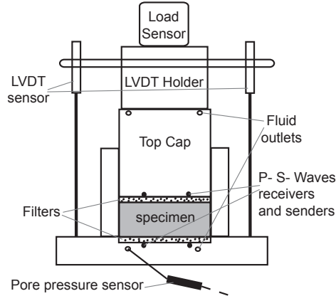
Figure 5.1: Schematic view of an oedometer cell. The top cap is made of titanium grade 5, the rest of the cell is made of stainless steel.
