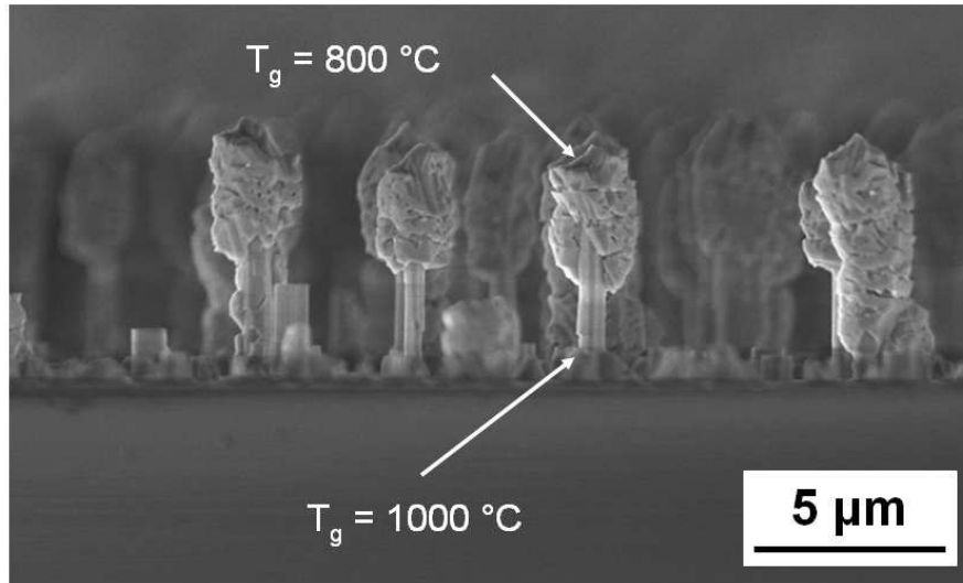
Figure 3.14 : Influence of a change of temperature during the wire growth. The temperature was stepwise reduced from 1000 to 800\text{ }^\circ\text{C} during growth (see text). The material quality is damaged at lower temperature forming tree-like structures.
