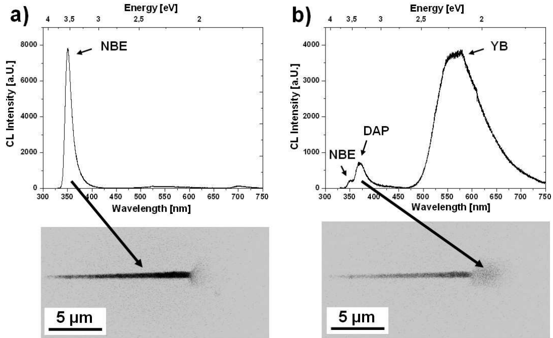
Figure 4.5 : a) CL (5 K) spectra of the n-doped GaN wire with a strong near band edge emission. The CL image shows the emission at 350 nm. b) CL spectra of the top of the wire grown under Cp_2Mg injection at 850 °C. The spectra show an emission peak at 370 nm three times stronger than the near band edge emission and a strong yellow band centred at 560 nm. The CL image shows the emission at 370 nm.
