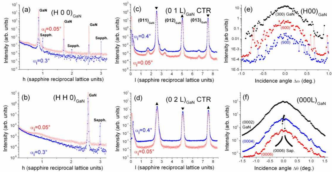
Figure 3.20 : X-ray diffraction measurements of GaN wires grown on c-sapphire. (a-b) In-plane grazing incidence X-ray diffraction measurements at two incidence angles ( \alpha_i=0.05, 0.3^\circ ) along the (a) [H 0 0] Sap. (resp. (b) [H H 0] Sap.) sapphire directions and corresponding to [H 0 0] GaN (resp. [H H 0] GaN) GaN lattice. (c-d) (0 1 L) and (0 2 L) crystal truncation rod.
