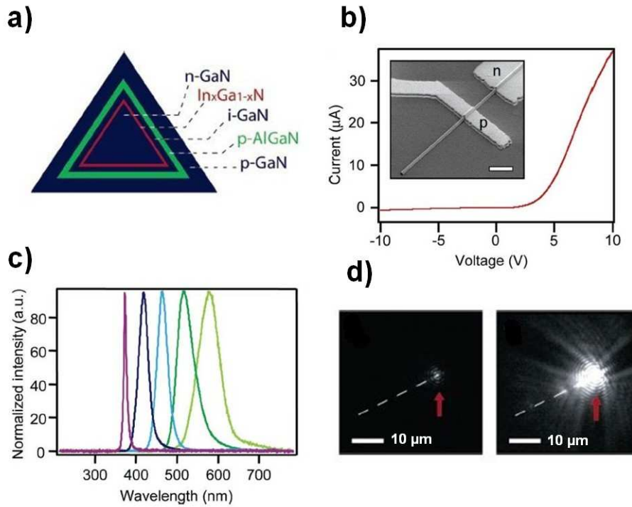
Figure 1.16: a) Schematic view of single nanowire LED structures based on an n-GaN core wire with InGaN/i-GaN/p-AlGaN/p-GaN shells, b) Connected wire with n- and p-pads and corresponding I-V curve, c) Normalised EL spectra for different In-concentrations, d) Optical microscopy images for 9 and 11 V forward bias [Qian05]
