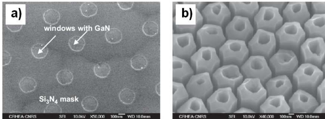
Figure 1.26: a) Patterned \text{Si}_3\text{N}_4 mask on GaN, b) GaN grown on the patterned \text{Si}_3\text{N}_4 layer [Cordier09]
