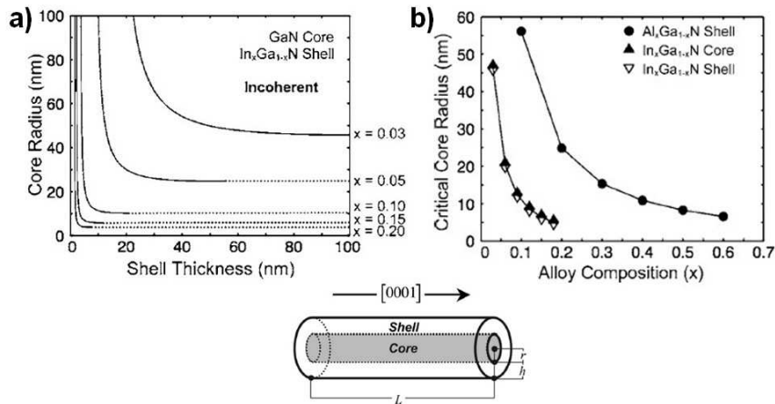
Figure 1.5: a) Limit between coherent and incoherent core/shell heterostructure. The GaN core radius is given as a function of the InGaN shell thickness for different indium concentrations. b) Critical core radius as function of the alloy composition for different core shell systems (black dots: GaN core – AlGa x N shell, black triangles: InGa x N core – GaN shell, white triangles: GaN core – InGa x N shell)
