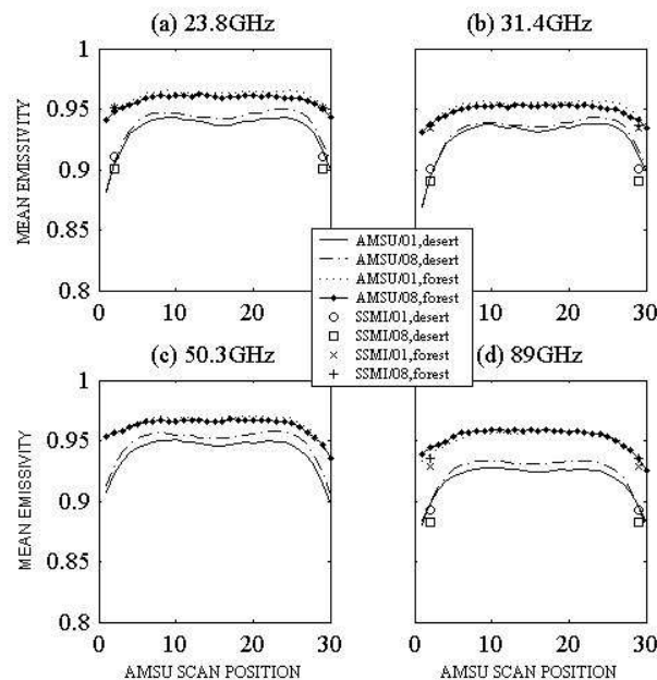
Figure 4: Monthly mean AMSU emissivities with respect to 30 scan positions ( \pm 58^\circ of zenith angle variation) and two surface types: desert (solid lines for January and dashed-dotted lines for August) and forest (dotted lines for January and solid-dotted lines for August): (a) at 23.8 GHz with SSMI emissivities at 53° and at 19 GHz, (b) same as (a) but at 31.4 GHz with SSMI emissivities at 37GHz, (c) same as (a) but at 50.3 GHz, (d) same as (a) but at 89 GHz with SSMI emissivities at 85 GHz.
