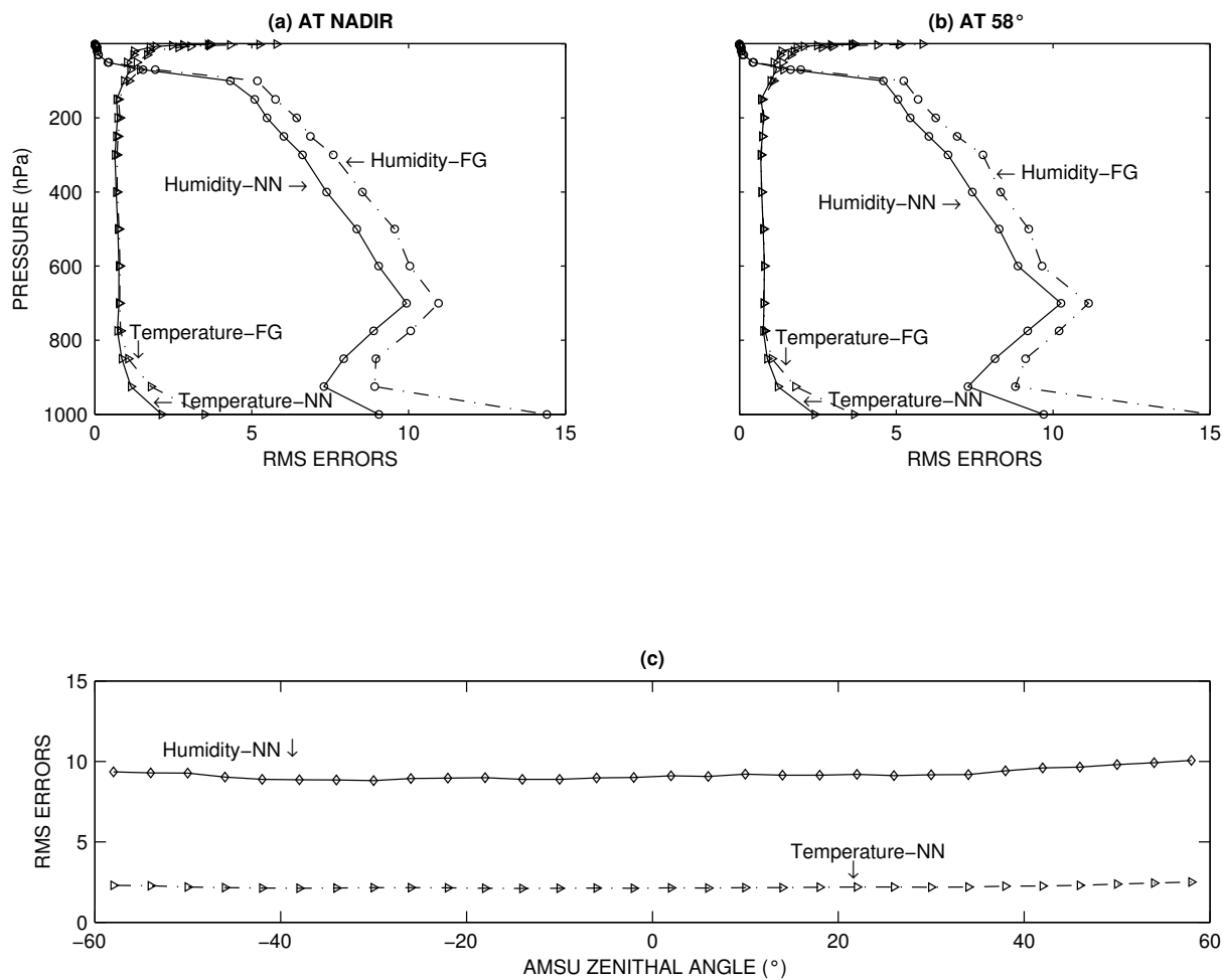
Figure 7: (a) Temperature and humidity RMS error profiles for nadir situations; both FG and NN error profiles are shown, (b) same as (a) but at 58° zenith angle (c) NN RMS errors at 1000 hPa level for both temperature and humidity sorted by AMSU zenith angle.
