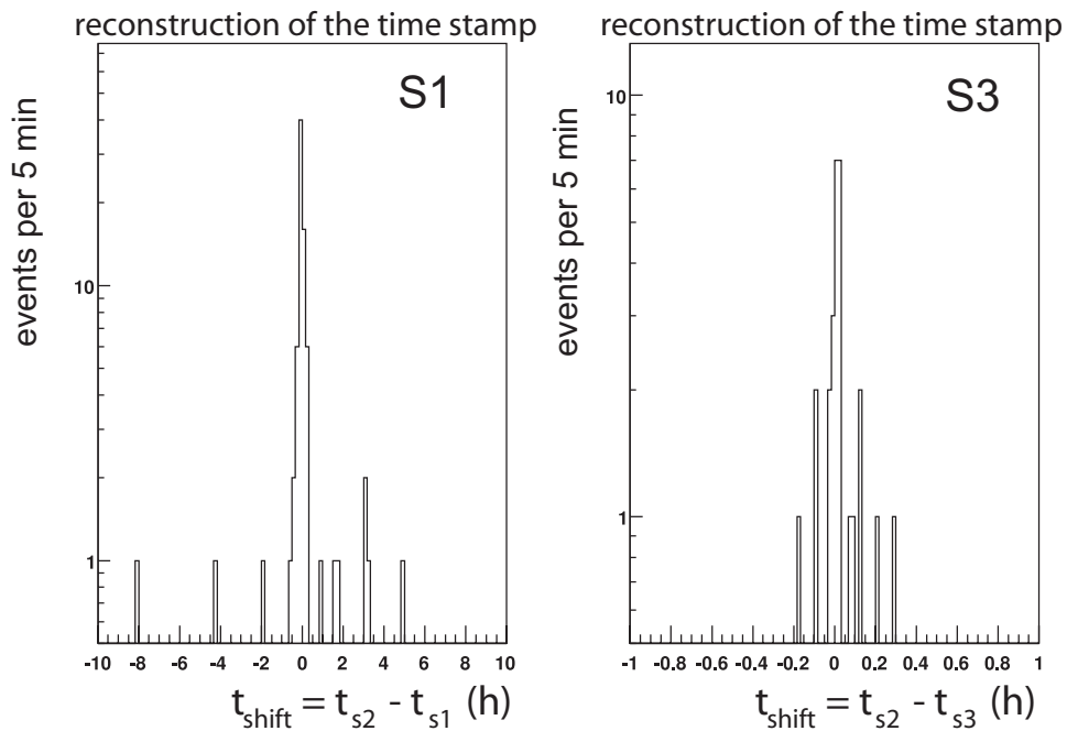
Figure 5.6: Shift applied to reconstruct the time stamp of s1 (left) and the time stamp of s3 (right) to correspond to this of s2 , shown in a 5 min binning. There is no systematic shift between the different clocks, and in the mean \Delta t_{\text{shift}} is \sim 1.5 min.
