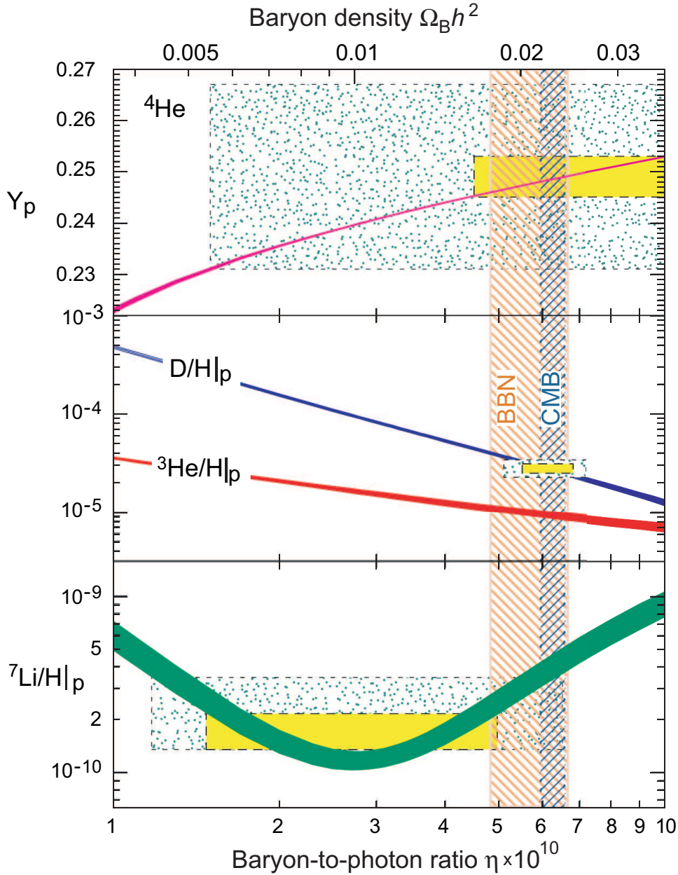
Figure 1.8: The abundances of ^4\text{He} , \text{D} , ^3\text{He} , and ^7\text{Li} as predicted by the standard model of big-bang nucleosynthesis – the bands show the 95% CL range. Boxes indicate the observed light element abundances (smaller boxes: \pm 2\sigma statistical errors; larger boxes: \pm 2\sigma statistical and systematic errors). The narrow vertical band indicates the CMB measure of the cosmic baryon density, while the wider band indicates the BBN concordance range (both at 95% CL). Figure from [25].
