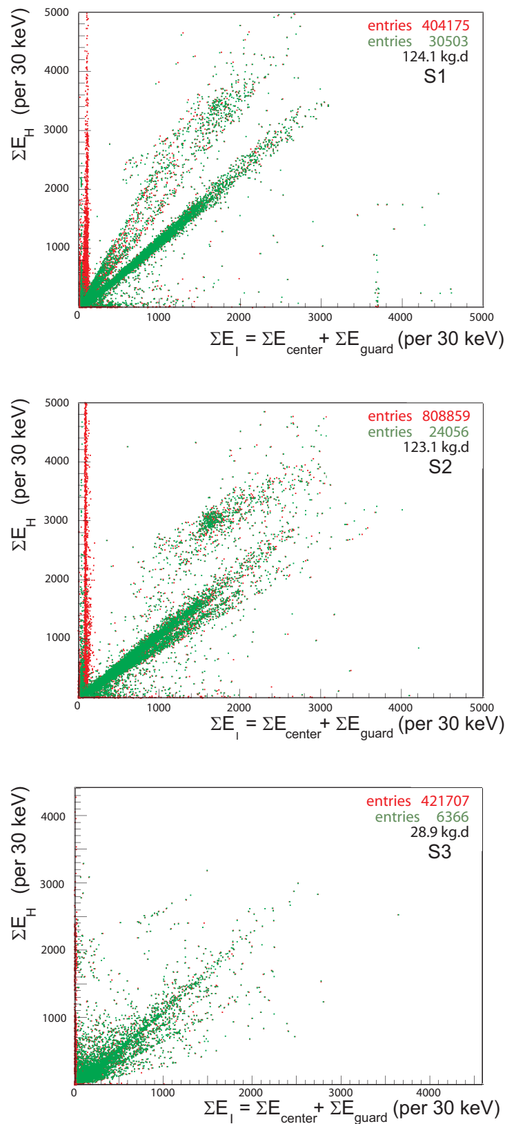
Figure 6.5: Biplot of the heat channel versus the sum of the ionization channels from guard and center from s1, s2 and s3 for energies below 5 MeV. Events in red survive the adaptative threshold, events in green have E_H > 30 keV and E_I > 30 keV.
