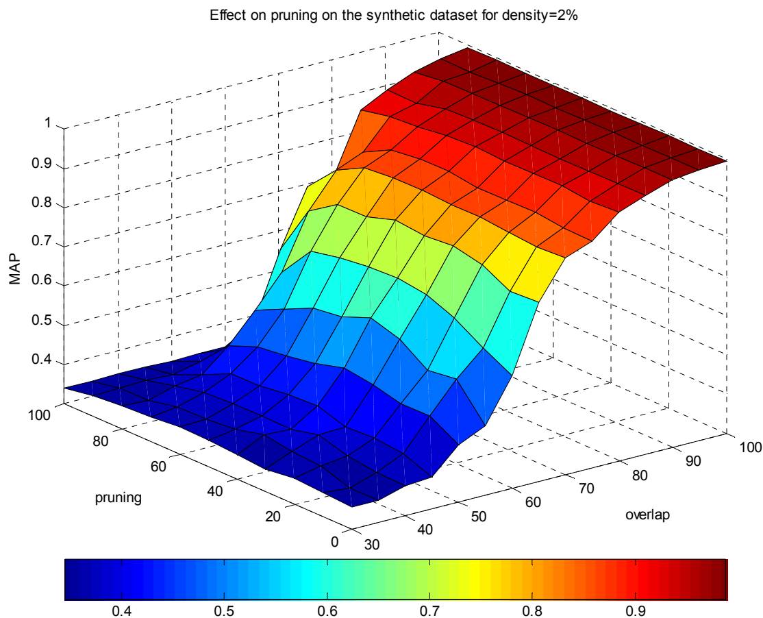
FIGURE 4.3 Effect of pruning on the synthetic dataset
