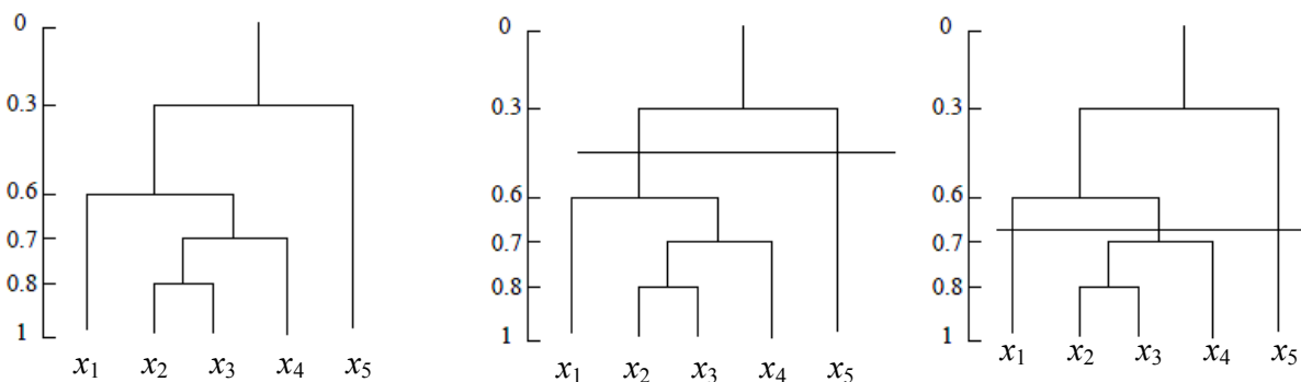
FIGURE 2.2 A dendrogram showing different clustering of 5 documents x_1..x_5
