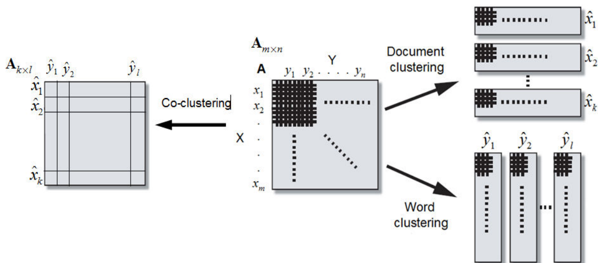
FIGURE 2.6 The Two-Way clustering and Co-clustering Frameworks
