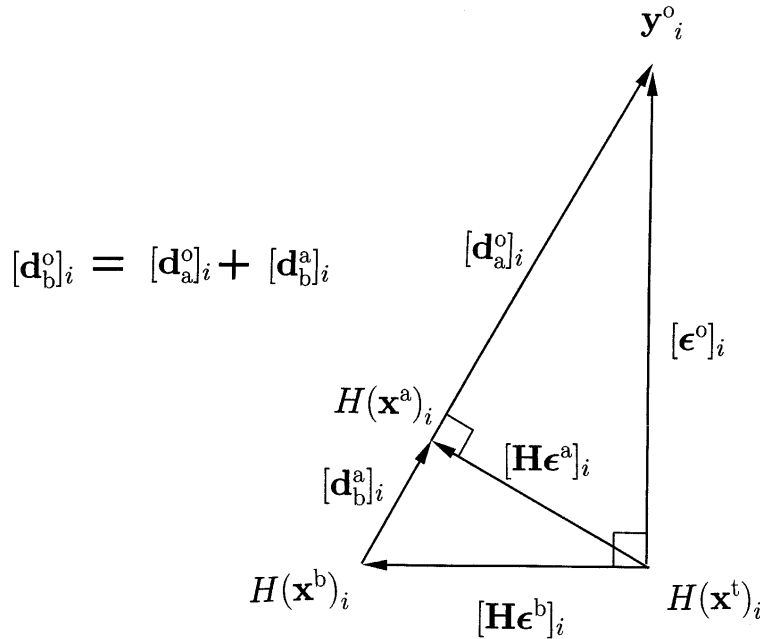
Figure 1. Geometrical representation of the analysis projected onto a particular eigenvector \mathbf{v}_i of matrix \mathbf{HK} .
