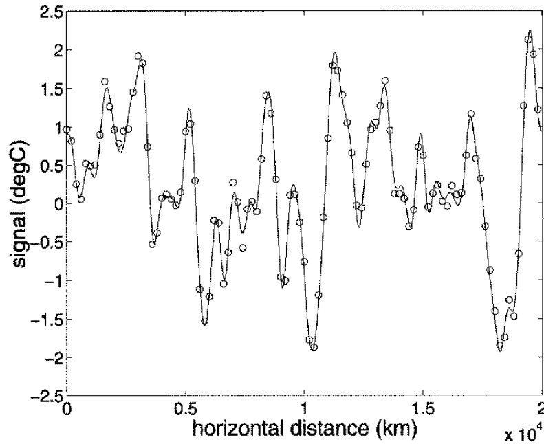
Figure 1. True signal x^t (full line) and observations y^o (circles) simulated with the procedure described in section 3(b); the length-scale of the structure function is 300 km and \lambda = s^{o2}/s^{b2} = 0.01 . See text for further details.
