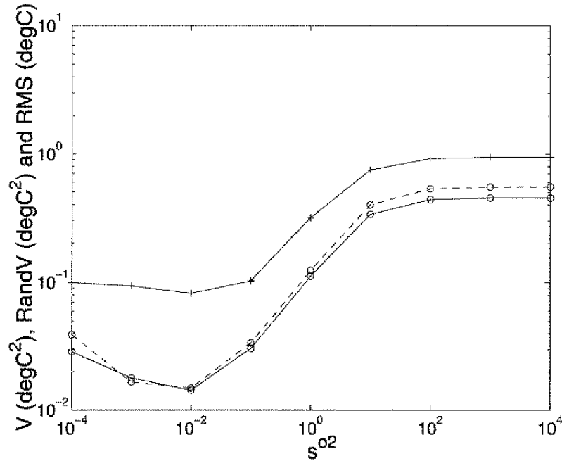
Figure 3. Exact Generalized Cross Validation criterion, V , as a function of s^{02} computed with the explicit solution (full line with circles) and randomized estimation \text{Rand} V of V (dashed line with circles) computed with the two solutions \mathbf{x}_{(y^0+\delta y^0)}^a and \mathbf{x}_{(y^0)}^a ; the root mean square error (r.m.s.) between \mathbf{x}^a(s^{02}) and \mathbf{x}^T is also plotted (solid line with crosses). See text for further details.
