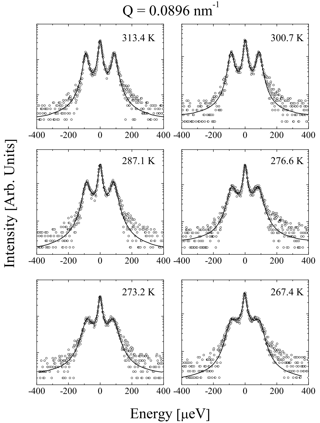
Figure 4.19: IUVS spectra at Q \approx 0.089 \text{ nm}^{-1} and temperatures indicated. The fitting lines are superimposed, evaluated according to the full spectrum lineshape of Eq. (4.4) in the generalized hydrodynamic regime which takes the structural relaxation into account.
