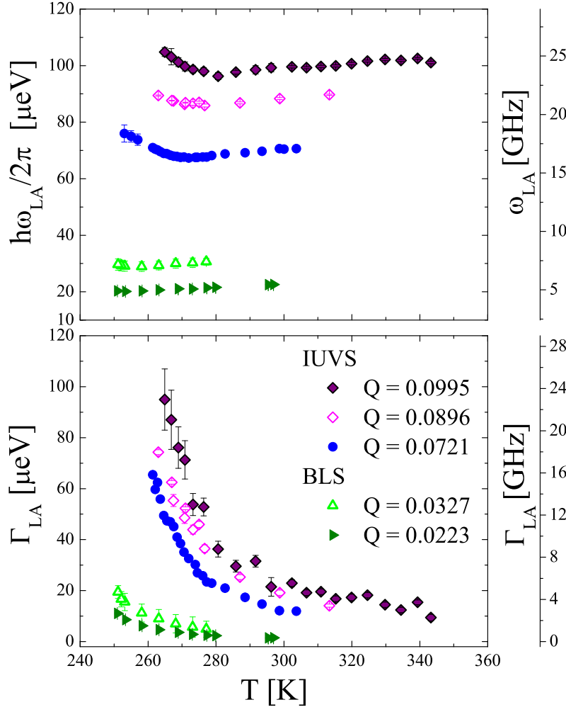
Figure 4.15: Fitting parameters \omega_{LA}(T) (upper panel) and \Gamma_{LA}(T) obtained from DHO analysis through Eq. (4.10). Each color corresponds to a series of experiment as specified in Table 4.4, which identify the Q -th longitudinal acoustic mode. Each point corresponds to a spectrum. Momentum transfer values are specified in figure's legend.
