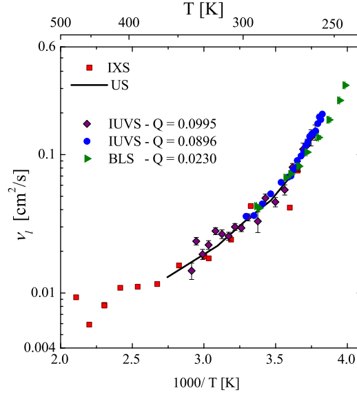
Figure 4.31: Angell plot of the longitudinal kinematic viscosity of water \eta/\rho , evaluated in this work by the DHO analysis.
