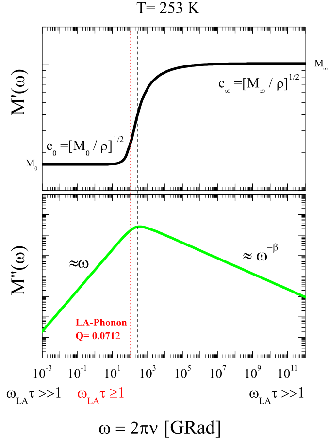
Figure 4.20: Frequency dependent (relaxing) longitudinal elastic modulus at T = 253, drawn from Eqs. (4.18) and (4.19) using the best-fit parameters of the full-spectrum analysis reported in Table 4.21. The relation between the parameters and the frequency regions of the relaxation is specified.
