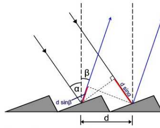
Figure 3.6: Blazed interference grating used in IUVS normal incidence monochromator and analyzer. The incoming radiation is reflected at a different "steps" of the blazed grating. Constructive interference is achieved when the condition m\lambda = d(\sin\alpha + \sin\beta) is fulfilled, with m integer number and \lambda the wavelength.
