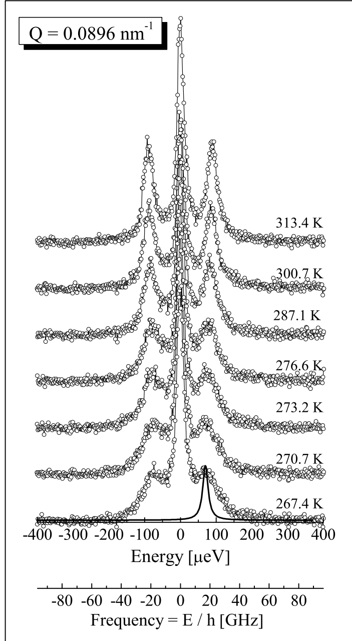
Figure 4.8: Series of IUVS spectra of water acquired at 6.2 eV incident energy and Q = 0.089 nm -1 . The temperature has been varied between 313 and 267 K. The resolution function is also shown as a bold continuous line.
