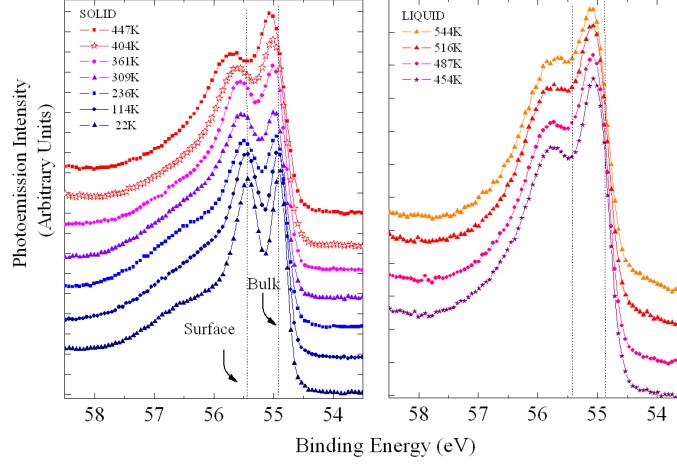
Figure B.2: Selection of the acquired XPS spectra of Li(110). Left panel: solid phase. Right panel: liquid phase. 22 K is the minimum temprature investigated, 544 K is the maximum temperature at which the liquid held. In both panels, the vertical dotted lines mark the position of bulk and surface peak at 22 K, as a reference for the binding energy temperature shift. A third contribution is present at high binding energies, due to lithium oxidation. It has been characterized and subtracted in data analysis.
