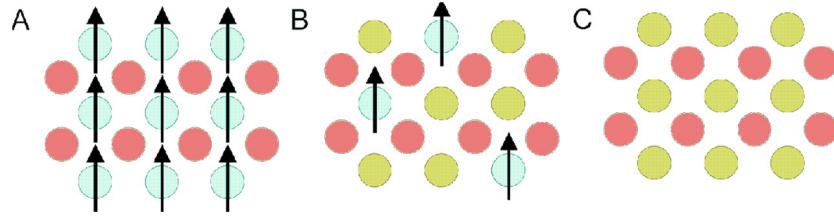
Figure 1.5: Three types of semiconductors: (A) a magnetic semiconductor, in which a periodic array of magnetic element is present; (B) a diluted magnetic semiconductor, an alloy between nonmagnetic semiconductor and magnetic semiconductor; and (C) a nonmagnetic semiconductor, which contains no magnetic ions[14].
