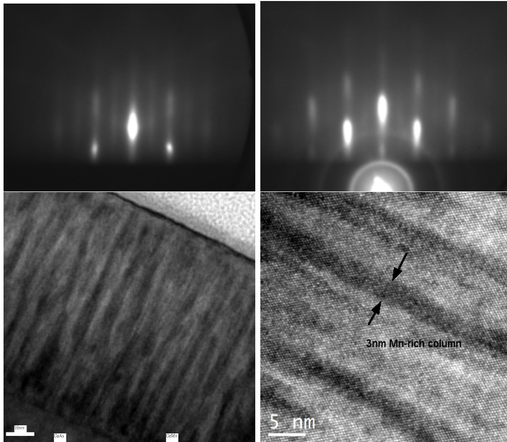
Figure 3.3: (a) (2\times 1) RHEED reconstruction shows flat GaAs surface, (b) RHEED pattern shows surface rougher after 80 nm (Ge,Mn) growth, (c) By cross-section TEM image of (Ge,Mn), Mn-rich nanocolumns are parallel, and (d) HRTEM image shows single crystal structure and around 3 nm columns.
