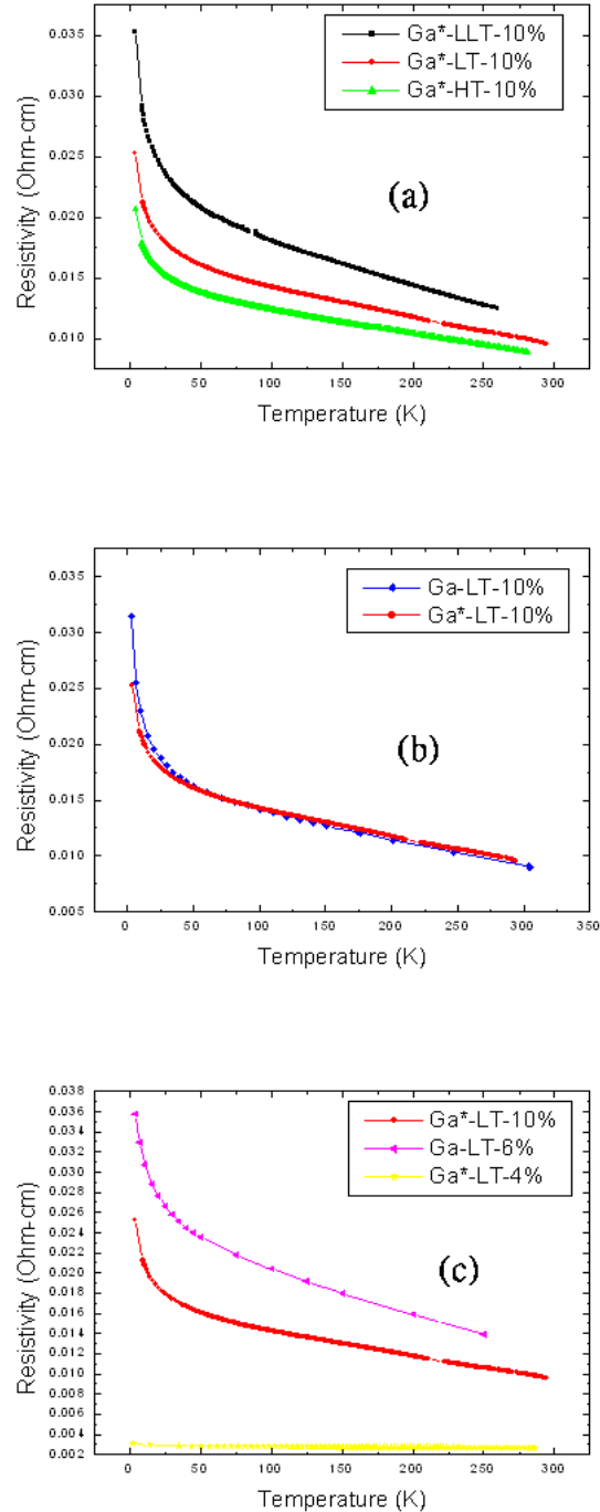
Figure 3.7: Temperature dependence of the zero-field resistivity for Ga-GeMn samples: (a) In 10% Mn samples, higher growth temperature makes (Ge,Mn) films lower resistivity (b) The curves are similar for samples with rough surface (Ga-LT-10%) and flat surface (Ga*-LT-10%), and (c) The samples with different Mn concentrations have different resistivity as a function of temperature.
