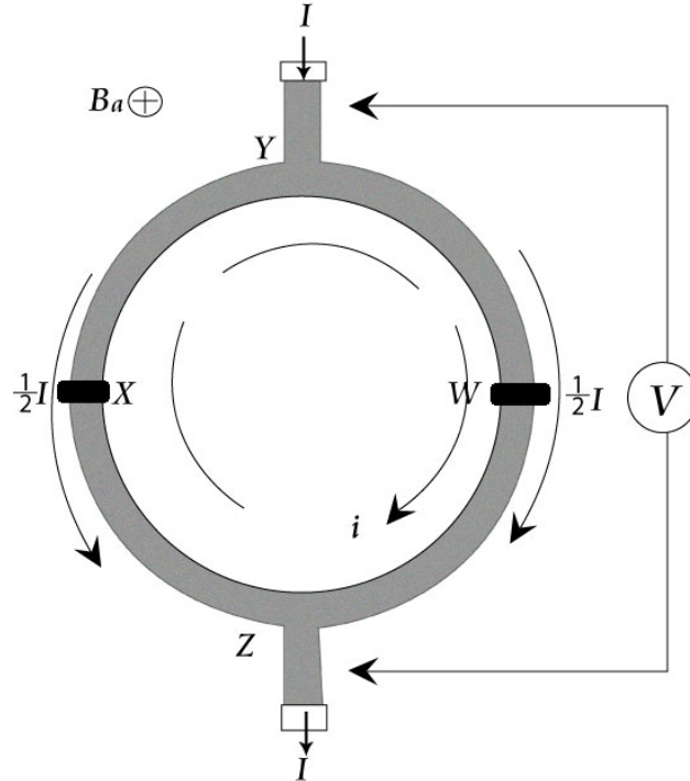
Figure 2.6: Superconducting quantum interference device as a single magnetometer.
