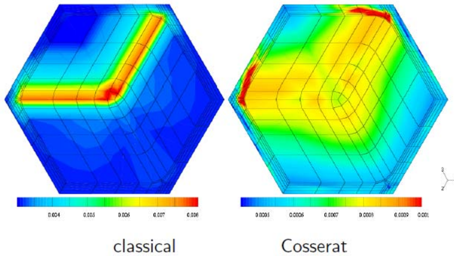
Figure I-3 Comparison of lattice rotations computed in classical continuum mechanics and using Cosserat modeling [For07].
