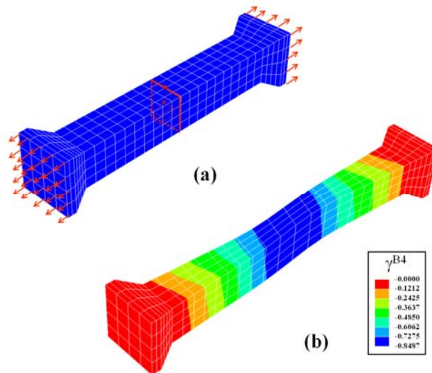
Figure II-1-13. (a) 512 element mesh and boundary conditions used for FEM tensile simulation along direction is <-1 2 5> (b) Deformed shape and resolved shear strain distribution on slip system B4 after up to 33% of global tensile deformation
