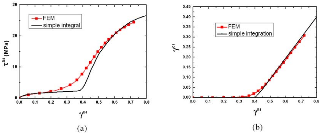
Figure II-1-14. Comparison between FEM calculation and simple integration (a) Resolved shear stress with resolved shear strain on slip system B4 during <-1 2 5> tensile test (b) Shear strain resolved on slip system C1 plotted versus the shear strain resolved on B4
