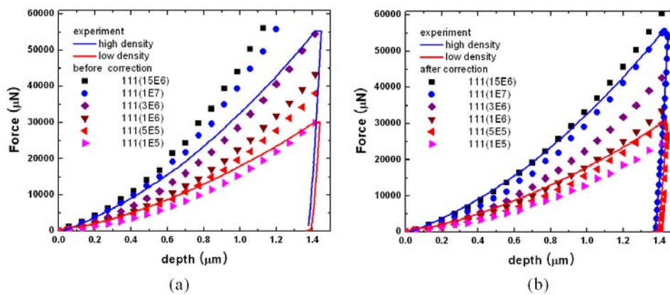
Figure III-4-3. Simulated applied load versus indenter displacement curves for indentation of (111) surface oriented samples with various initial dislocation densities (a) before correction of the simulation results, (b) after correction of the simulation results
