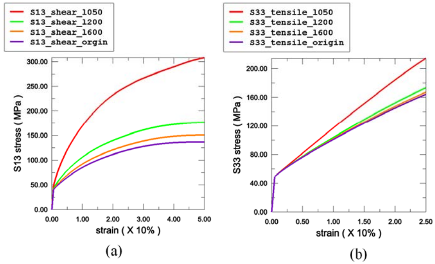
Figure II-2-11. Global loading curves plotted against the global strain (a) shear stress for difference element sizes (b) tensile stress for difference element sizes
