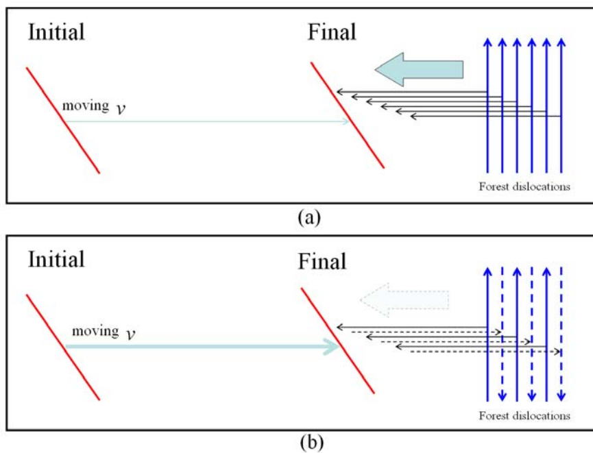
Figure II-2-3. Synopsis of dislocation movement beside two kinds of dislocation array (a) through array with high Nye tensor (b) through array with low Nye tensor
