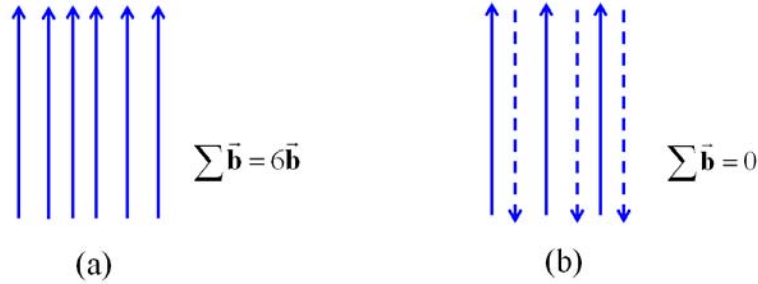
Figure II-2-1. Examples of dislocation arrays
