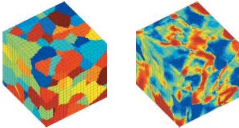
Figure I-2 Example of application of CPFEM in the case of Zinc polycrystal aggregates loaded in tension. Second figure shows plastic deformation on basal slip systems [FF04].
