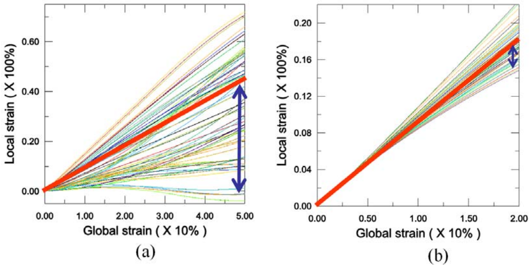
Figure II-2-12. Local strain in all the elements as function of the global strain (a) from shear loading condition (b) from tensile loading condition
