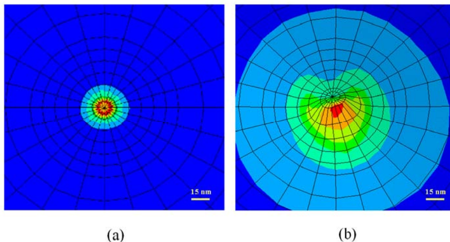
Figure III-3-3. Overview of diverging mesh effect due to the implicit method (a) initial mesh and initial stress results from nanoindentation of (111) surface orientation (b) deformed mesh obtained after deeper nanoindentation.
