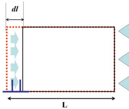
Figure II-2-9. The schematic diagram for extra compression forces and related variables
