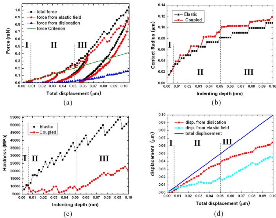
Figure III-6-14. DD simulation results .(a) force displacement curves, (b) contact radius vs. displacement, (c) hardness vs. displacement, (d) displacing fields
