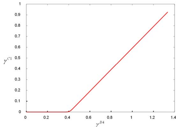
Figure II-1-9. Shear strain resolved on C1 slip system plotted versus the shear strain resolved on B4 slip system
