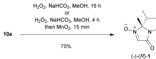
Scheme 5 Resolution of MiPNO: one-pot removal of resolving agent and oxidation.
