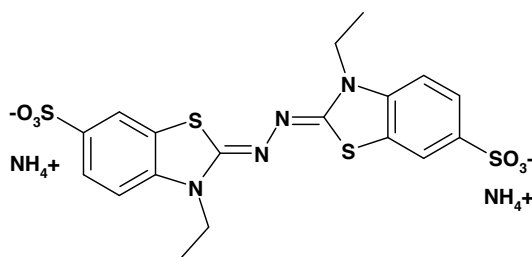
Figure 65 : ABTS
