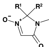
Figure 15 : N -oxy-imidazolidinones
