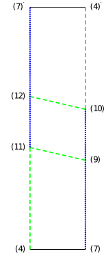
Figure 4.1: Fundamental domain in the case m = 19 .
