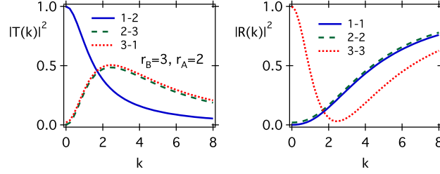
Fig. 9. Transmission and reflection probabilities for Y-junction with \text{rank}(B) = 3 , \text{rank}(A) = 2 . Parameter values s_{11} = s_{12} = s_{22} = s_{33} = 1 , s_{13} = s_{23} = 2 are used in (4.40).
