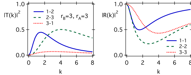
Fig. 10. Transmission and reflection probabilities for Y-junction with \text{rank}(B) = 3 , \text{rank}(A) = 3 , the generic condition. In the left side, solid line represents |\mathcal{T}_{12}(k)|^2 , dashed line |\mathcal{T}_{23}(k)|^2 , and dotted line |\mathcal{T}_{31}(k)|^2 . In the right, solid line represents |\mathcal{R}_1(k)|^2 , dashed line |\mathcal{R}_2(k)|^2 , and dotted line |\mathcal{R}_3(k)|^2 . Parameter values s_{11} = -1/3 , s_{12} = -1 , s_{13} = 1 , s_{22} = 1 , s_{23} = -3 , s_{33} = -4 are used in (4.40).
