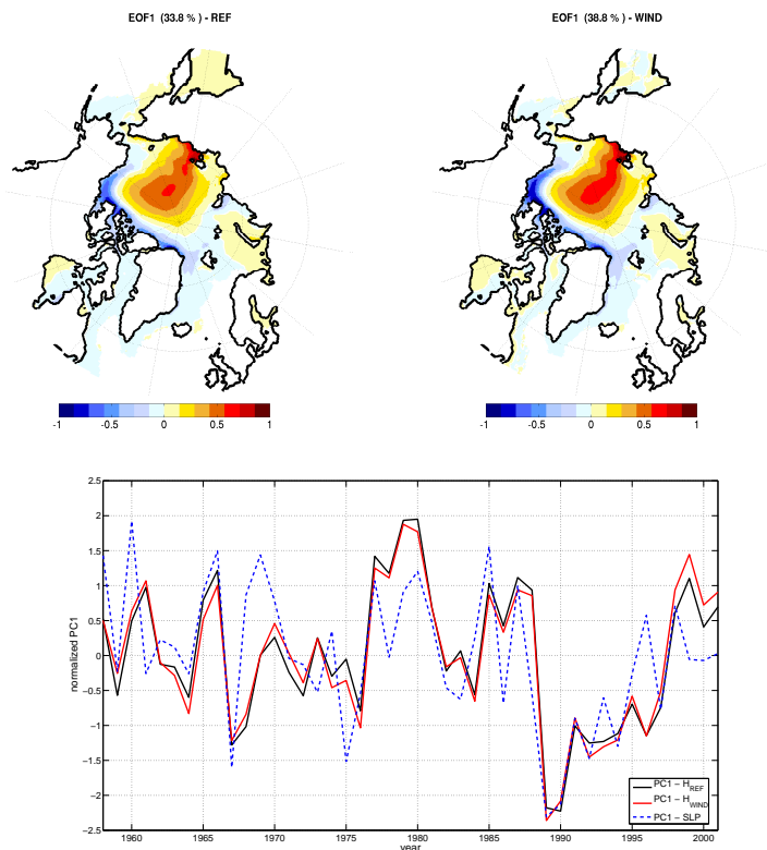
Fig. 5.8, along with the time series of its amplitude coefficient.
