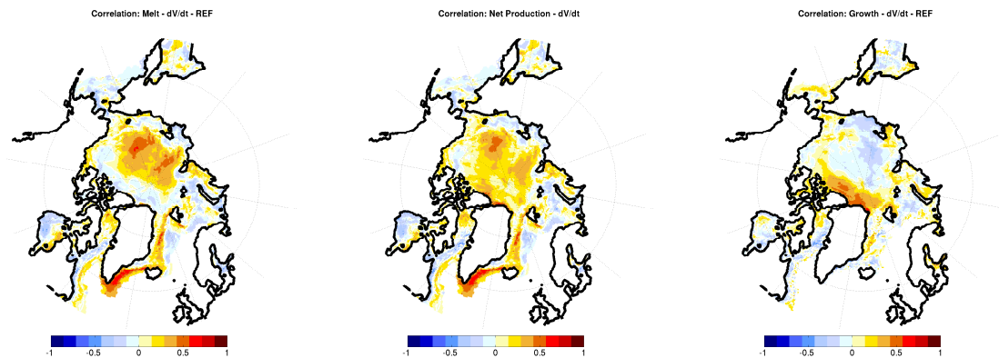
FIG. 5.11: Correlation between the sea ice volume derivative time series and the sea ice melt (left), net production (middle) and growth (right) for the REF simulation.
