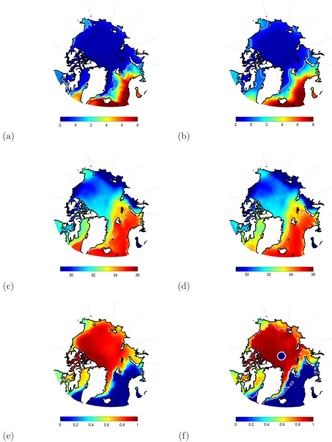
FIG. 4.10: Left : Mean model fields over the Arctic Ocean. (a) Sea Surface Temperature (in ^{\circ}C ). The 0^{\circ}C contour is superimposed in white. (c) Sea Surface Salinity (in psu). The 34 psu contour is superimposed in white. (e) Sea-ice concentration, with the September (dotted line) and March (plain line) extents superimposed with a dotted and a plain white line, respectively. Right : Same as Left, but for the PHC climatology ((b) and (d)) and Sea Ice observations averaged over 1992–2001 (Ezraty et al., February 2007).
