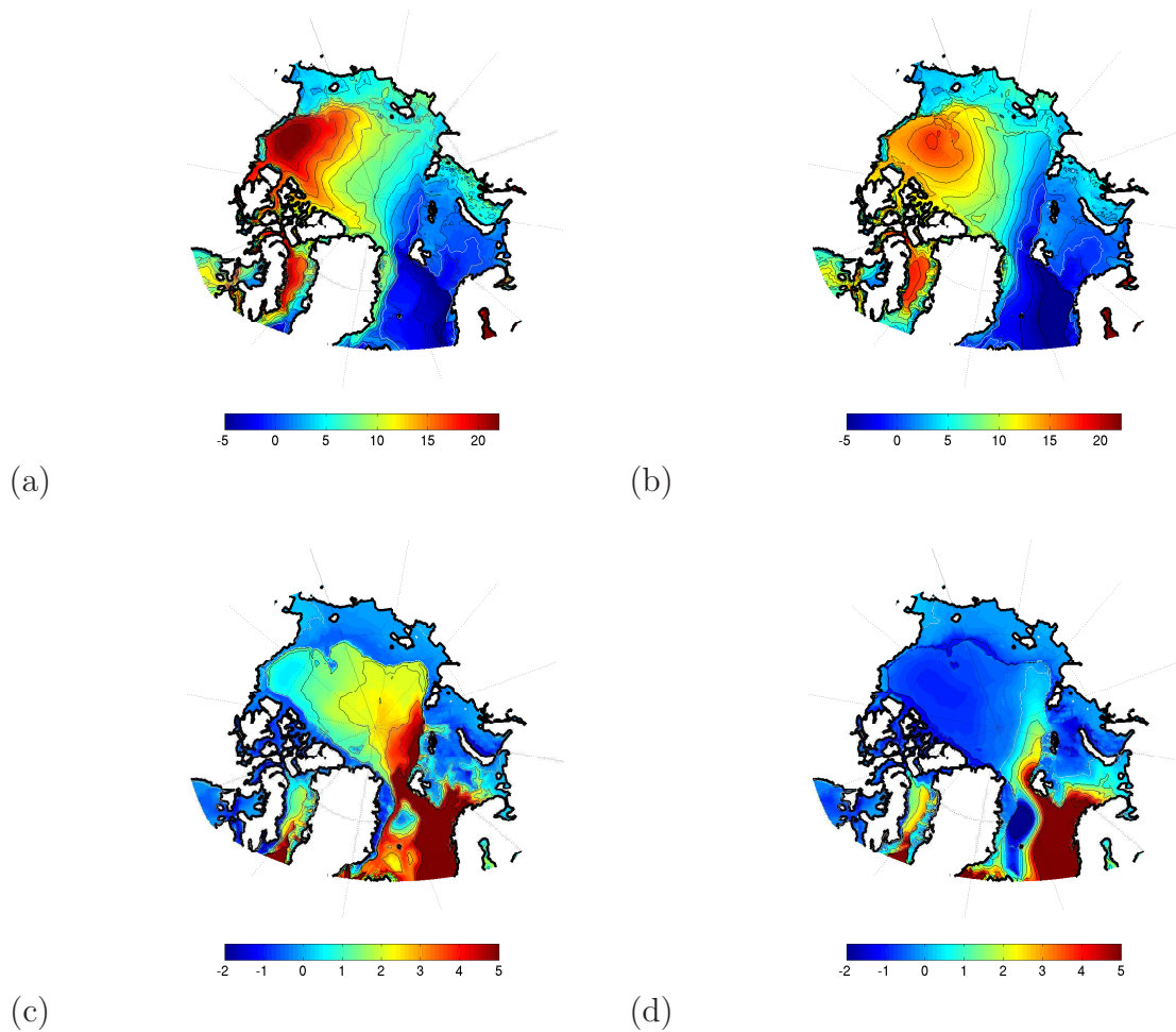
FIG. 4.3: Left : Model annual mean freshwater content ((a), in m.) and heat content ((c), in GJ.m^{-2} ) over the upper 1000 m. Right : Same as Left, but for the PHC climatology. The freshwater content and the heat content are referenced to 34.8 psu and 0^{\circ}C .
