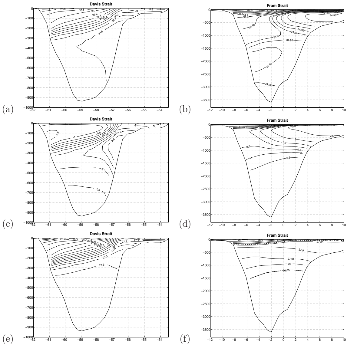
FIG. 4.4: Model vertical section of mean salinity (in psu) (a and b), mean temperature (in °C) (c and d) and mean density (referenced to the surface) (e and f) across Davis Strait (left) and Fram Strait (right). Isopycnal contours 27.8 and 28.05 are superimposed as dotted lines (f).
