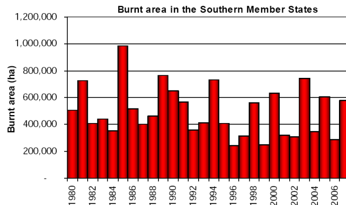
FIG. 5.14 – Burnt area climatology between 1980 and 2007 for 5 south Member States of European Union. After EFFIS (2008).
