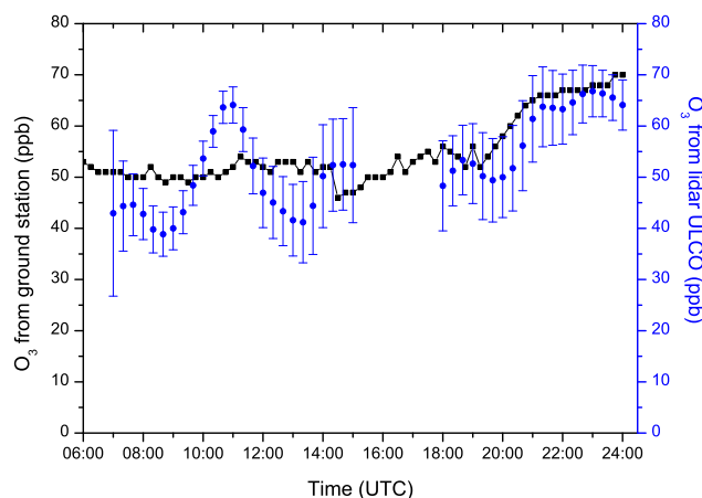
O3 measurements from lidar ULCO and ground station at PDM (03/07/2005)
