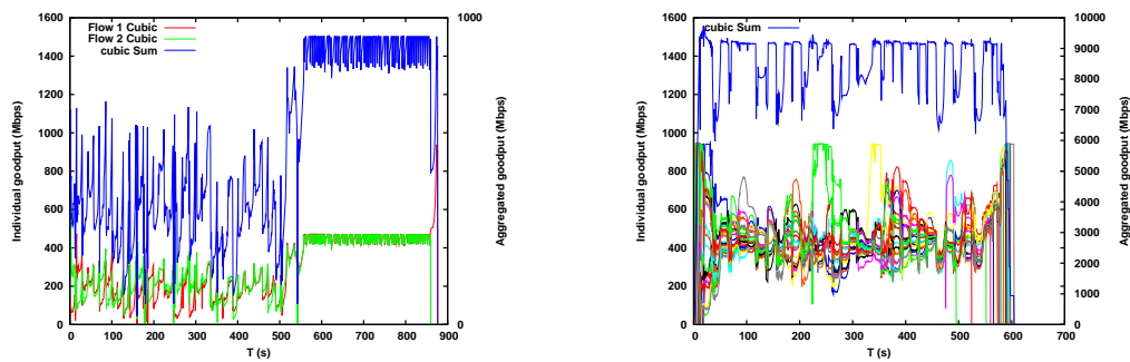
(a) 2x Cubic 1Gbps flows, 1Gbps bottleneck
