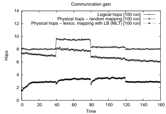
Figure 4.10: Reduction of the communication by the lexicographic mapping.
