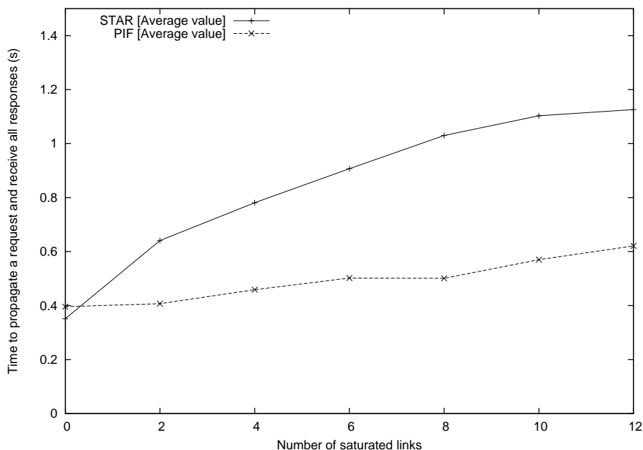
Figure 6.10: Experimenting the \text{PIF}_{async} and the \text{STAR}_{async} scheme on a network with overloaded links.
