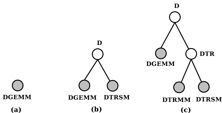
Figure 3.3: Construction of a proper greatest common prefix tree. Nodes storing some services' references (labeled by real keys) are grey-filled, the others are labeled by virtual keys. (a) First a DGEMM is declared. (b) A DTRSM is declared resulting in the creation of their parent, whose label is their greatest common prefix, i.e. , D. (c) Finally, a DTRMM is declared and the node DTR is created.
