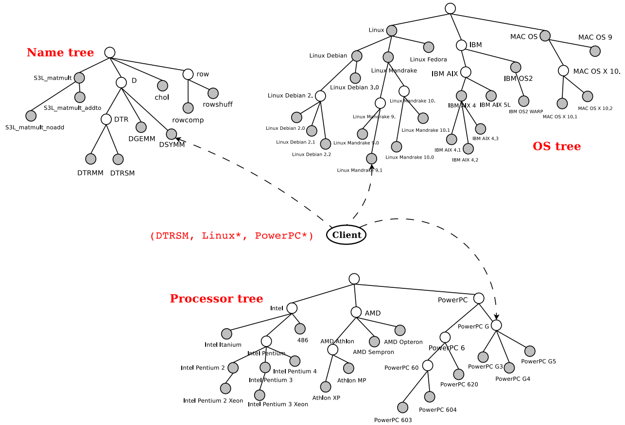
Figure 3.8: Processing a multi-attribute query.
