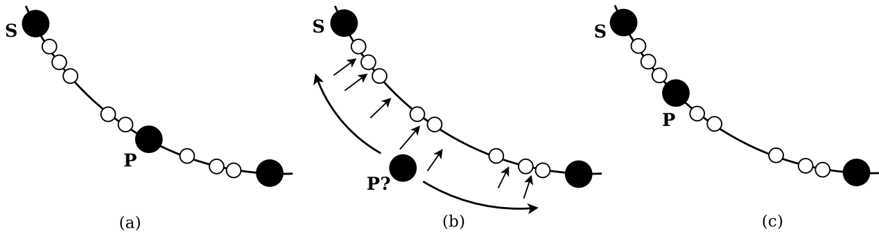
Figure 4.4: One local load balancing step.
