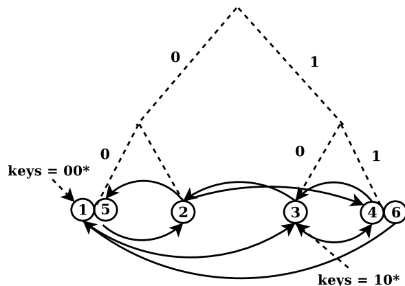
Figure 2.7: P-Grid.
