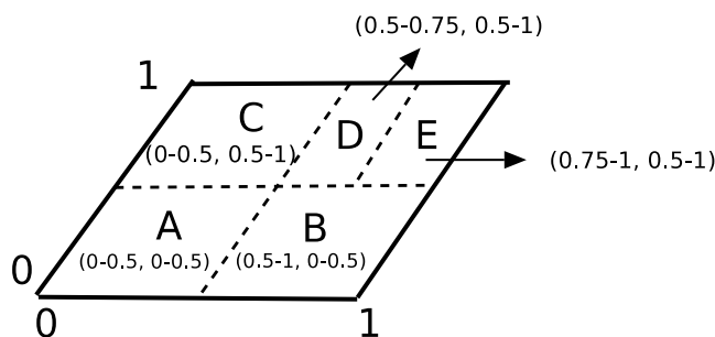
Figure 2.1: CAN, d = 2 .
