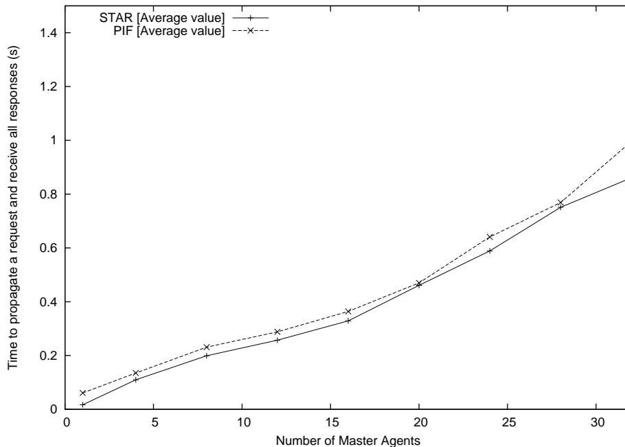
Figure 6.7: Evaluating the cost of using the \text{PIF}_{async} compared to the \text{STAR}_{async} on one cluster.
