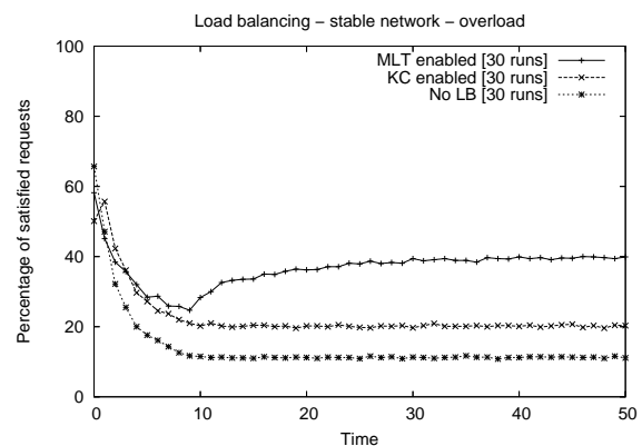
Figure 4.6: Stable network, high load.
