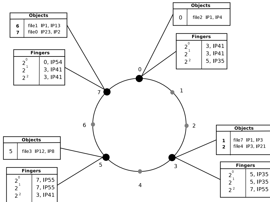
Figure 2.2: Chord, m = 3 .
