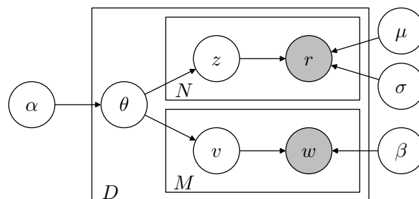
FIGURE 5.2 – Modèle GM-LDA
