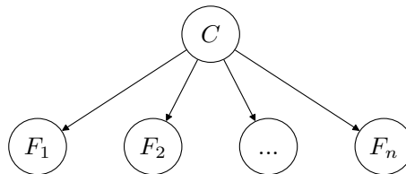
FIGURE 6.5 – Naïve Bayes
