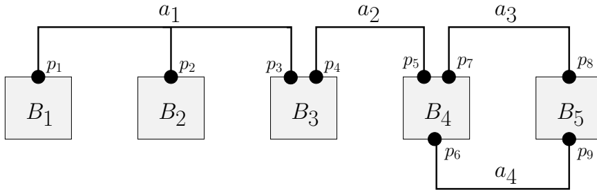
Figure 5.1: A simple high-level BIP model.
