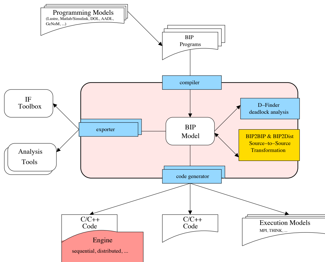
Figure 3.14: The BIP tool-chain.
