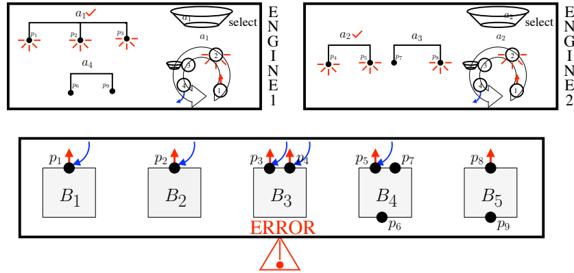
Figure 5.3: Violating of BIP semantics when badly distributed interactions.
