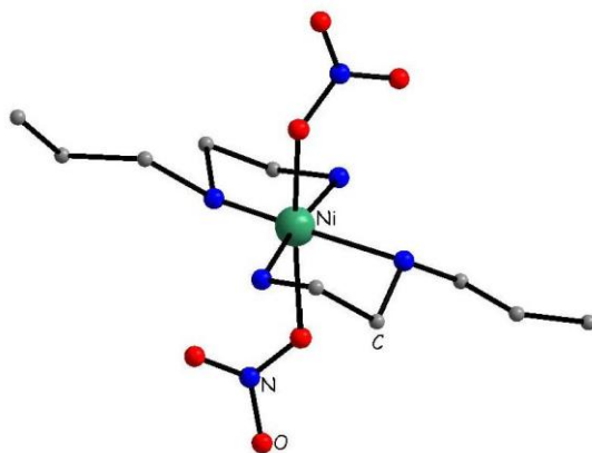
Figure 4.3 Model of the crystal structure of complex \text{Ni}(\text{Pren})_2(\text{NO}_3)_2 , complex 2 (grayer C atom, blue N atom, red O atom, yellow S atom, green Ni(II)).
