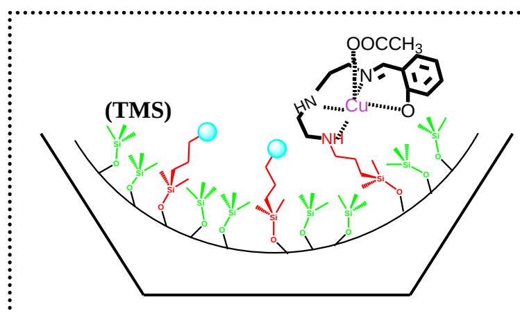
Scheme 5.8 Trimethylsilyl (TMS) and \text{Cu(II)} complex [\text{Cu(L}^3\text{)}(\text{CH}_3\text{COO})] functionalized LUS (MCM-41 type) via molecular stencil patterning method.
