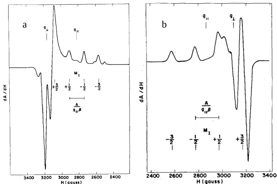
Figure 2.29 EPR spectra of (a) [\text{Cu}(\text{en})(\text{H}_2\text{O})_4]^{2+} at -150^\circ\text{C} in 60 % glycerine/40 % water with \text{en}/\text{Cu}(\text{II}) = 0.83 . The total \text{Cu}(\text{II}) concentration is 0.02M with roughly 68 % as [\text{Cu}(\text{en})(\text{H}_2\text{O})_4]^{2+} , 24 % as \text{Cu}(\text{H}_2\text{O})_6^{2+} , and 8 % as [\text{Cu}(\text{en})_2(\text{H}_2\text{O})_2]^{2+} ; (b) 0.02 M [\text{Cu}(\text{en})_2(\text{H}_2\text{O})_2]^{2+} at -150^\circ\text{C} in 60 % glycerine/40% water with \text{en}/\text{Cu}(\text{II}) = 2.25 . 124
