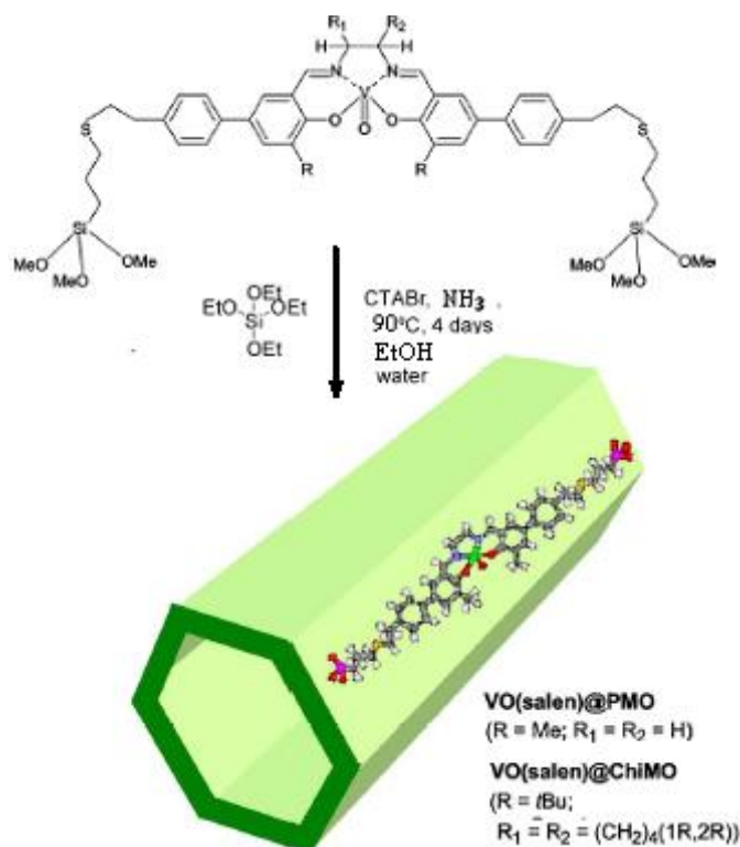
Figure 2.24 Preparation of VO(salen)@PMO and VO(salen)@ChiMO. Synthesis conditions: TEOS, \text{NH}_3 , CTAB, \text{H}_2\text{O} , EtOH, 90 °C, 4 days. 119
