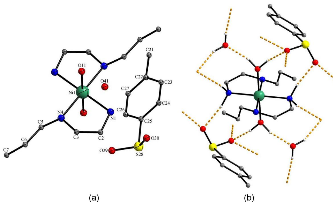
Figure 4.1 (a) Asymmetric unit of complex 1 , [\text{Ni}(\text{pren})_2(\text{H}_2\text{O})_2] \cdot 2\text{A} \cdot 2\text{H}_2\text{O} , ( \text{A} = \text{C}_7\text{H}_7\text{SO}_2 ), with atom labelling. Ellipsoids are represented with a probability of 30%. Hydrogen atoms have been removed for clarity; (b) hydrogen bonds present in the structure of complex 1 and hydrogen atoms are not involved in.
