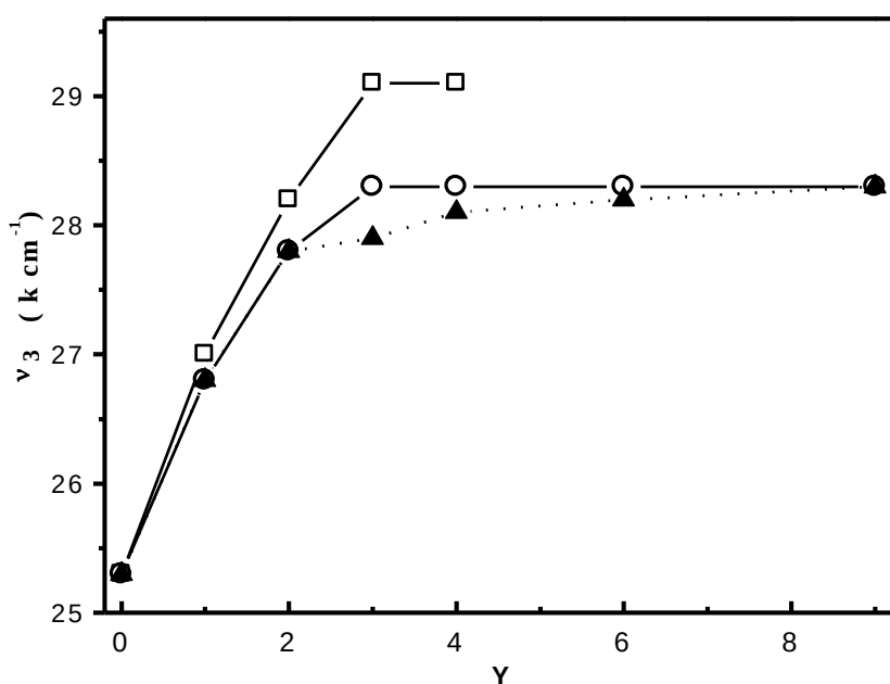
Figure 4.7 \nu_3 absorption bands vs. Y (Ligand/Ni) molar ratio. “□”, Ni-en complexes in water; “○”, Ni-Pren complexes in absolute ethanol; “▲”, Ni-Pren or Ni-L 1 complexes in water.
