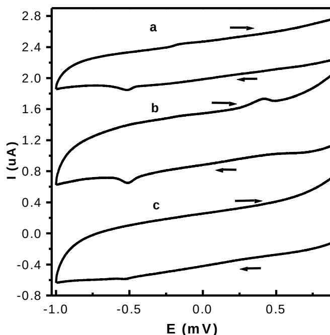
Figure 5.5 Cyclic voltammogram of \text{Cu}(\text{L}^1)_2 (a), \text{M-OP-Cu}(\text{3L}^1) (b), \text{M1'-ES-Cu}(\text{2L}^1) (c) at scan rate 0.4 \text{ V}\cdot\text{s}^{-1} .
