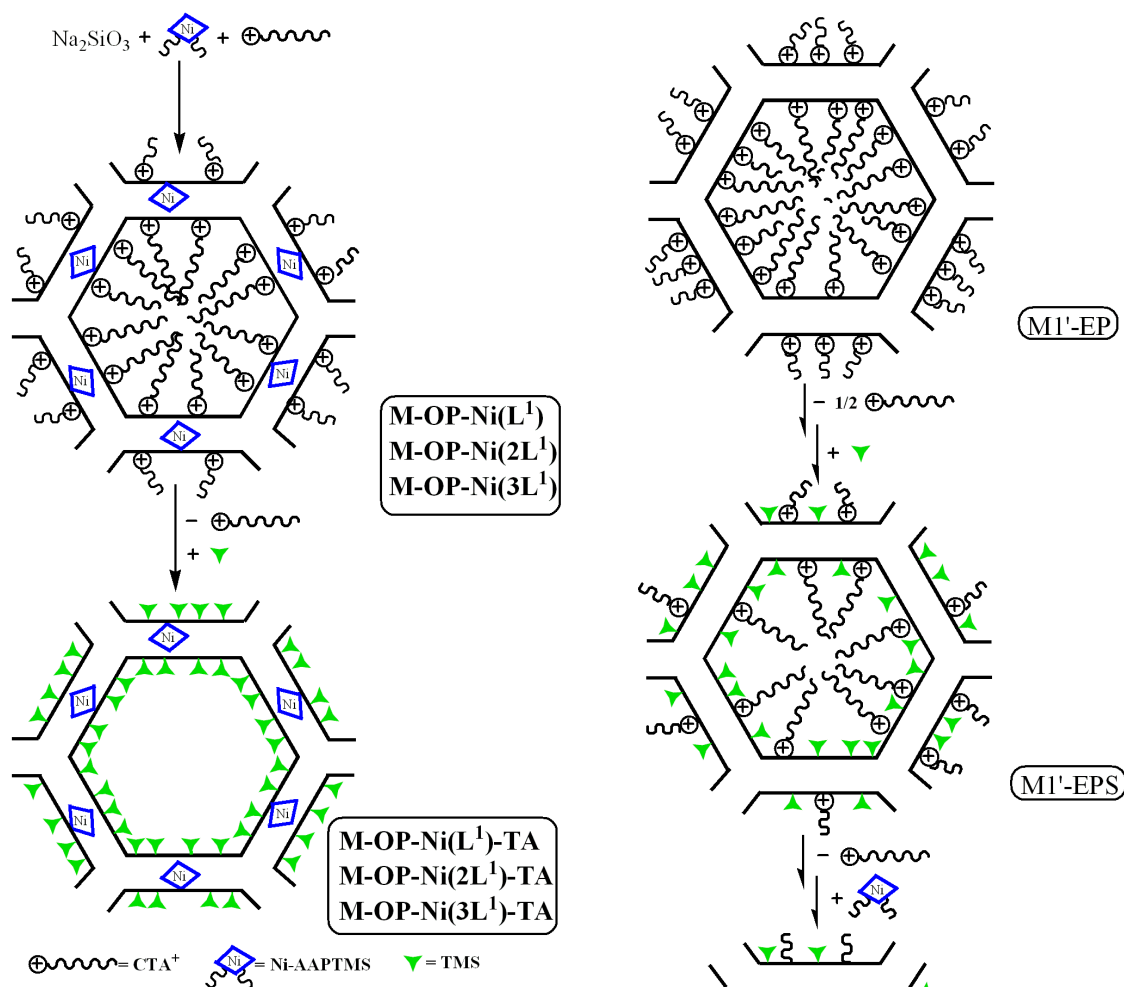
Scheme 4.3 Synthesis route of PMOs M-OP-Ni(YL 1 )-TA (Y= 1, 2, 3) (above).
