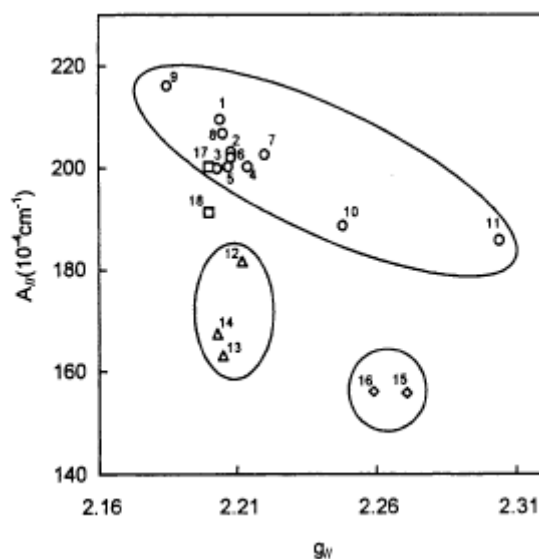
Figure 2.28 Relation between g_{||} -values and A_{||} -values for a \text{CuN}_4 complex. 123 ( \circ ) square-planar, ( \Delta ) axially-coordinate square-planar, ( \diamond ) tetrahedral, ( \square ) distorted square-planar. 1. (ethylenediamine) 2 ; 2. ( N -Methyl-ethylenediamine) 2 ; 3. ( N,N -dimethyl-ethylenediamine) 2 ; 4. ( N,N' -dimethyl-ethylenediamine) 2 ; 5. ( N -ethylene-ethylenediamine) 2 ; 6. ( N -Propyl-ethylenediamine) 2 ; 7. (1,3-trimethylenediamine) 2 ; 8. (trans-1,2-cyclohexanediamine) 2 ; 9. 1,4,8,11-tetraazacyclotetradecane; 10. ( \text{NH}_3 ) 4 ; 11. (pyridine) 4 ; 12. (diethylenetriamine) 2 ; 13. tetraethylenepentamine; 14. pentaethylenehexamine; 15. (1,10-phenanthroline) 2 ; 16. (2,2'-bipyridine) 2 ; 17. triethylenetetramine; 18. 1,4,7,10-tetraazacyclododecane.
