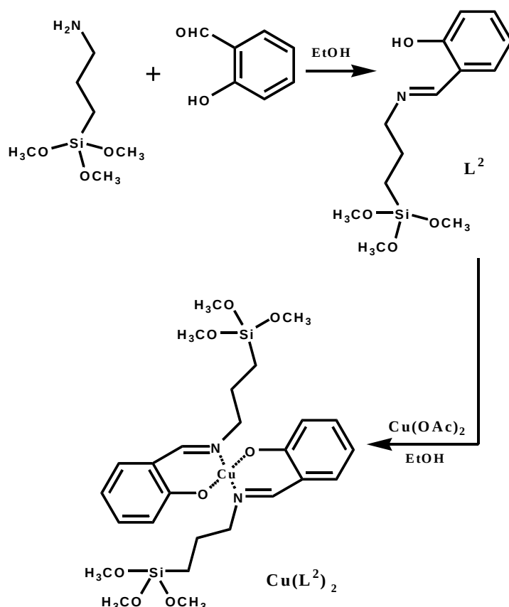
Scheme 5.4 Synthesis route for [Cu(L^2)_2] complex
