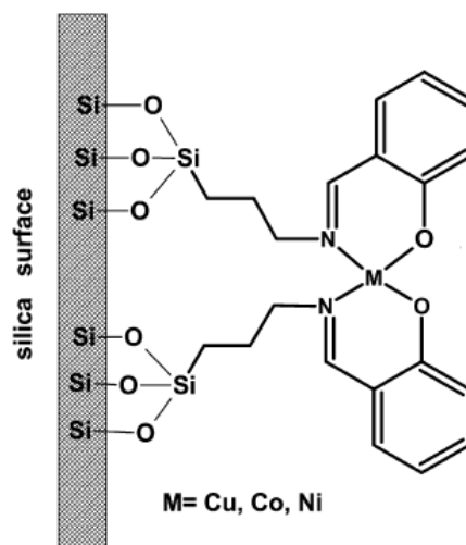
Figure 2.30 Synthetic route of the supported salicylaldimine complex [Cu(sal)]. 126
