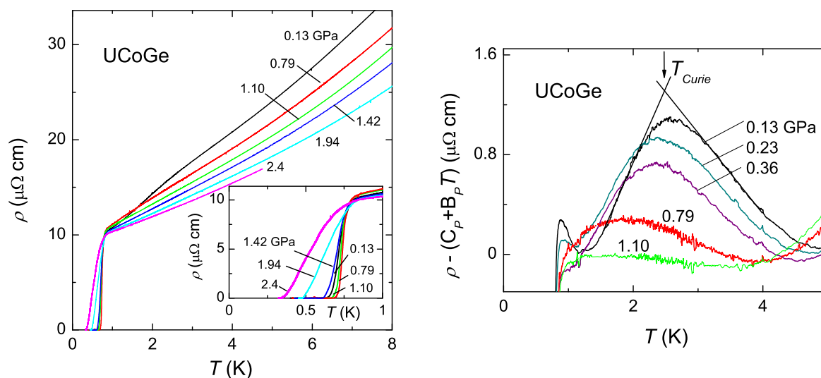
Fig. 4.5 : Left: Resistivity ( T, P ) of UCoGe for different pressures between 0.13 GPa and 2.4 GPa. The inset shows a zoom into the low temperature region with the superconducting transition, which is seen for all measured pressures. Right: Determination of the Curie temperature T_{Curie} in UCoGe: A straight line (resistivity linear in T ) has been subtracted from the resistivity data for each pressure to see clearly the transition temperature which has been determined by the crossing point of the two tangents here presented for P = 0.13 GPa.
