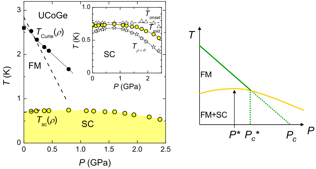
Fig. 4.6 : Left: Phase diagram ( T, P ) of UCoGe from resistivity measurements with the ferromagnetic (FM) phase and the superconducting (SC) phase. The dashed lines indicate the slopes of the transition lines calculated from Ehrenfest relation at ambient pressure (Huy et al. 2007). In the insert the onset-, midpoint- and zero-resistivity temperatures of the superconducting transition are shown. Lines are guides to the eye. Right: Schematic presentation of the phase diagram to visualize the definitions of the characteristic pressures appearing in the text.
