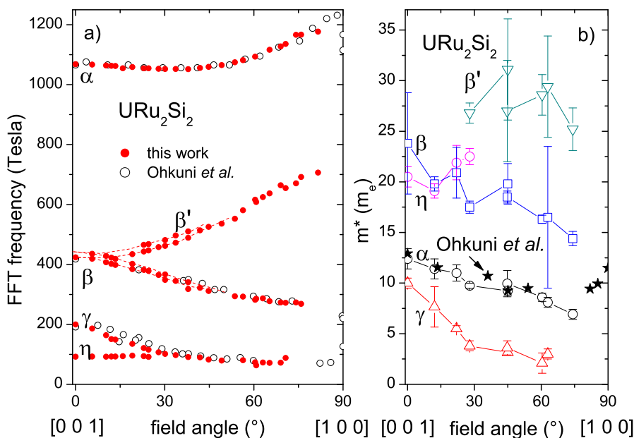
Fig. 3.32 : a) Angular dependence of the FFT frequencies obtained from SdH measurements in URu 2 Si 2 . The field range is 5-8 T as long as H_{c2} is low enough, then adapted to the available field range. b) Angular dependence of the effective masses. Earlier results by Ohkuni et al. (Ohkuni et al. 1999) are also plotted and are in excellent agreement.
