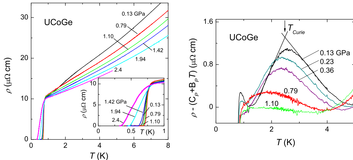
Fig. 4.5 : Left: Resistivity (T, P) of UCoGe for different pressures between 0.13 GPa and 2.4 GPa. The inset shows a zoom into the low temperature region with the superconducting transition, which is seen for all measured pressures. Right: Determination of the Curie temperature T_{Curie} in UCoGe: A straight line (resistivity linear in T ) has been subtracted from the resistivity data for each pressure to see clearly the transition temperature which has been determined by the crossing point of the two tangents here presented for P = 0.13 GPa.
