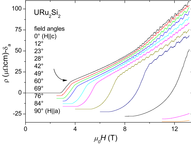
Fig. 3.25 : The magnetoresistance of URu 2 Si 2 for different angles for a field in the c - a plane.
