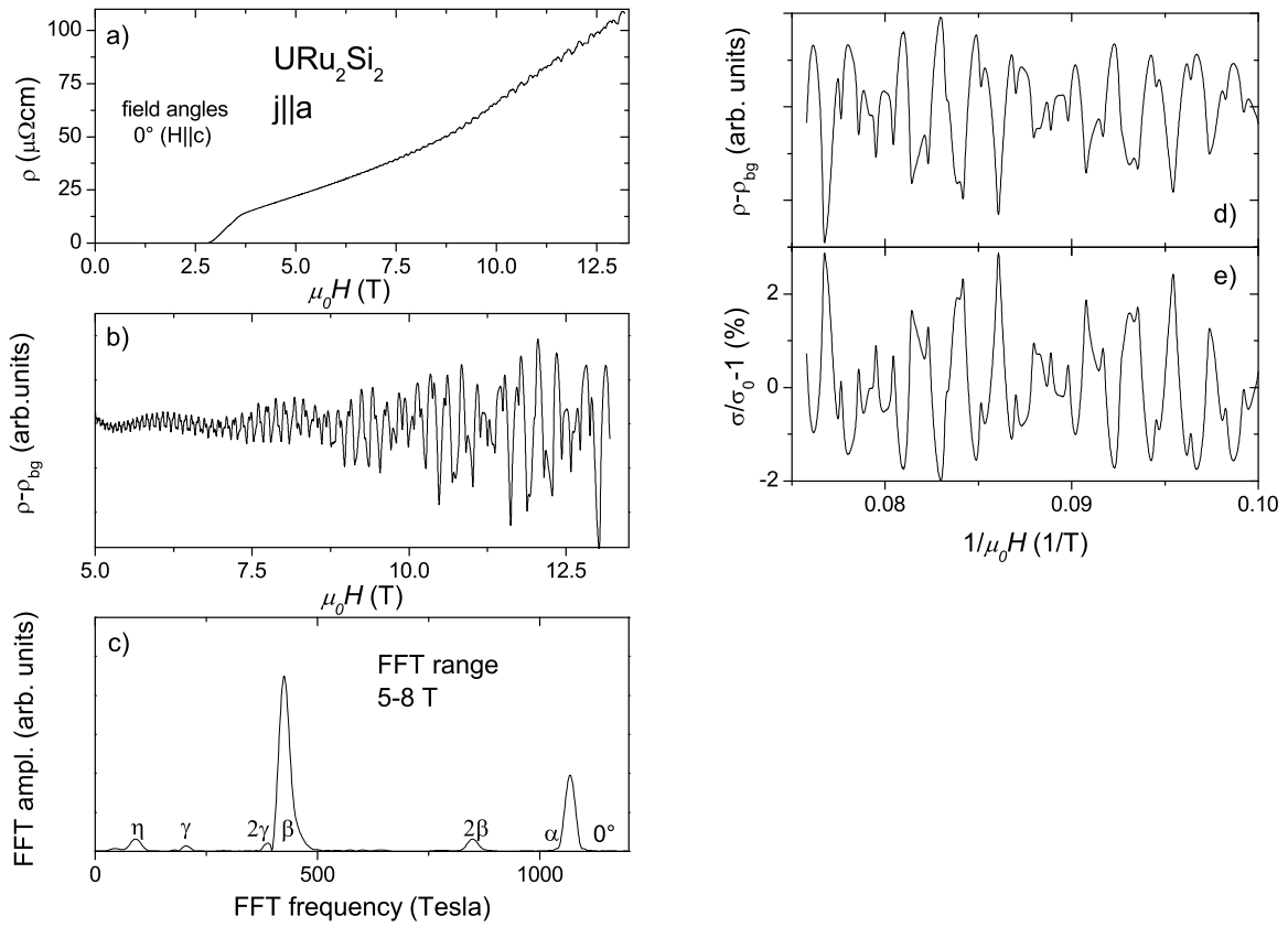
Fig. 2.9 : a) Magnetoresistance of URu 2 Si 2 at the lowest temperature T = 25 mK. b) Oscillatory part of the resistance as a function of field. c) FFT amplitude of this oscillatory part between 5 T and 8 T. d) Oscillatory part of the resistance as a function of the inverse field. e) Relative oscillatory part of the conductivity as a function of the inverse field.
