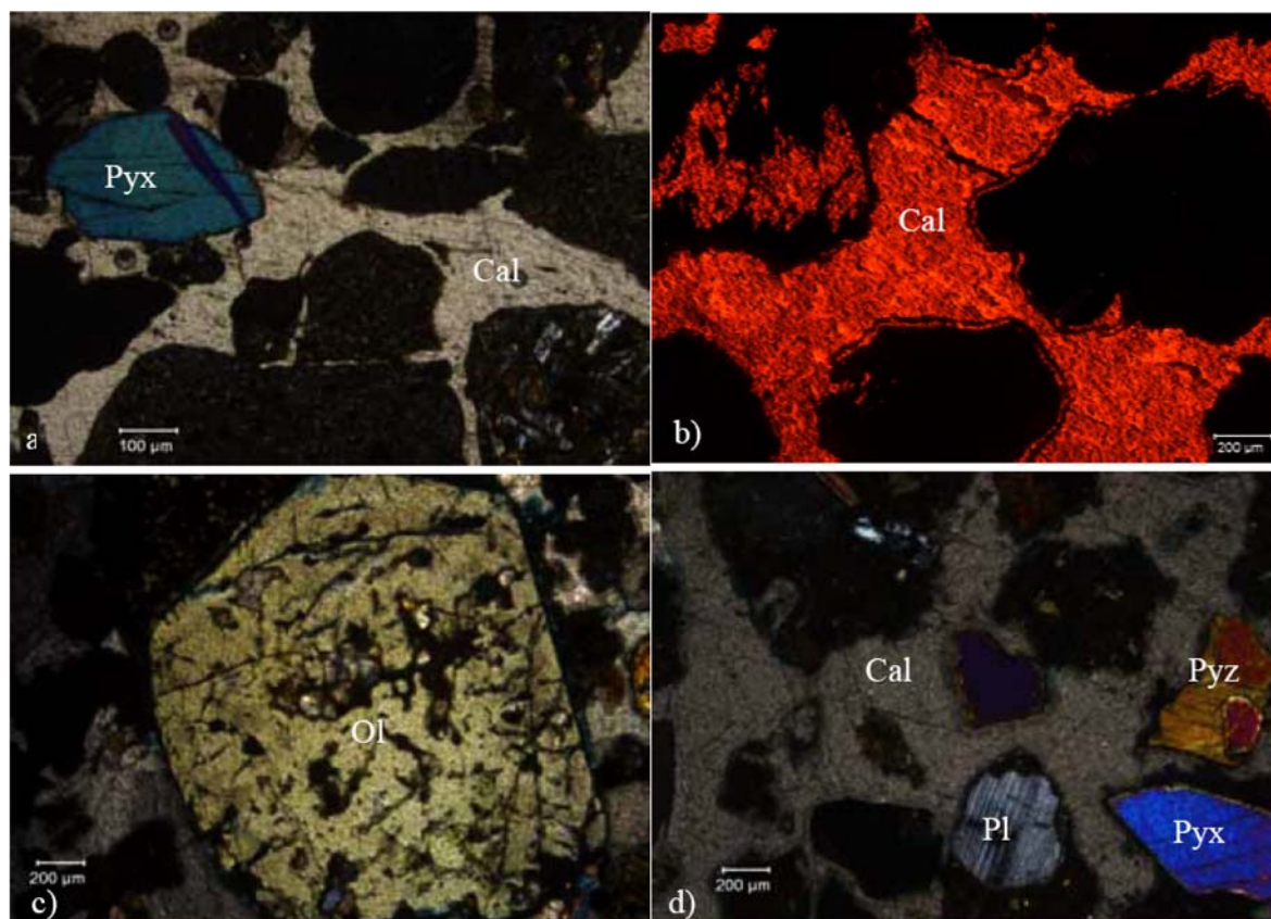
Figure 38. Petrographic characteristics of the Lothidok Sandstones. The main features include volcanoclastic detrital grains, cementation by calcite and the almost total absence of porosity. (a) detrital grains include volcanic grains, sedimentary rock fragments (srf), amphiboles and pyroxenes (Pyx). Cementation by calcite (cal) is pervasive, with poikilotopic textures. (b) Under cathodoluminescence, three zones of calcite are observed. The earliest is a very thin zone of brightly luminescent calcite, succeeded by a dark non-luminescent zone which is followed by a later brightly luminescent zone filling the pore spaces. (c) Olivine mineral (Ol) is a common detrital constituent of the Lothidok sandstones. (d) Plagioclase (Pyx), relatively unaltered is also common in the sandstones but in small percentages.
