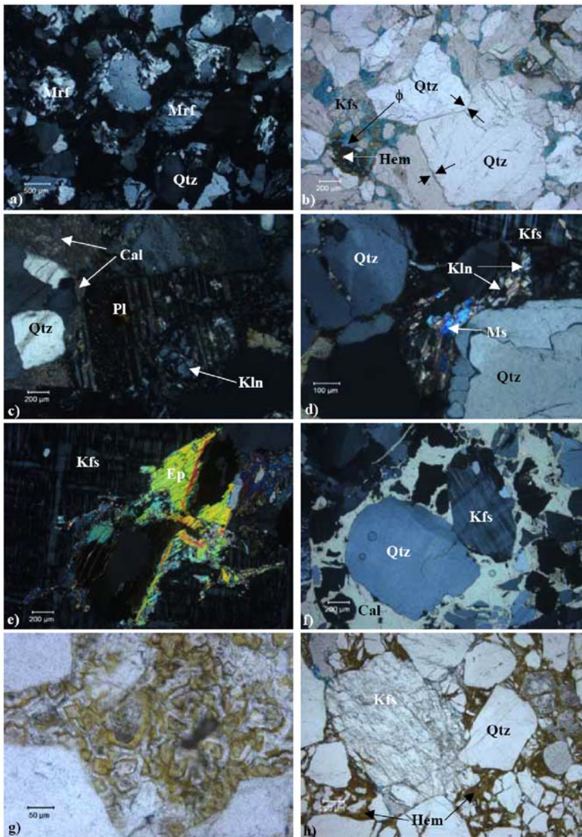
Figure 39. (a) Grains of metamorphic origin as well as metamorphic rock fragments ( mrff ) are an important detrital grains component within the Mt. Porr Formation. Polycrystalline quartz ( Qtz ) grains are also very common (LPA photo). (b) Hematite ( Hem ) is an early generation cement, mechanical compaction has resulted in dissolution of grains at their contacts. Substantial amounts of residual primary intergranular porosity ( \bar{E} ) has been preserved within the sandstones (LPNA photo). (c) Plagioclase feldspar ( pl ) dissolution is accompanied by precipitation of kaolin ( Kln ) (LPA photo). (d) Bent, broken and partially kaolinized muscovite grains ( Ms ) are good evidence for sediment mechanical compaction and chemical diagenetic alteration (LPA photo). (e) Intergrowths of feldspars and epidote ( Ep ) are common phenomena within the sandstones (LPA photo). (f) Early calcite ( Cal ) cementation was predated by some mechanical compaction of sediment, resulting in the dissolution of quartz and feldspar grains at contacts (LPA photo). (g) Pseudomorphs of dolomite have retained distinctive euhedral rhombic textures and zoning (LPNA photo). (h) Hematitic cements are post-compaction and they also postdate grain-to-grain pressure solution (LPNA photo). (LPA = polarized analysed light; LPNA= non polarized analysed light).
