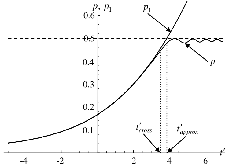
Fig. 2.4. Numerical graph of the molecular state probability p and adiabatic approximation (2.26) p_1 versus time t' for \lambda = 30 [where t' = \sqrt{\delta_0}t with t being time used in the initial set of equations (1.2)]. Two vertical lines mark the points where the exact phase trajectory and the adiabatic approximation cross the separatrix, t'_{cross} \approx 3.535 and t'_{approx} = \sqrt{\lambda/2} \approx 3.873 , respectively.
