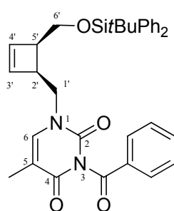
(+)-II.86
