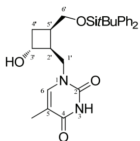
(-)-II.51a
