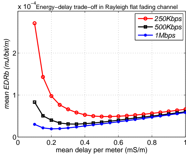
Figure 7.9: Effect of transmit rate on energy-delay tradeoff
