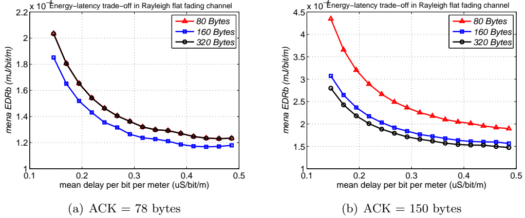
Figure 6.12: Effect of N_b on energy-delay trade-off in Rayleigh flat fading channels
