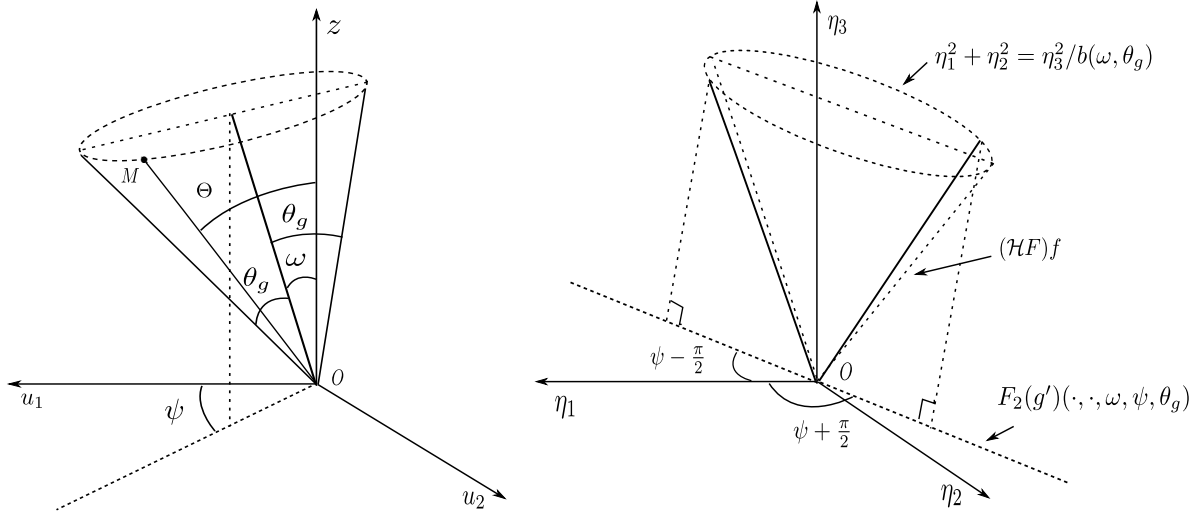
(a) Spatial domain. Cone \mathcal{C}(0, 0, \omega, \psi, \theta_g) .
