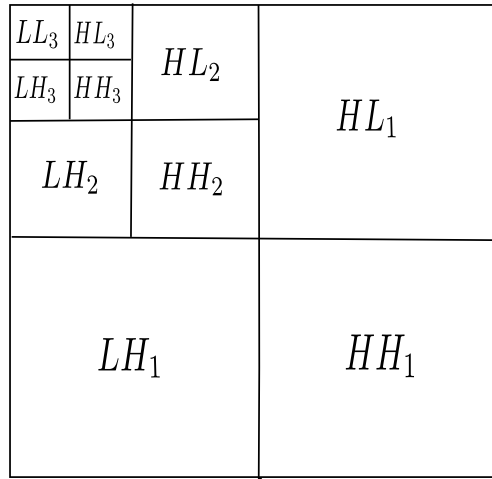
Figure 5.5: Schematic representation of the structure generated by applying a 2D-DWT with three decomposition levels of an input image. The coefficients d_{l,1} \in HL_1 , d_{l,2} \in LH_l , d_{l,3} \in HH_l , l = \overline{1, 3} represent the image details, while a_3 \in LL_3 represents the approximation coefficients of the low resolution image.
