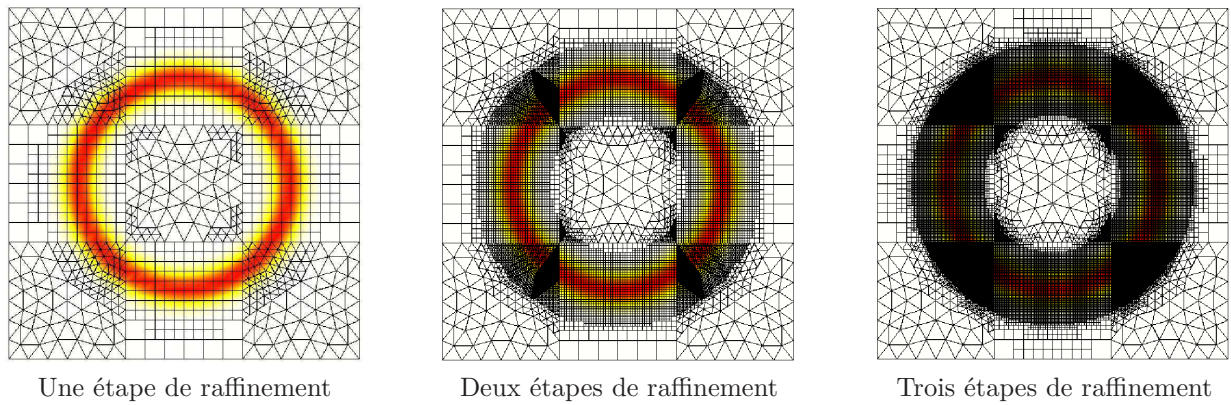
FIG. II.15 – Tri/Quadr-angles- P_1/Q_1 . Maillages raffinés.
