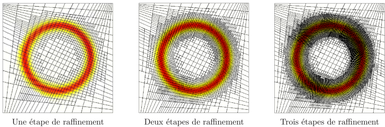
FIG. II.16 – Quadrangles- Q_1 . Maillages raffinés.
