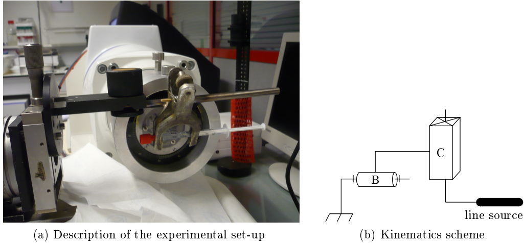
Figure 3.54 – Experimental set-up
