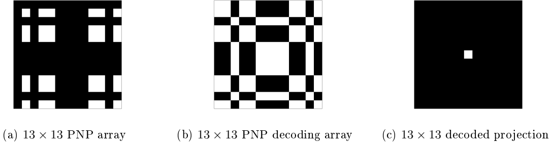
Figure 1.20 – PNP array
