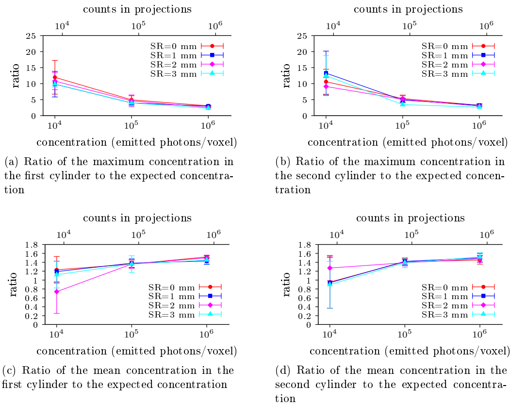
Figure 3.48 – Quantification ability of the imaging system with the accelerated MLEM-algorithm, the intrinsic spatial resolution (SR) of the detector being varied from 0 mm to 3 mm
