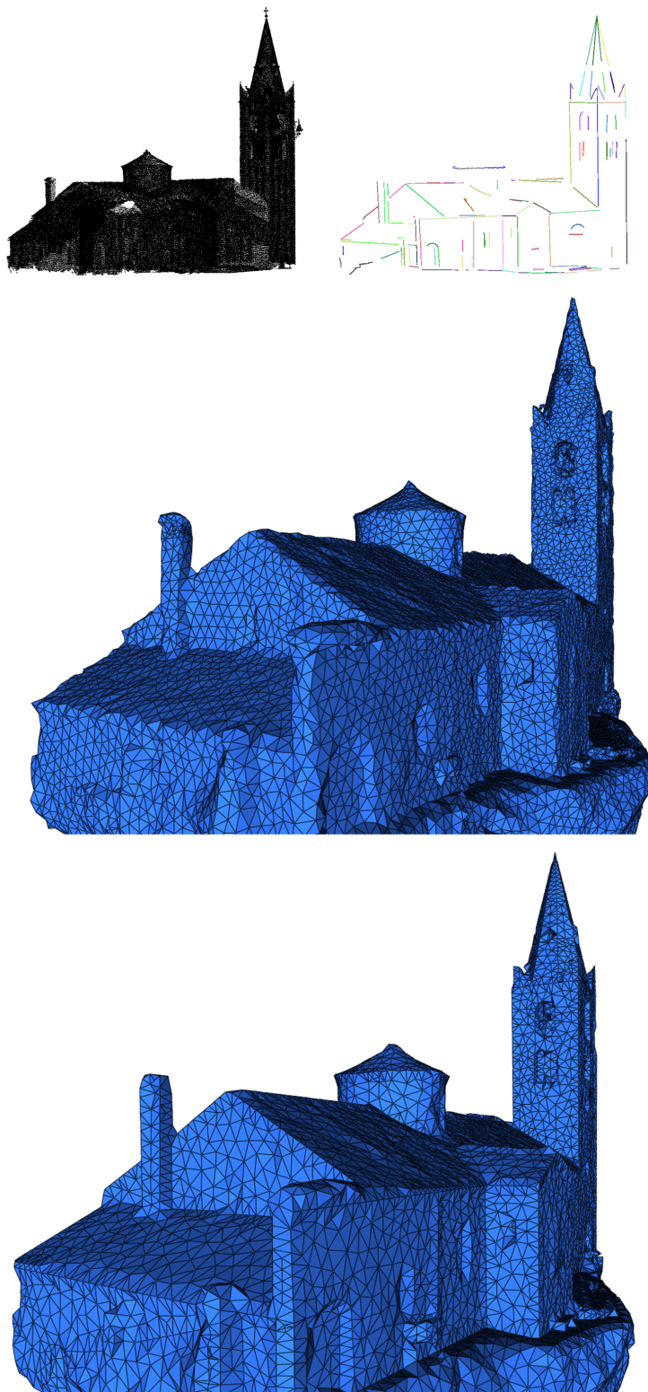
Figure 7.17: From top to bottom, left to right: input point cloud of Church model (courtesy of INPG ) down-sampled to about 7.2% of the original dataset; extracted feature polylines; meshed Poisson implicit function; output of our feature preserving mesh generation (18k facets).
