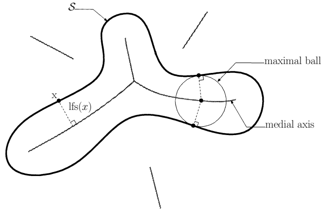
Figure 2.4: Medial axis of a planar curve \mathcal{S} .
