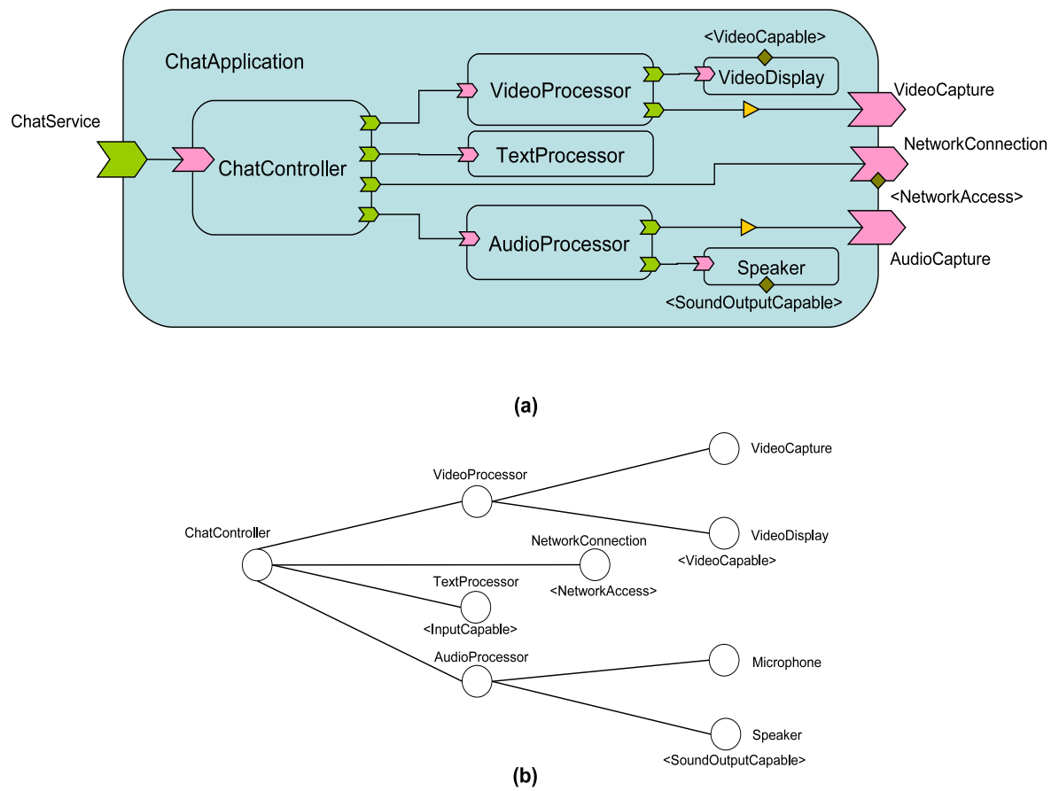
Figure 4.3: Example Chat application (a) SCA composite (b) graph representation
