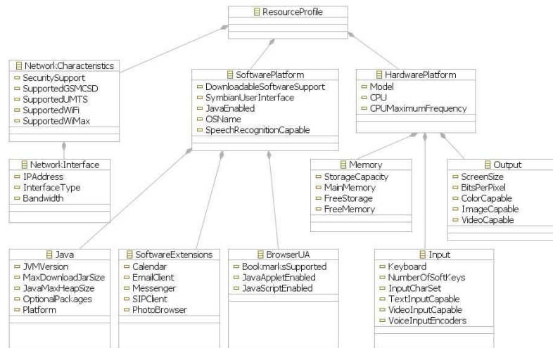
Figure 3.3: The extended CC/PP model
