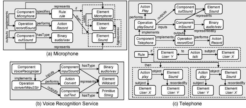
Figure 2.7: Examples of CoSMoS (Fujii and Suda, 2009)
