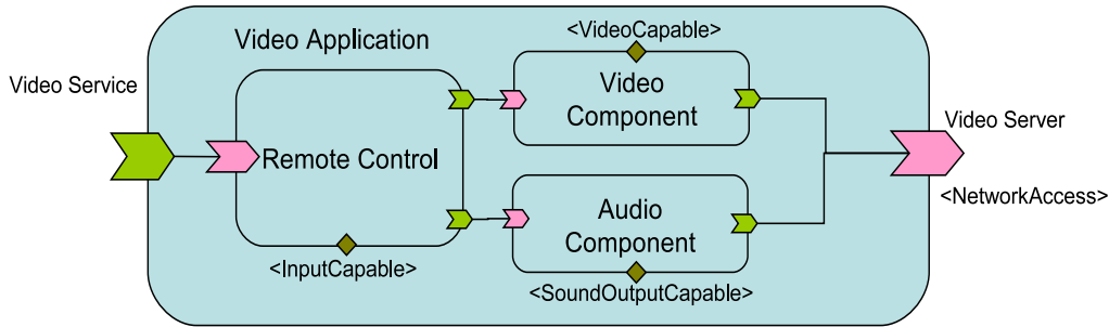
Figure 5.1: Example Video Application in SCA
