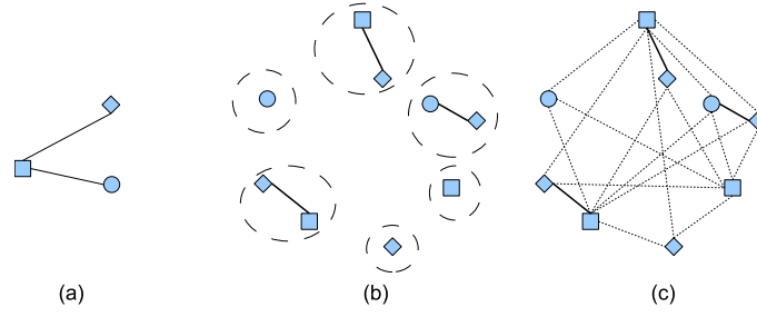
Figure 4.7: (a) User Task Graph (b) Different Devices with Available Components (c) Aggregate Graph
