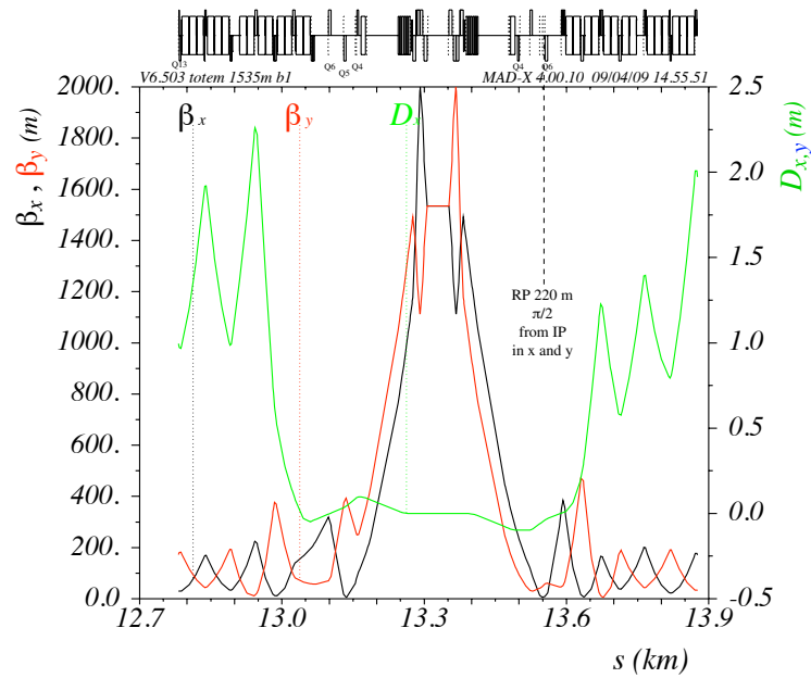
Figure 7.7: Beam 1 optics of the baseline solution.
