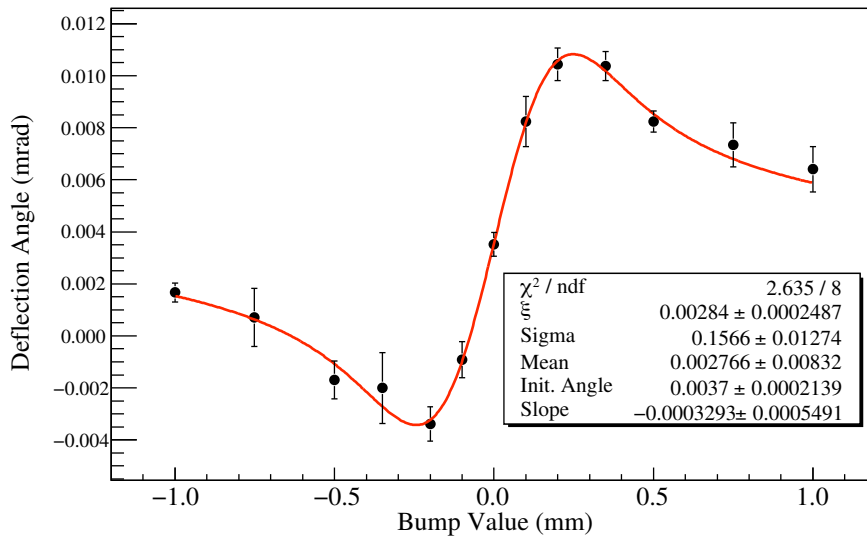
Figure 5.8: Beam-beam deflection scan in the horizontal plane observed at STAR.
