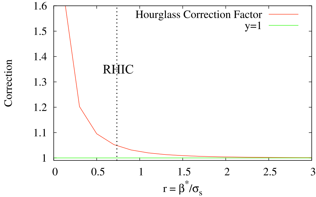
Figure 2.3: Hourglass correction factor as function of r = \beta^*/\sigma_s . RHIC corresponds to r = 0.7 and the LHC to r = 7.3 .
