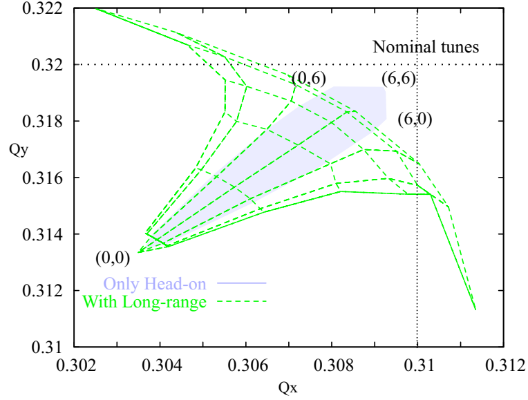
Figure 1.5: Tune footprint with and without long-range interactions. Nominal tunes are 0.31 and 0.32. The coordinates represent the particle amplitude in x and y expressed in units of RMS beam size. The maximum tune shift is observed at (0,0) .
