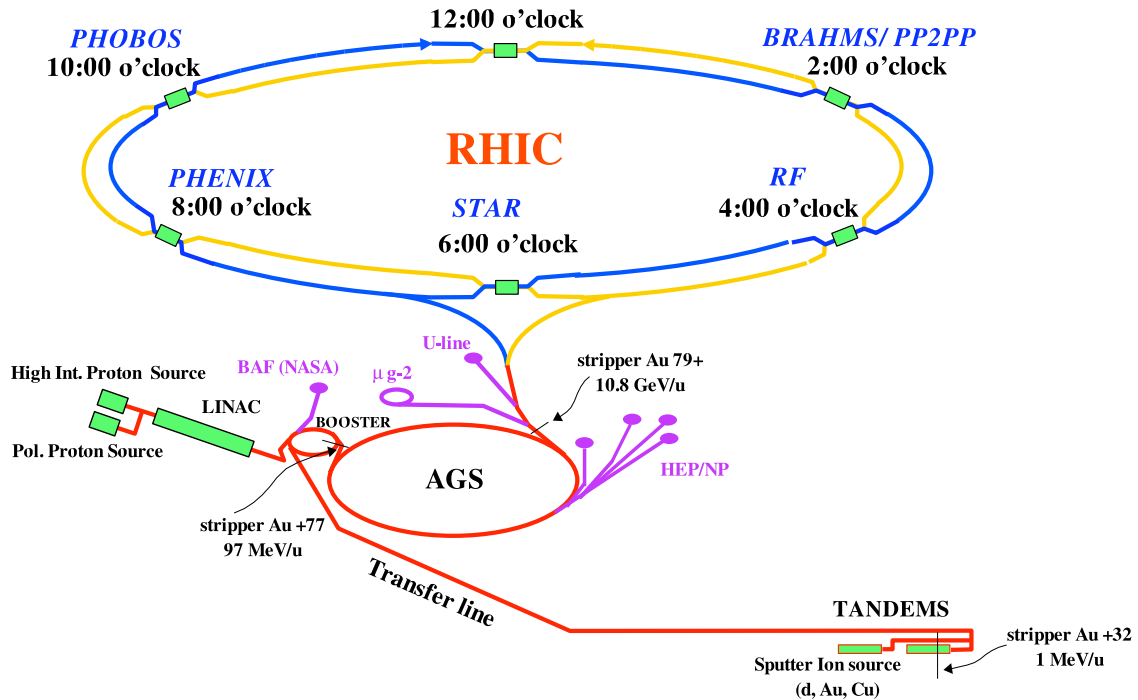
Figure 5.1: The RHIC accelerator complex. The path of the gold ions can be tracked from the TANDEMIS while the polarized protons are first injected from the LINAC into the booster, AGS, and finally into RHIC.
