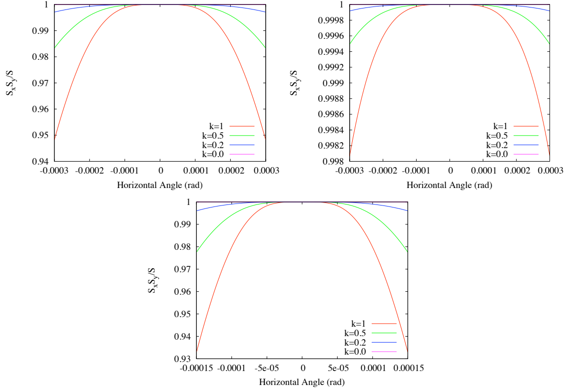
Figure 2.2: Ratio S_x S_y / S for nominal LHC (top left), LHC at 3.5 TeV (top right) with \beta^* = 2 m and RHIC beam parameters with \beta^* = 0.7 m, \sigma_s = 1 m and an energy of 250 GeV (bottom). k represents the ratio between the projected angles, in this case \phi_y / \phi_x . In the actual LHC configuration the error is smaller than 1 % and can be neglected. It becomes relevant for LHC nominal parameters and RHIC.
