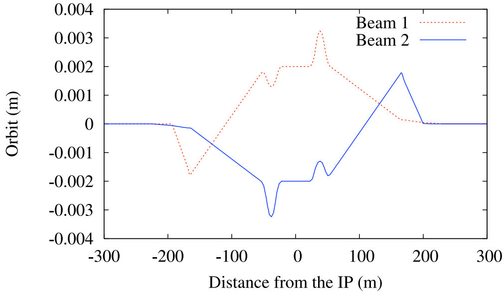
Figure 3.6: Parallel separation bumps at IP5. Vertical plane.
