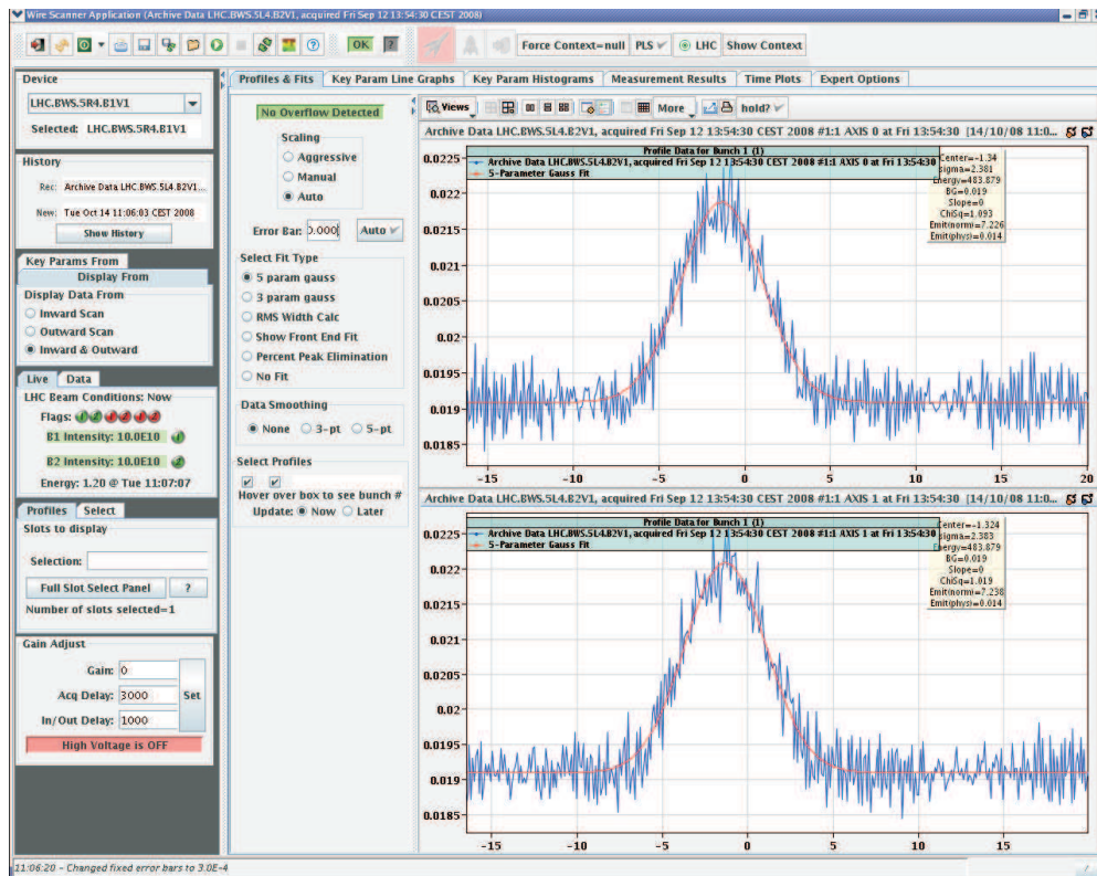
Figure 4.2: Display of the LHC wire scanner application. In and out vertical wire scans on a single circulating pilot bunch [39].
