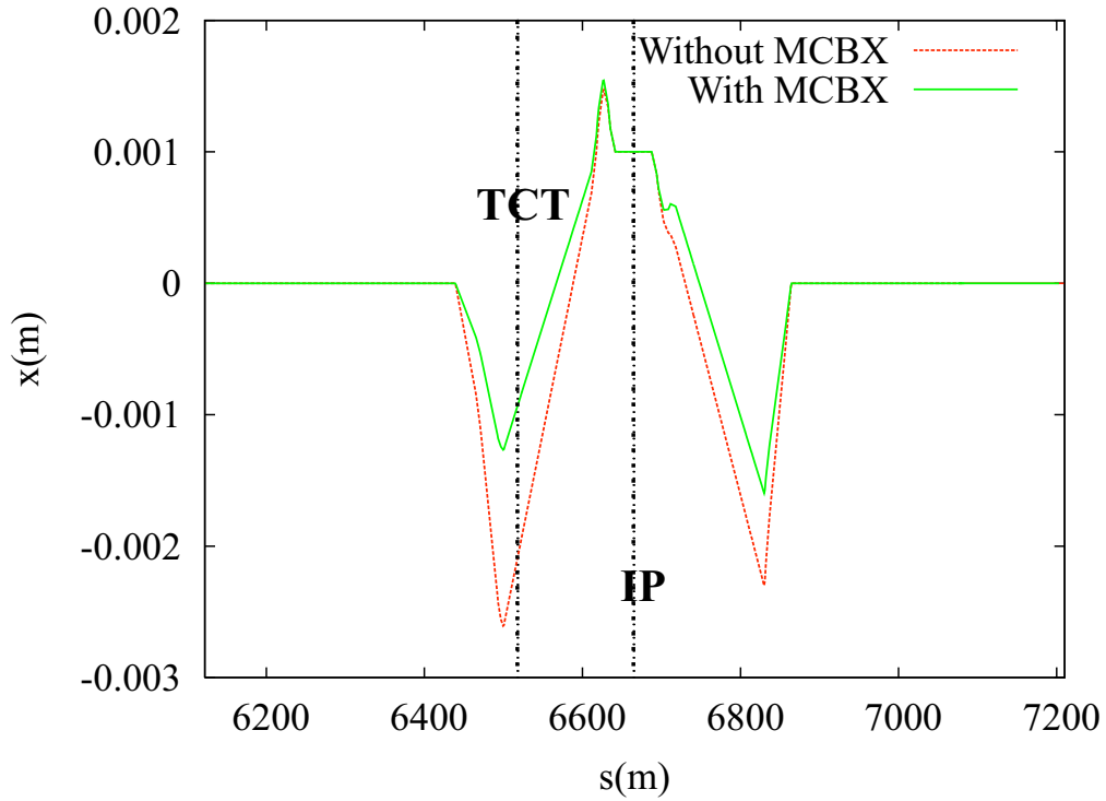
Figure 6.2: Example of closed orbit bumps. The case without MCBX is the one described above, with MCBX is a six magnet bump used for injection which reduces the orbit excursion outside the interaction region. Displacing the beam at the IP also changes the orbit at the tertiary collimator location.
