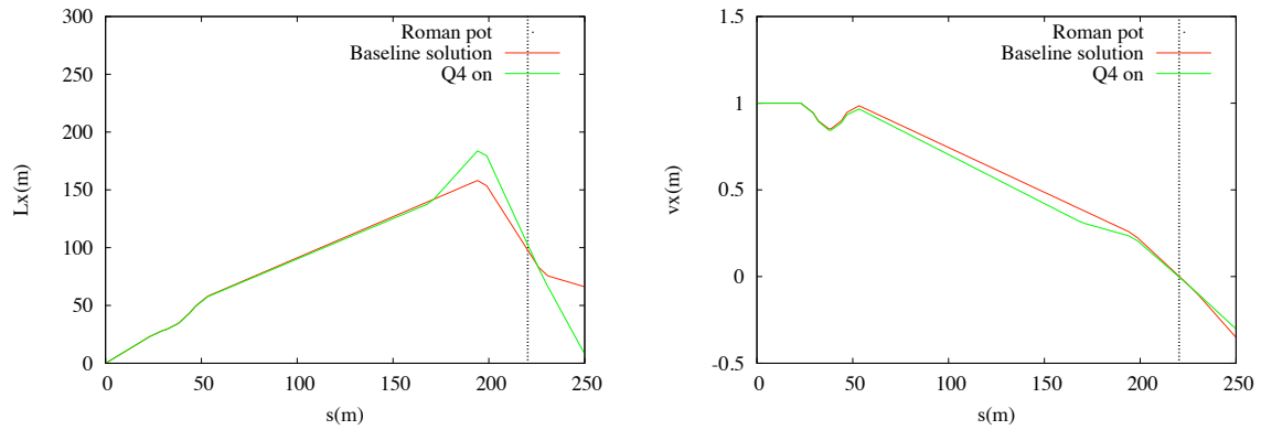
Figure 7.9: Effective length defined in Equation 7.12 (left), magnification defined in Equation 7.13 (right) in the horizontal plane. The performances are similar for both designs.
