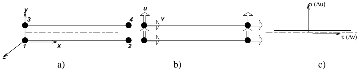
Figure 5.2: Interface 4-nodes element, a) Topology, b) Displacements, c) Stress [102] [103]
