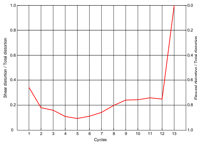
Figure 4.39: Rotation caused by shear effect and flexural effect
