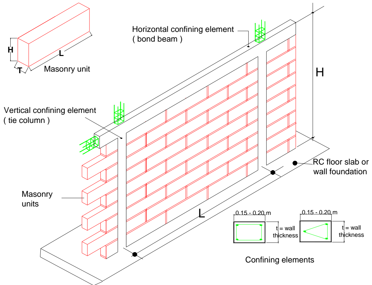
Figure 2.1: Confined masonry wall characteristics [42] [106]
