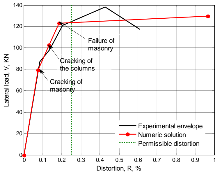
Figure 5.31: Experimental positive envelope by Aguilar (1997) and numeric solution
