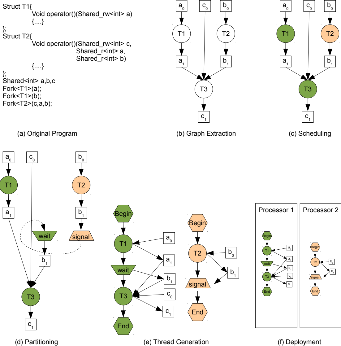
Figure 4.10: Steps of static partitioning in KAAPI: From the original program (a) a data flow graph is extracted (b). Each task is mapped to a partition (c). The tasks are partitioned and the graph enriched with communication tasks (d). Individual stacks of tasks are generated (e). The stacks of tasks (K-Threads) are distributed across the processors (f)
