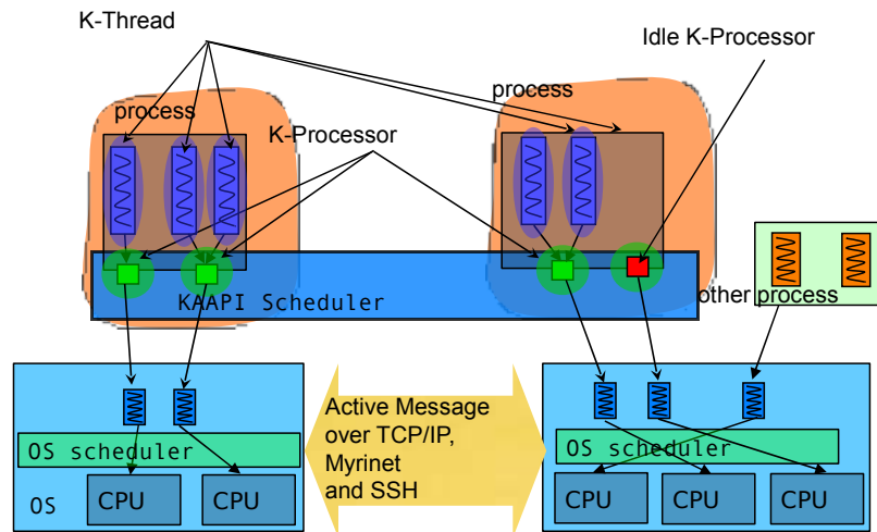
Figure 4.9: Hierarchical structure of KAAPI
