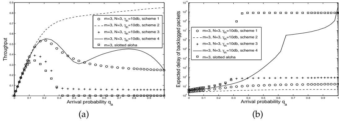
Figure 1.14: Nash equilibrium throughput and EDBP for 4 mobiles when the payoff function is the individual throughput.
