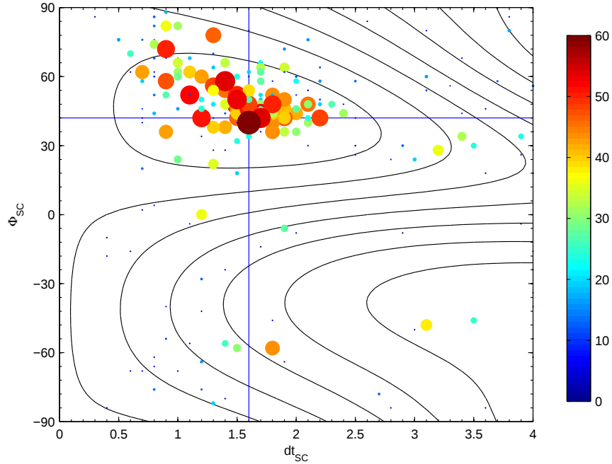
Figure 31: Same as Figure 30, except in (\Phi, dt) parameter plane. Size and color of each symbol represents the amount of non-Null measurements recovered for the corresponding seismogram. The contour lines represent the stacked energy map of all non-Null measurements. This energy map has its minimum for \Phi=42^\circ and dt = 1.6\text{sec} . This is in very good agreement with Barruol & Hoffmann [1999], who manually determined \Phi=48^\circ and dt = 1.59\text{sec}
