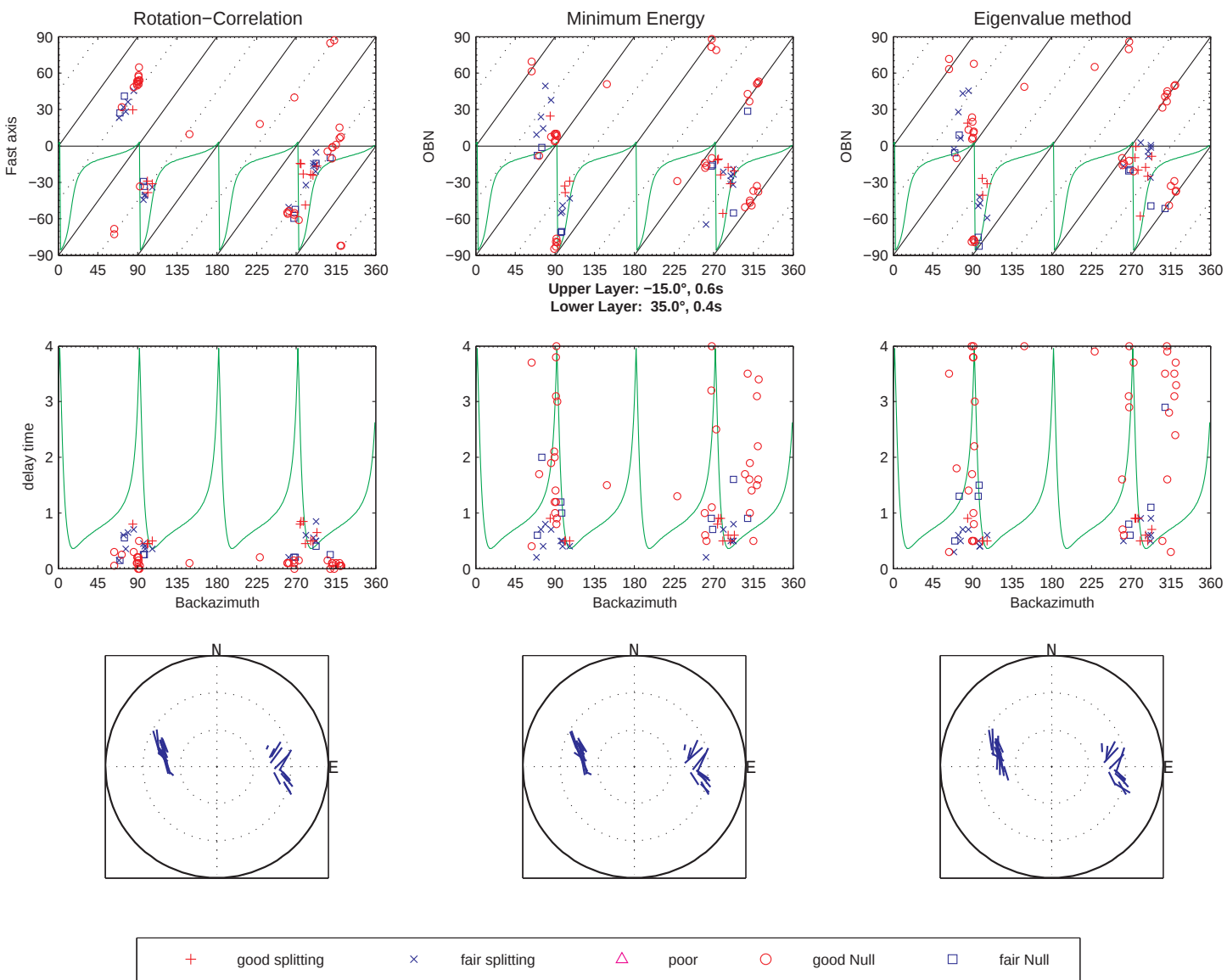
Figure A-15: Backazimuthal plots for station OBN with best two layer model fit at 8sec dominant frequency
