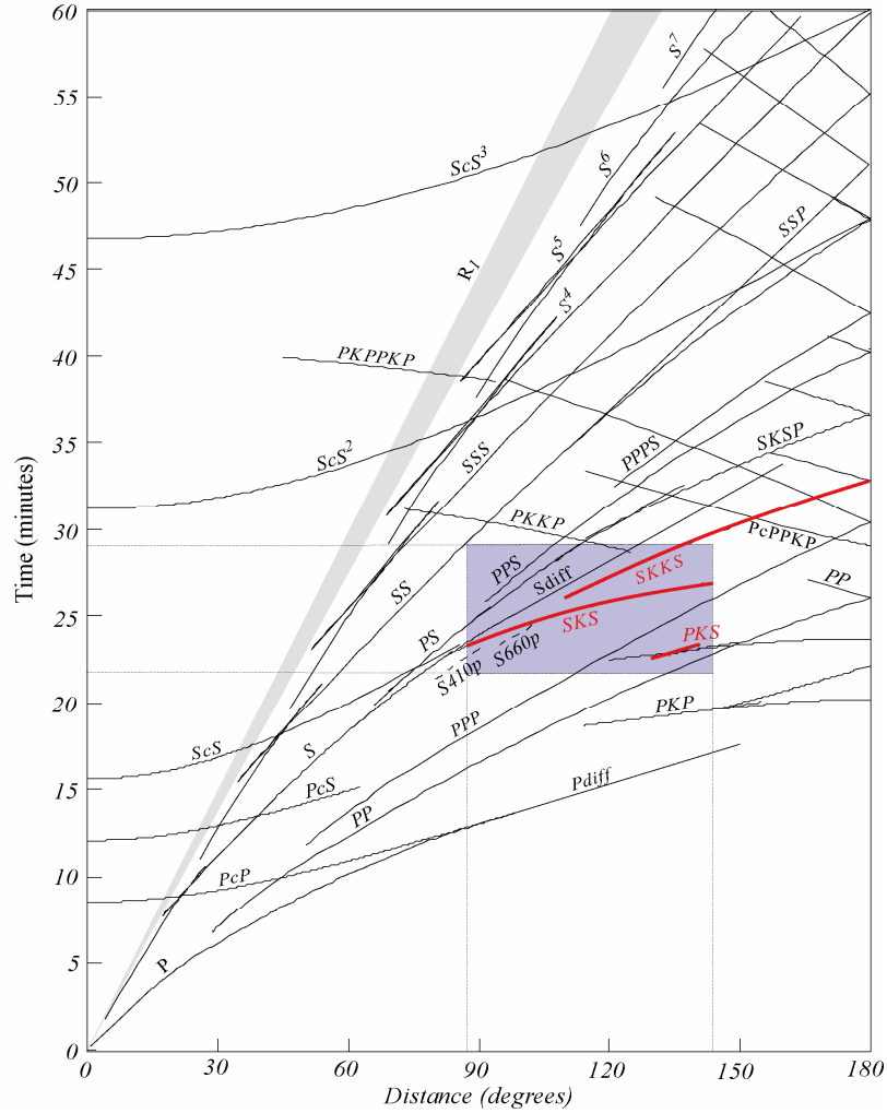
Figure 16: Theoretical phase plot. Core refracted shear-phases used for shear-wave splitting occur at distances between 90° and 145°. Mostly these are well separated from other phases, which could otherwise contaminate the signal of the phase of interest.
