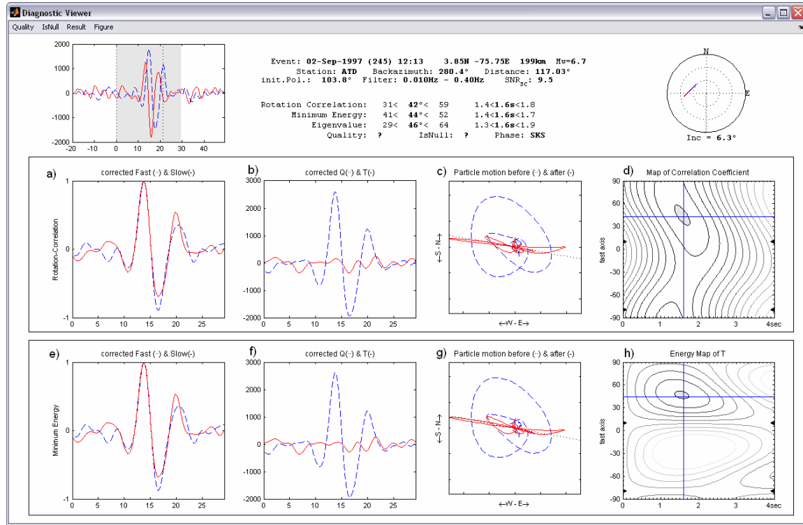
Figure 24: Diagnostic plot of a single measurement. The center panels displays the result for the Rotation-Correlation (RC) technique: a) seismogram components in fast (solid) and slow (dashed) direction for the RC-anisotropy system after RC-delay correction (normalized); b) radial (Q, solid) and transverse (T, dashed) components after RC-correction (not normalized); c) particle motion before (dashed) and after (solid) RC correction; d) map of correlation coefficients. The lower panels display the results for the minimum energy (SC) technique: e) seismograms shown after splitting correction shown on SC-fast and slow components (normalized); f) same on radial and transverse components (not normalized); g) SC particle motion before and after correction; h) map of minimum energy values on transverse component. In the upper left an extended section of the Q (solid) and T (dashed) components before anisotropy correction is displayed. In the upper right a stereoplot of the result is presented. The header gives specifications of the event as well as splitting parameters resulting from the three techniques. Depending of the chosen option, the lower panels e) - h) may display instead of the SC the results of the EV technique
