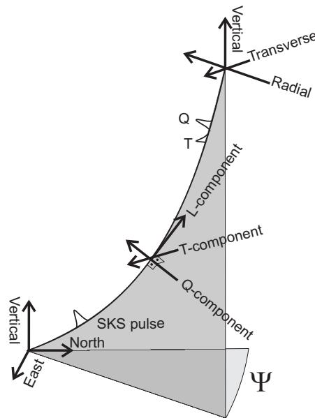
Figure 22: Components of a seismogram in a right-handed L-Q-T system. The ray plane, shown in grey, is given by the L-component (parallel to the ray) and the Q-component (pointing towards the earthquake). The T-component is perpendicular to this ray plane. \Psi is the backazimuth.
