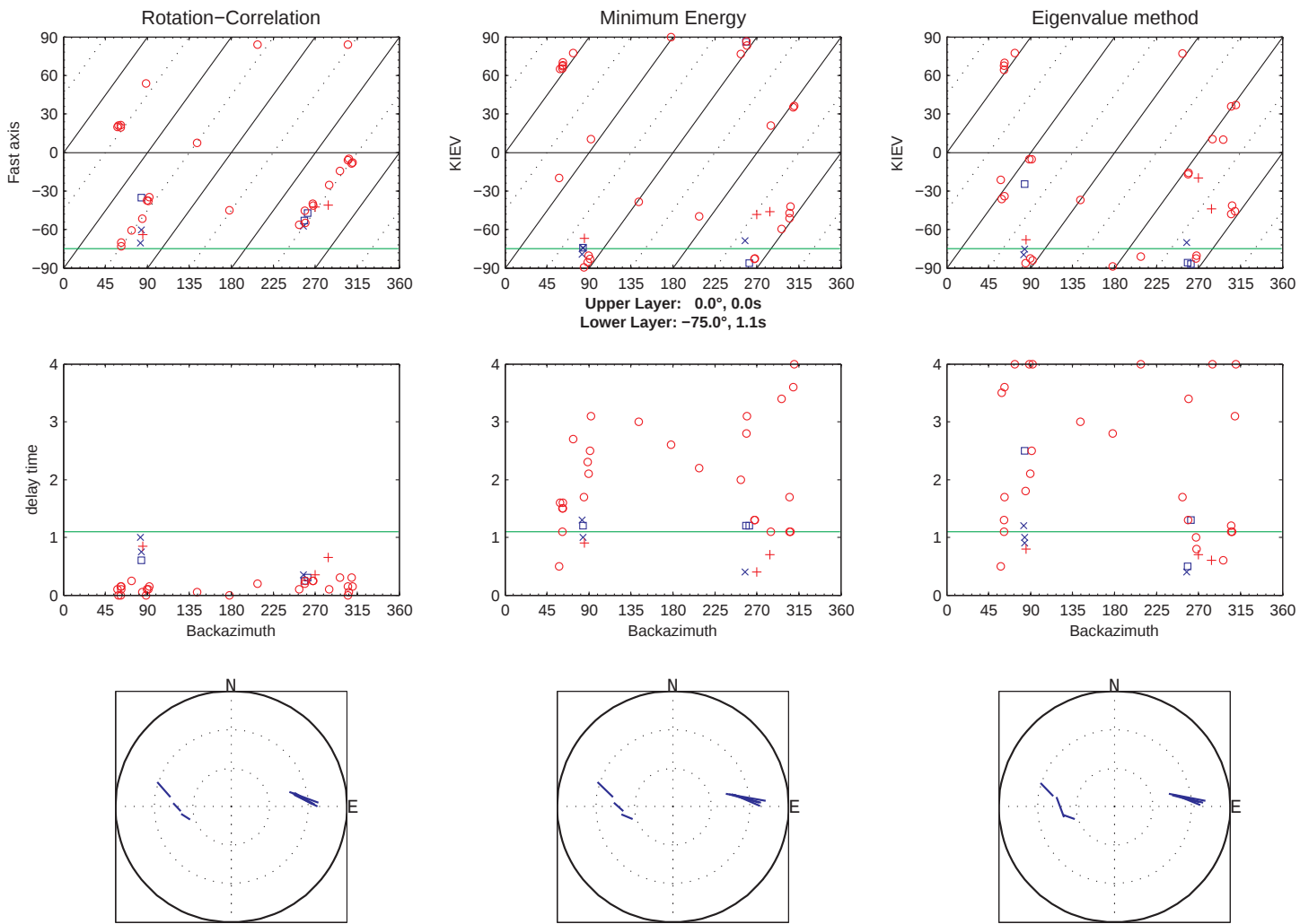
Figure A-6: KIEV backazimuthal plots
