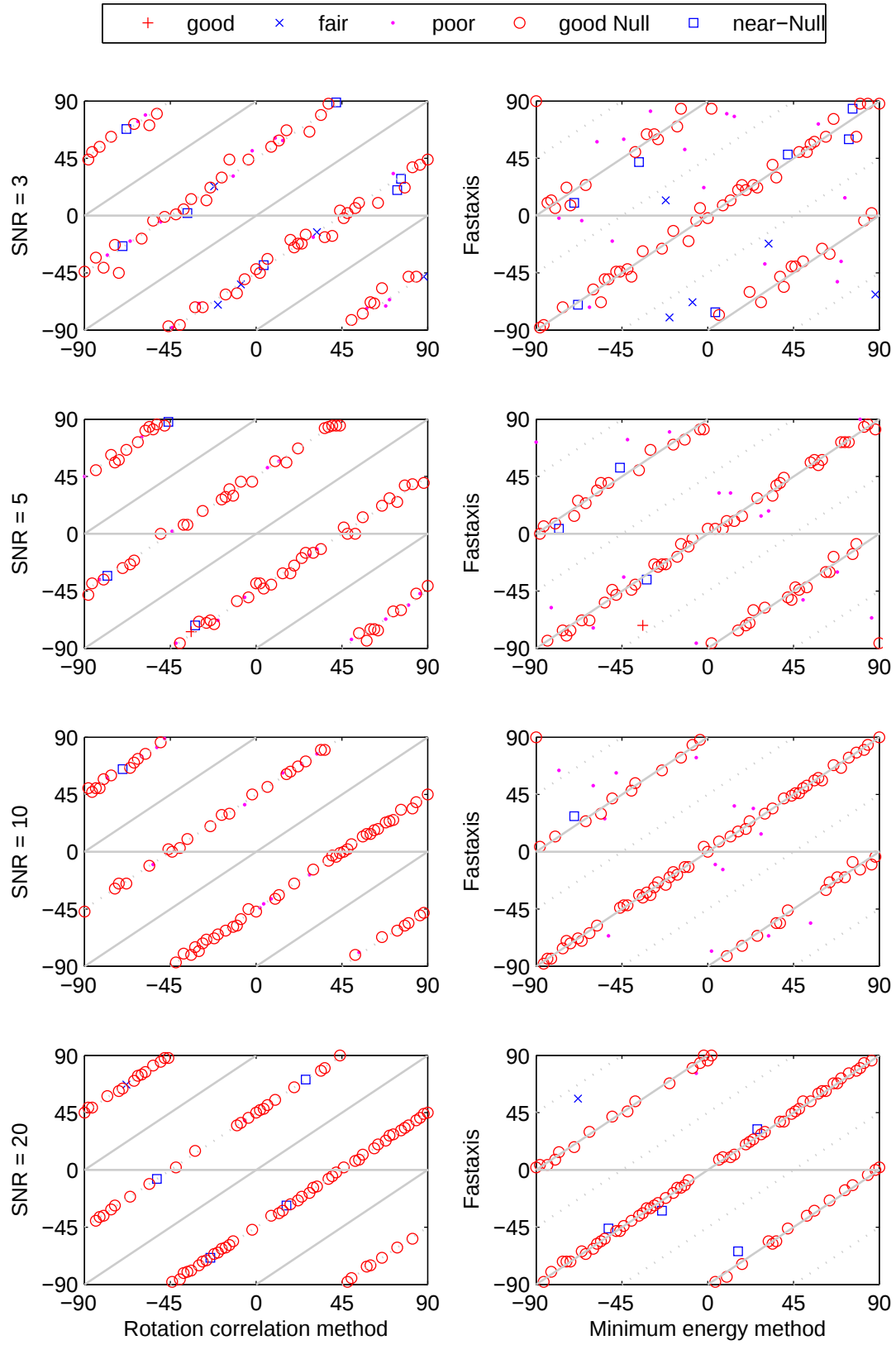
Figure B-1: Comparison of RC and SC fast axis estimates for different SNR. Model fast axis at 0° and delay time 0.0 seconds.
