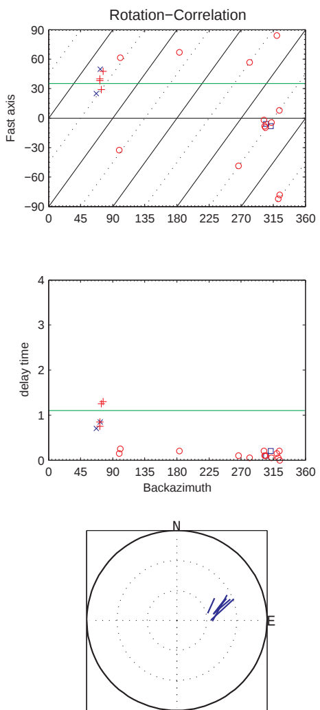
Figure A-8: Backazimuthal plots for station MHV with best single layer model fit
