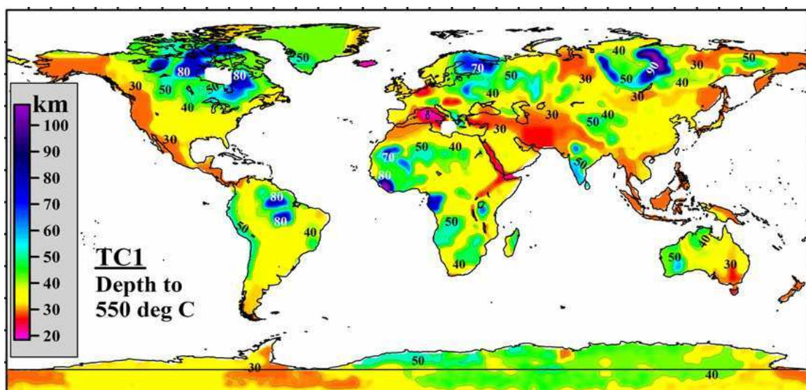
Figure 45: Global thermal model for the continental lithosphere constrained on a 1^\circ \times 1^\circ grid: depth to the 550°C isotherm interpolated with a low-pass filter [Artemieva, 2006].
