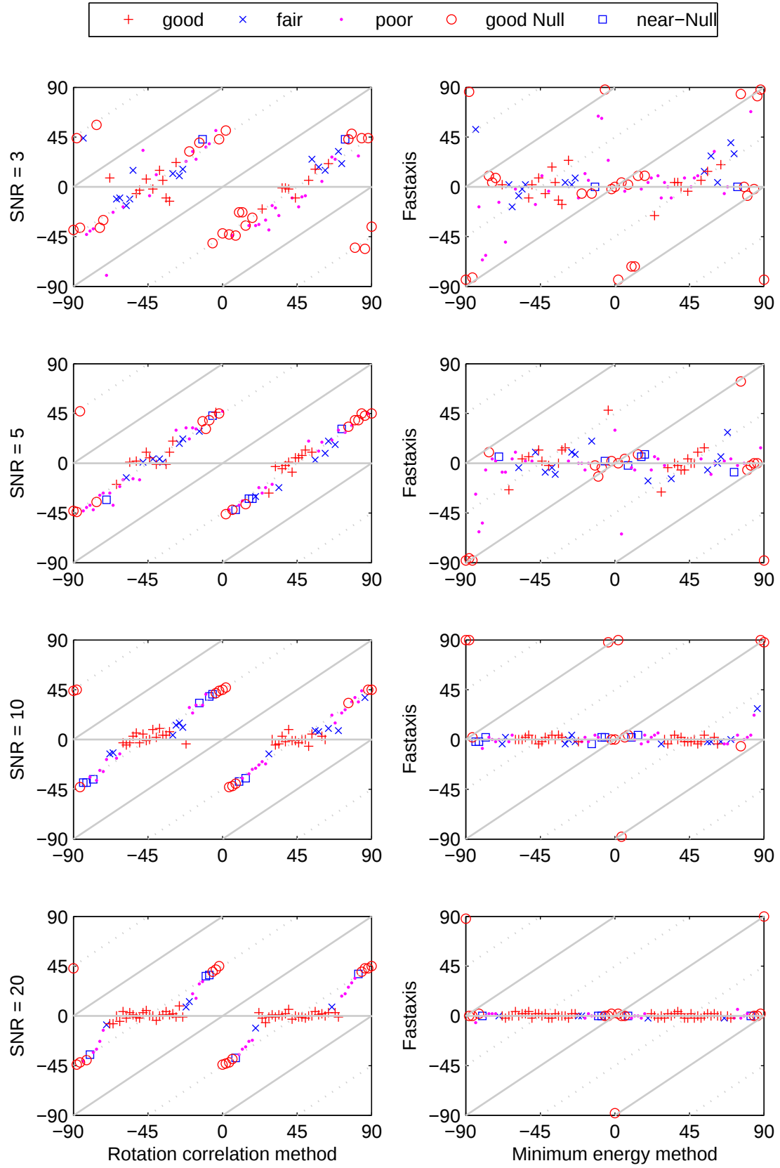
Figure B-11: Comparison of RC and SC fast axis estimates for different SNR. Model fast axis at 0° and delay time 1.5 seconds.
