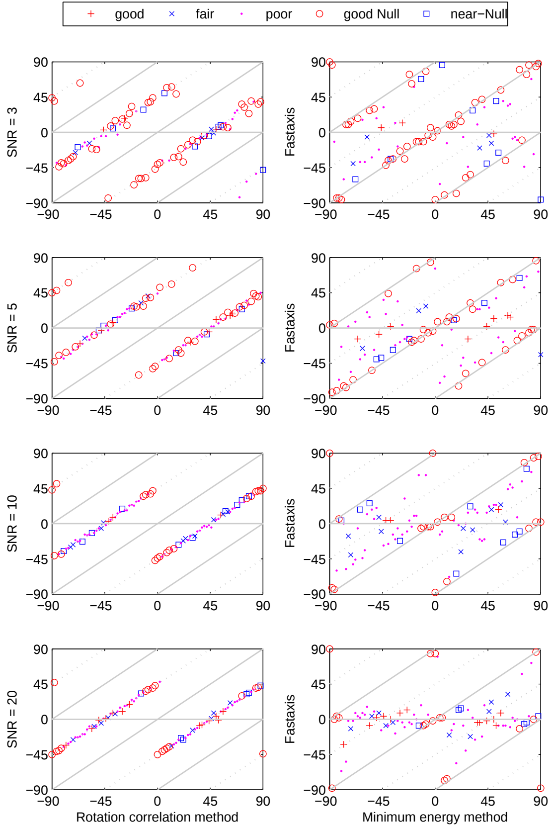
Figure B-3: Comparison of RC and SC fast axis estimates for different SNR. Model fast axis at 0° and delay time 0.5 seconds.
