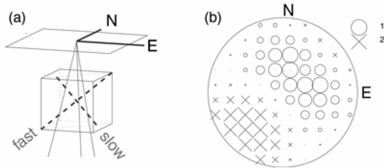
Figure 5: a) Ray geometry through an anisotropic block of dipping anisotropy. The fast axis is dipping 30^\circ to the SW, the intermediate axis is dipping 60^\circ to the NE, and the slow axis is horizontal. b) The lower hemisphere shows predicted fast/slow delays (crosses and circles respectively; given in sec) for a propagation through a 150 km anisotropic layer defined in a). [after Bokelmann, 2002b]
