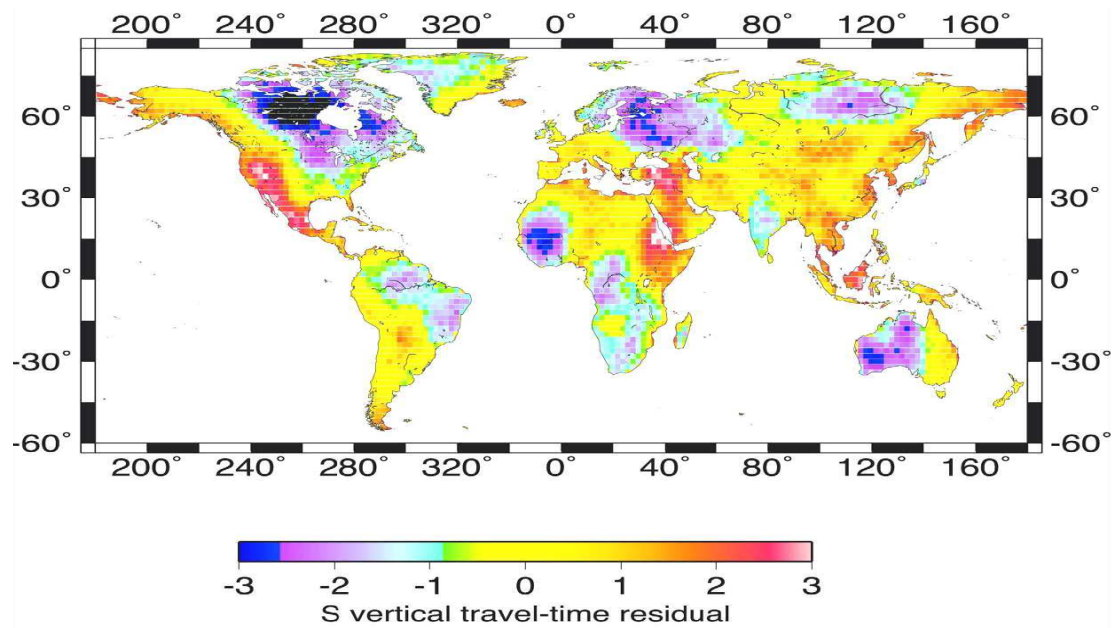
Figure 43: Map of one-way S_V travel time residuals deduced from surface-wave tomography [Shapiro & Ritzwoller, 2002] (after Poupinet et al., [2003]). The blue color represents early arrivals (and thus cooler material) and the late arrivals (warmer). The magnitude of the residual is inverse proportional to the lithospheric thickness. All Precambrian shields are fast and the S -vertical travel time increases regularly outwards from the centers of shields.
