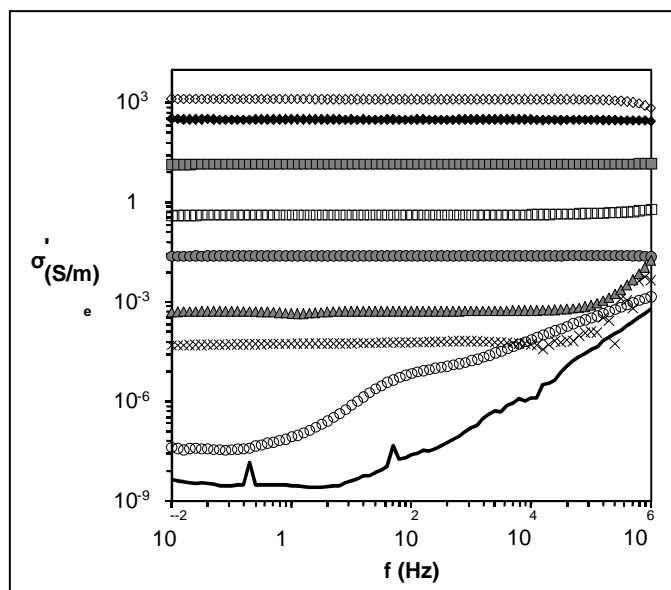
Figure 26 : real part of the conductivity as a function of frequency of the applied field for the P(S-ABu) matrix (—), the composite filled by 0.2 vol% ( \blacktriangle ), 0.5 vol% ( \bullet ) et 3 vol% ( \blacksquare ) of MWNTs processed by evaporation (full symbols) or processed by freeze drying (open symbols). Experimental results also for SDBS surfactant (sodium dodecyl benzyl sulfate) ( \times ), a SDBS/MWNTs film ( \blacklozenge ) and a MWNT film ( \blacklozenge ).
