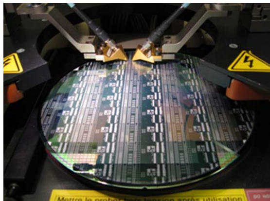
Figure 5.14 Snapshot of measurement with 2 probes GSG
