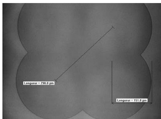
Figure 4.25 Vapor HF etching \text{SiO}_2 layer during 20 hours throughout hole of 1.2 \mu\text{m} in diameter after wet HF etching
