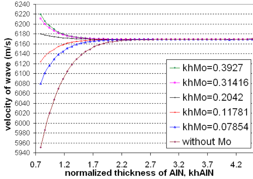
Figure 2.7 Wave velocity AIN/Mo/Si substrate depends on the normalized thickness kh_{AIN} and kh_{Mo}
