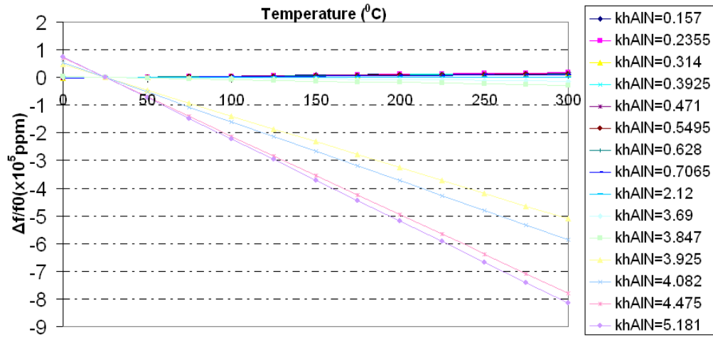
Figure 3.3 \Delta f/f_0(\text{ppm}) depending on temperature in SAW device: AlN/SiO 2 (khSiO 2 =0.3927)/Si substrate
