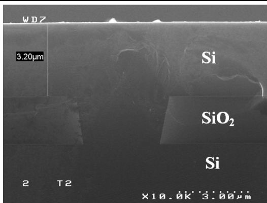
Figure 4.14 Slide view of 2μm wide trench, non selective epitaxy
