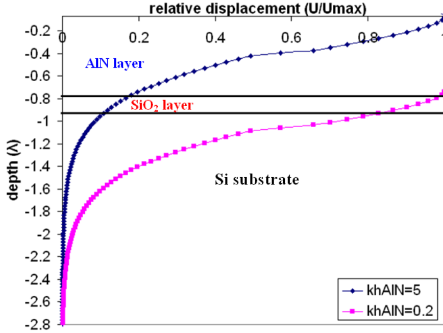
Figure 2.6 Displacement profile along the depth of the multilayer AlN/SiO 2 /Si, kh\text{SiO}_2=0.7854
