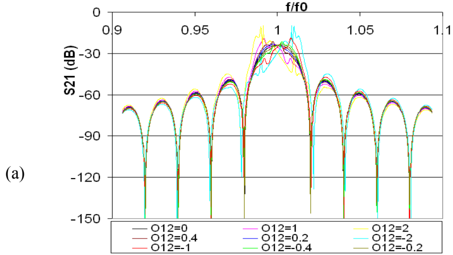
Figure 2.21 Effect of O_{12} on S_{21}(\text{dB}) , N=50 , v_{\text{SAW}}=5120\text{m/s} , \lambda=8\mu\text{m} , K=0.066453 , O_{11}=0
