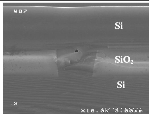
Figure 4.17 Slide view of 3μm wide trench, selective epitaxy
