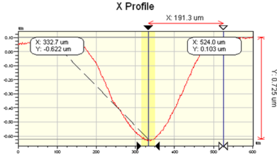
Figure 5.36 Measured membrane deformation
