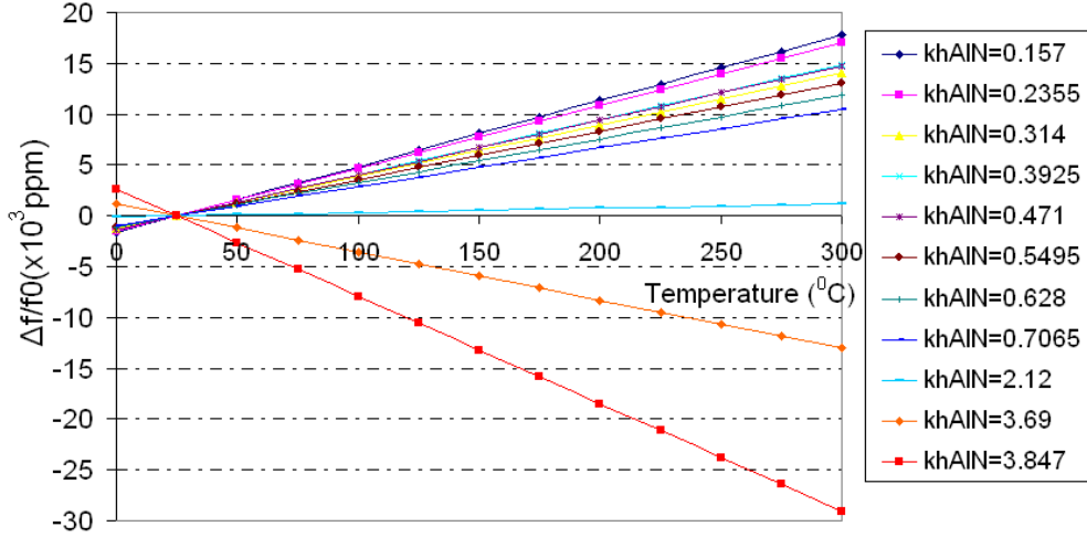
Figure 3.4 \Delta f/f_0(\text{ppm}) depending on temperature in SAW device: AlN/SiO 2 (khSiO 2 =0.3927)/ Si substrate
