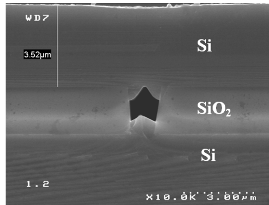
Figure 4.13 Slide view of 1.2μm wide trench, selective epitaxy
