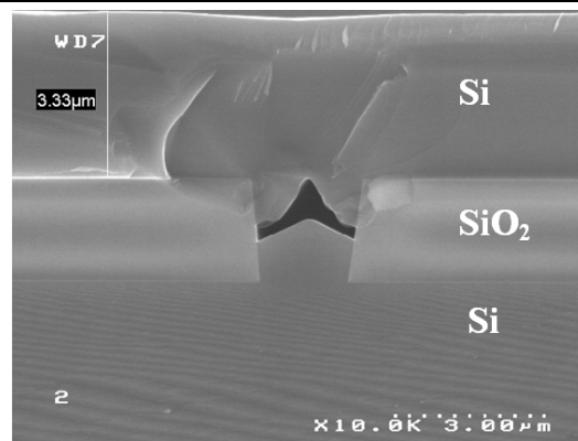
Figure 4.15 Slide view of 2μm wide trench, selective epitaxy
