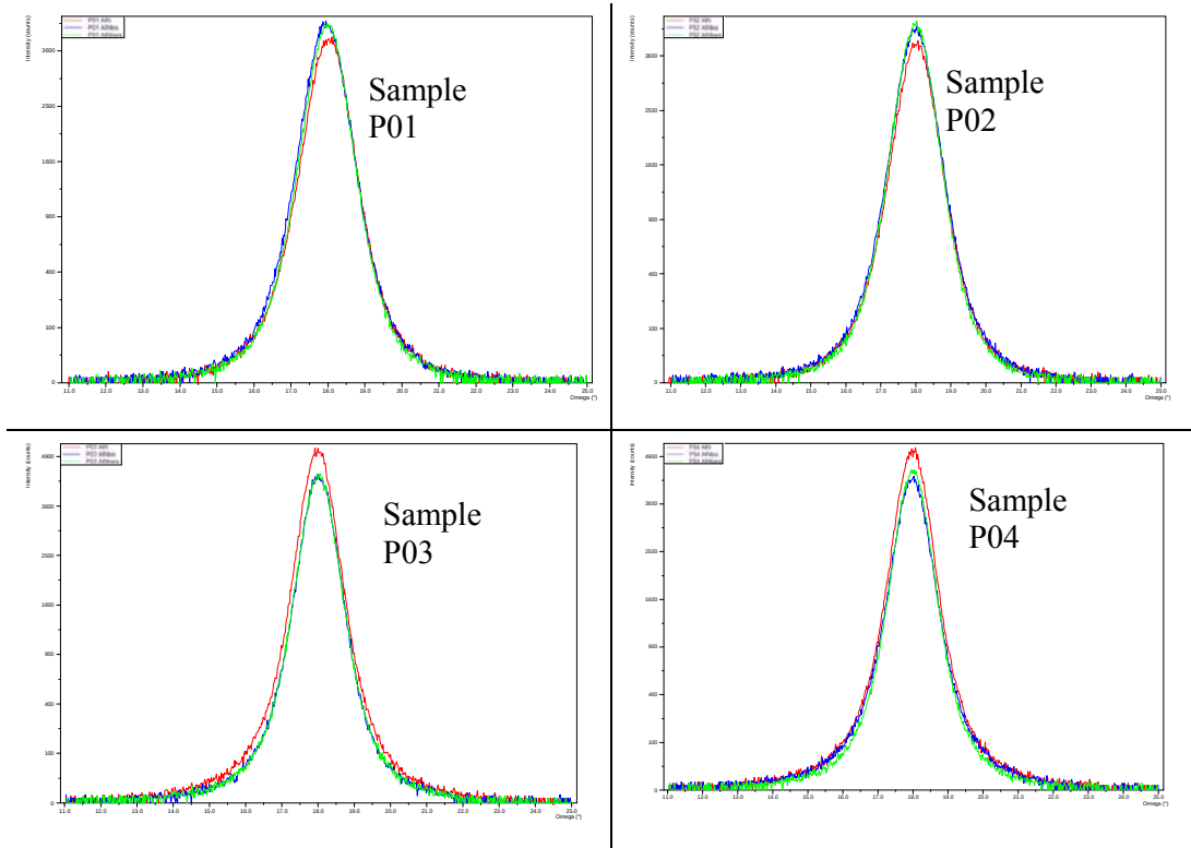
Figure 4.45 FWHM of AlN 1 \mu m films for four samples. The red line is measure 1, the green line is measure 2, and the blue line is measure 3
