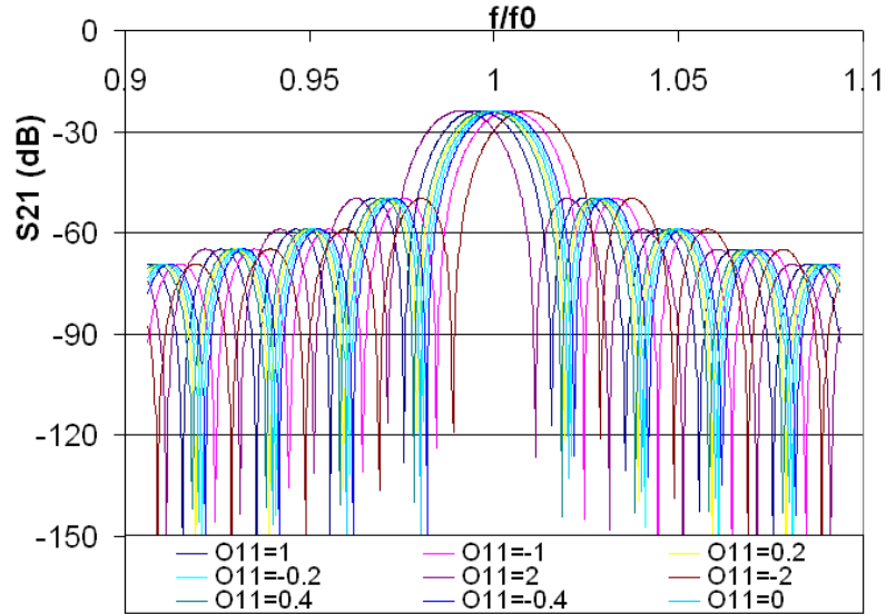
Figure 2.22 Effect of O_{11} on S_{21}(\text{dB}) , N=50 , v_{\text{SAW}}=5120\text{m/s} , \lambda=8\mu\text{m} , K=0.066453 , O_{12}=0
