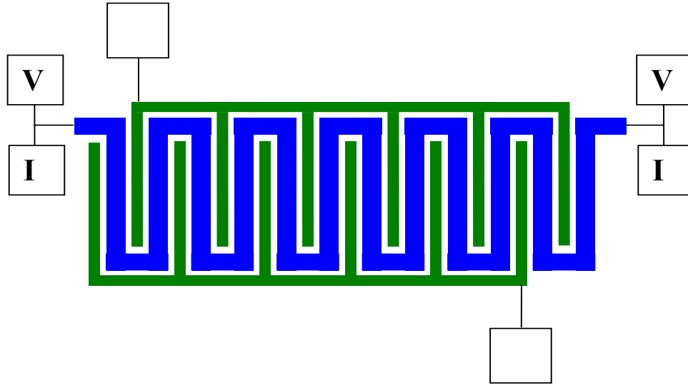
Figure 5.2 The pattern for checking the isolation and continuity
