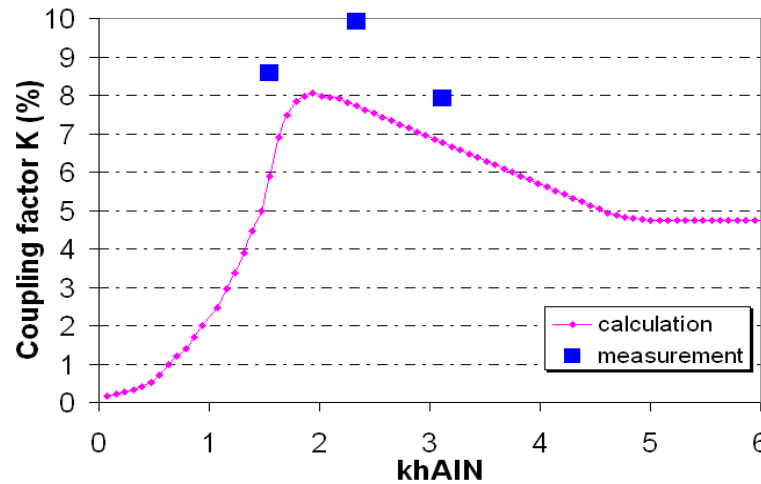
Figure 5.23 Coupling factor K(%) in AlN/SiO 2 /Si, comparison between calculation and measurement
