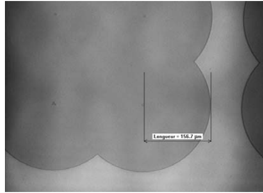
Figure 4.29 Vapor HF etching SiO 2 layer during 20 hours throughout hole of 3µm in diameter after wet HF etching
