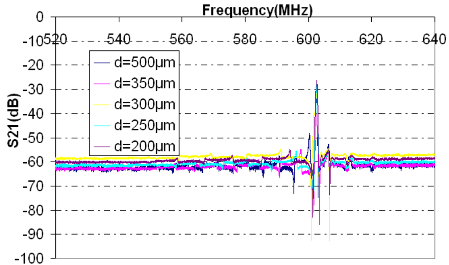
Figure 3.12 The measurement of frequency shift only by different delay line
