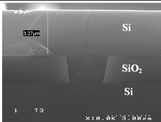
Figure 4.16 Slide view of 3μm wide trench, non selective epitaxy
