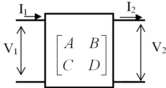
Figure B. 11 [ABCD] representation of two-port network for one IDT
