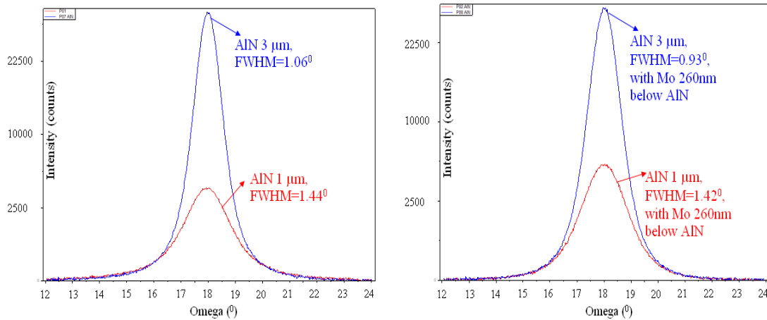
Figure 4.43 The FWHM of 1 \mu m and 3 \mu m AlN films, (a) without Mo layer below AlN, (b) with Mo layer below AlN
