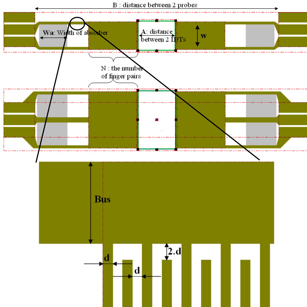
Figure 4.5 Description of devices Table 4.2 THE DIMENSION OF DEVICES
