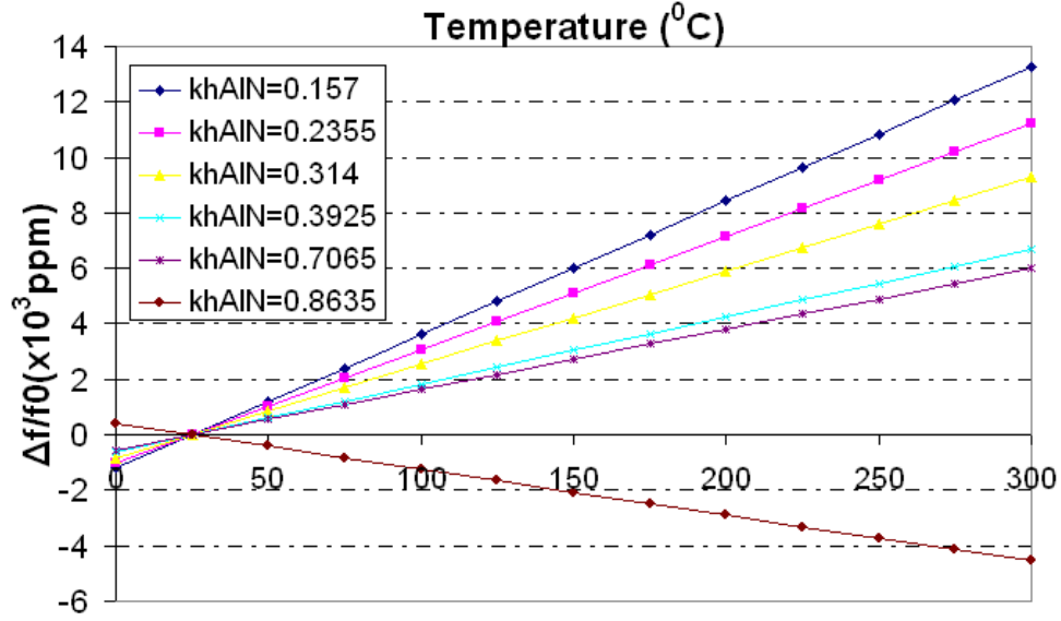
Figure 3.2 \Delta f/f_0(\text{ppm}) depending on temperature in SAW device: AlN/SiO 2 (khSiO 2 =0.0785)/Si substrate
