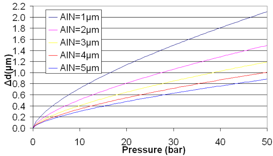
Figure 3.7 \Delta d in multilayer: Si (1 \mu\text{m} ), \text{SiO}_2 (200nm), AlN (1-5 \mu\text{m} )
