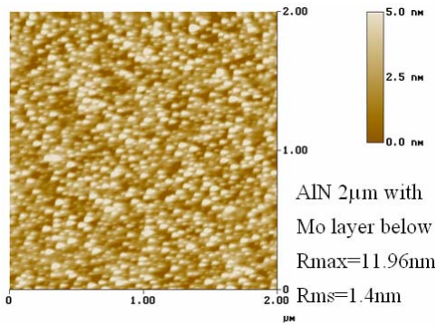
Figure 5.28 Atomic force micrographs of AlN 2 \mu m with Mo layer below
