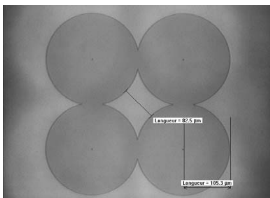
Figure 4.24 Wet HF 49% etching \text{SiO}_2 layer during 110 minutes throughout hole of 1.2 \mu\text{m} in diameter
