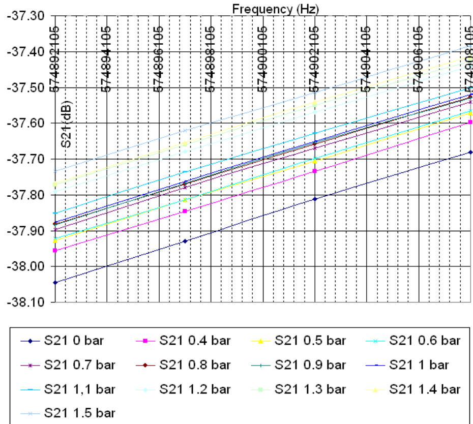
Figure 5.38 S_{21} variation under pressure
