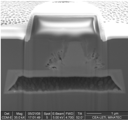
Figure 4.40 SEM slide view 1 of PSG plug
