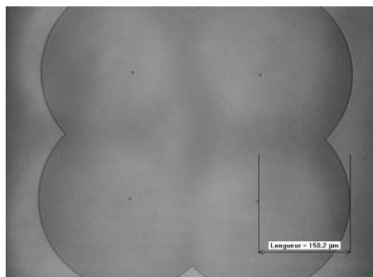
Figure 4.27 Vapor HF etching \text{SiO}_2 layer during 20 hours throughout hole of 2 \mu\text{m} in diameter after wet HF etching
