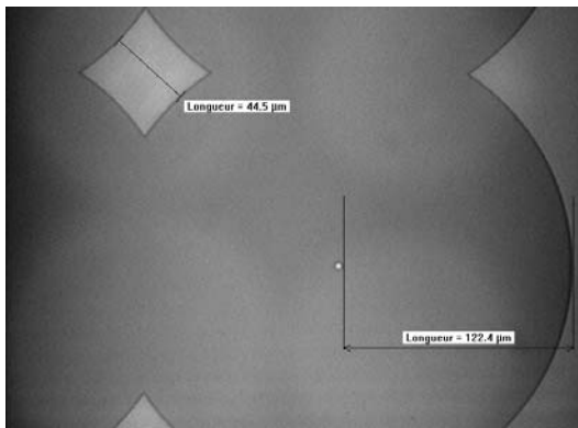
Figure 4.30 Wet HF 49% etching SiO 2 layer during 110 minutes throughout hole of 4µm in diameter
