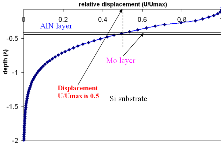
Figure 2.9 Displacement profile along the depth of the multilayer AlN/Mo/Si, kh_{\text{AlN}}=2.7
