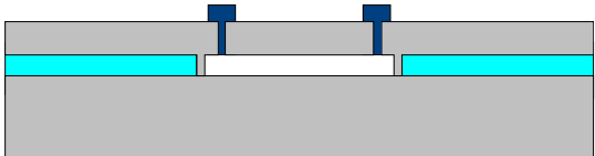
Figure 4.39 Etching PSG
