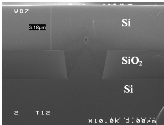
Figure 4.12 Slide view of 1.2μm wide trench, non selective epitaxy
