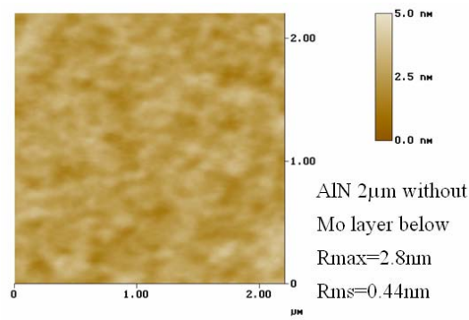
Figure 5.29 Atomic force micrographs of AlN 2 \mu m without Mo layer below
