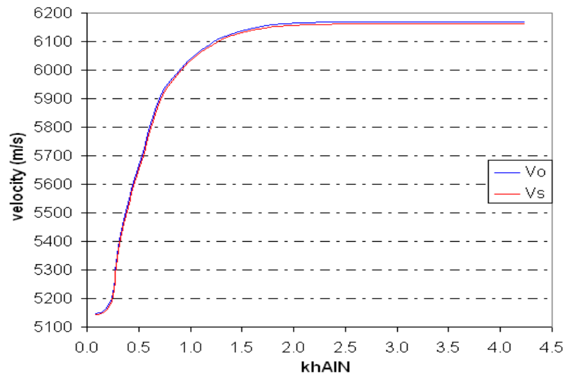
Figure 2.2 Calculated values of wave velocity V_0 and V_s in SAW device AlN/Si substrate depend on the normalized thickness kh_{\text{AlN}} of AlN layer
