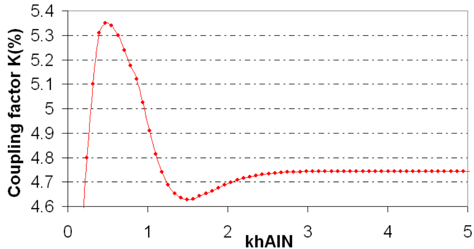
Figure 2.3 Calculated values of coupling factor K(\%) in SAW device AlN/Si substrate depends on the normalized thickness kh_{\text{AlN}} of AlN layer
