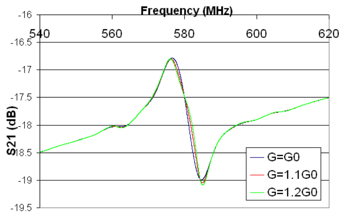
Figure 5.35 Simulation of S_{21}(\text{dB}) , effects of polyimide films on the f_0
