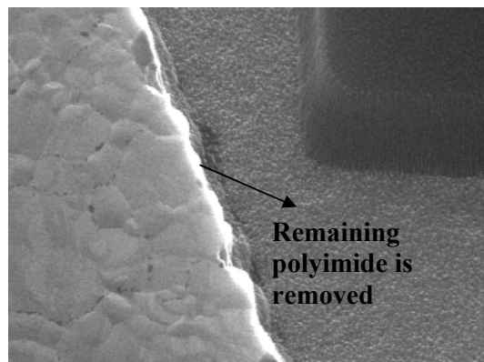
Figure C. 3 Etching polyimide during 180s
