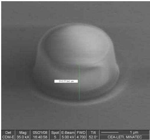
Figure 4.41 SEM image of a PSG plug
