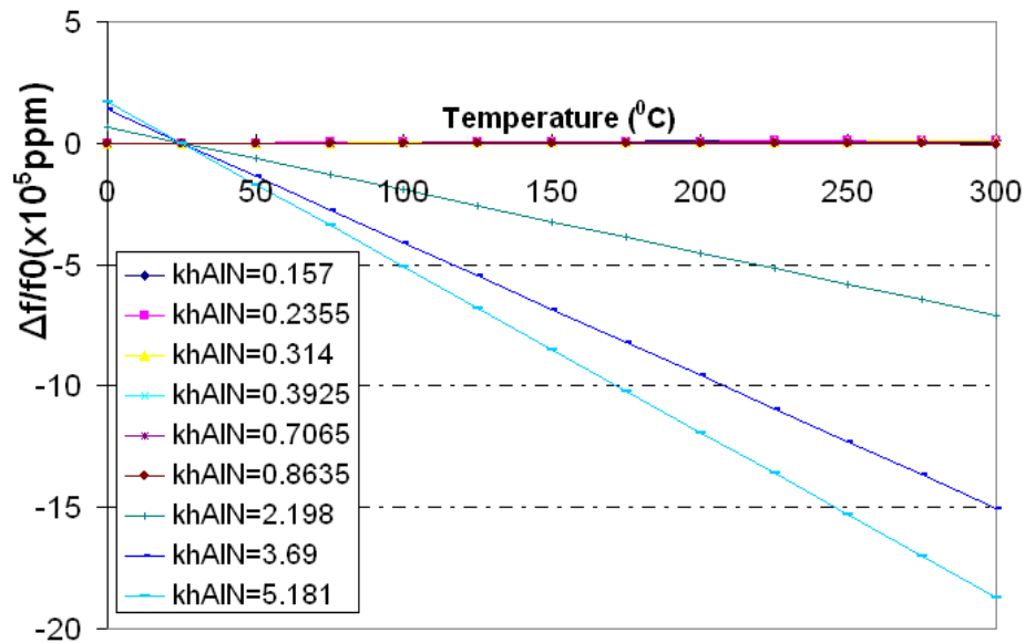
Figure 3.1 \Delta f/f_0(\text{ppm}) depending on temperature in SAW device: AlN/SiO 2 (khSiO 2 =0.0785)/Si substrate
