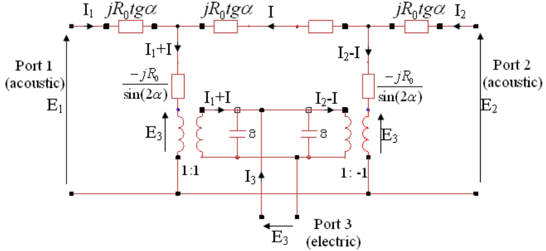
Figure B. 1 Mason equivalent circuit for one periodic section in “crossed-field” model
