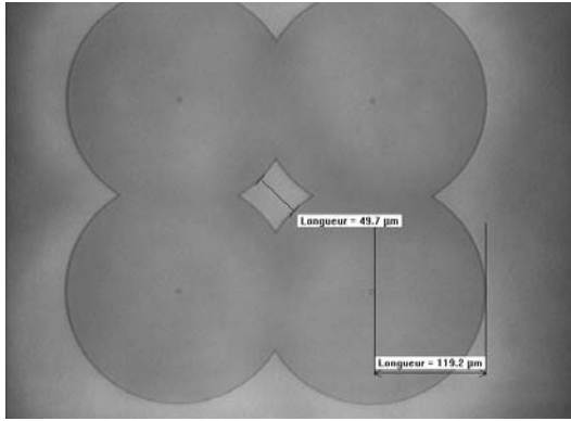
Figure 4.28 Wet HF 49% etching SiO 2 layer during 110 minutes throughout hole of 3µm in diameter
