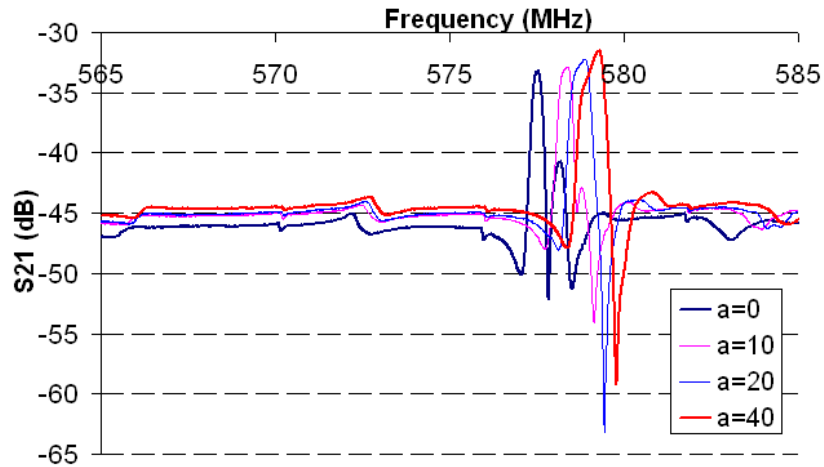
Figure 5.31 S_{21}(\text{dB}) with different lengths of polyimide
