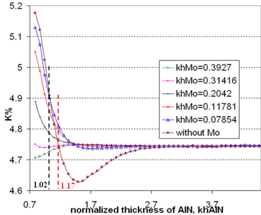
Figure 2.8 Coupling factor K(\%) in SAW device AIN/Mo/Si substrate depends on the normalized thickness kh_{AIN} and kh_{Mo}
