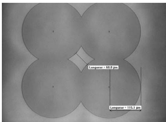
Figure 4.26 Wet HF 49% etching \text{SiO}_2 layer during 110 minutes throughout hole of 2 \mu\text{m} in diameter
