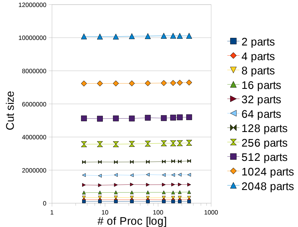
PT-Scotch 45MILLIONS
