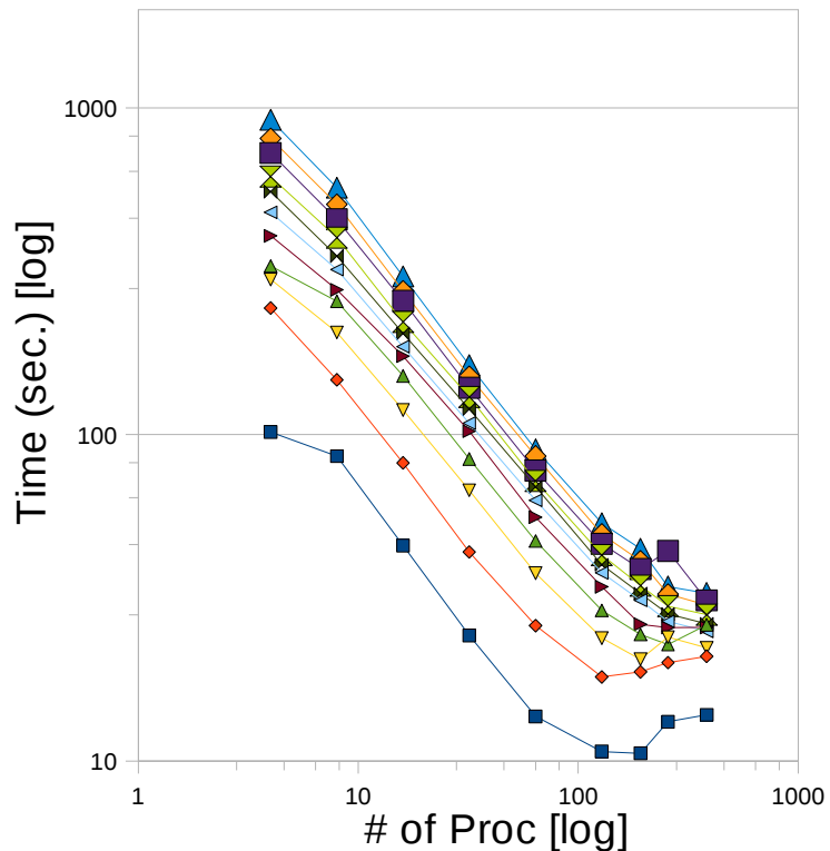
PT-Scotch 45MILLIONS
