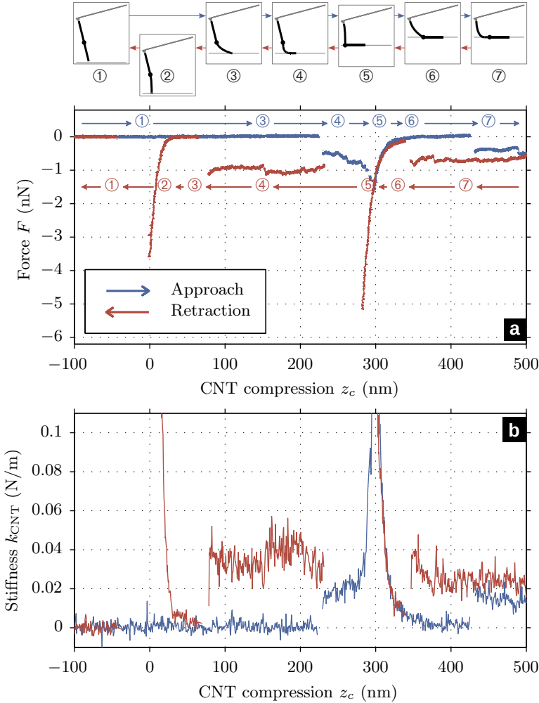
Figure 4.5 — Force F and dynamic stiffness k_{\text{CNT}} of a nanotube as a function of its compression on a graphite substrate. A strong hysteresis, due to adhesion, can be noted between approach (blue) and retraction (red). Well defined plateaux of force (around 0.98 nN) and stiffness (around 0.036 N/m) allow one to estimate the energy of adhesion of the CNT on graphite ( E_a^{\text{HOPG}} = 0.98 \text{ nJ/m} ), as well as the nanotube mechanical properties. The jumps and steep peaks of the curves are signature of transitions between contact and adhesion shapes of various portions of the nanotube, as suggested by the scenario of numbered sketches. Off scale data for k_{\text{CNT}} climb up to 1 N/m.
