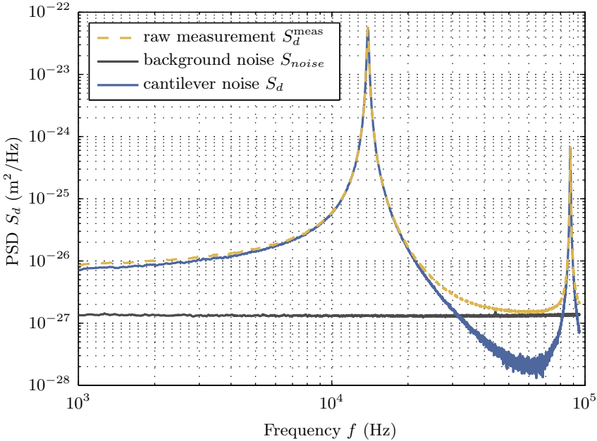
Figure 3.4 – Power spectrum density (PSD) of deflexion of a Budget Sensors BS-Cont cantilever. The thermal noise at the free end of the cantilever is measured in a 1 kHz to 100 kHz range. We clearly see the two first flexural modes of the mechanical beam, well above the background noise of the apparatus acquired on a rigid mirror. The difference between the measurement and the background noise spectra gives a full view of the behavior of the thermal fluctuations of the cantilever in this frequency window.
