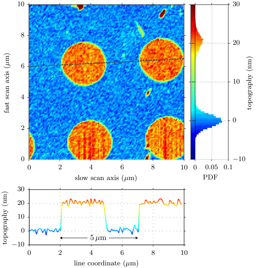
Figure 2.20 – ( 10\ \mu\text{m} \times 10\ \mu\text{m} ) topography image of a calibration sample Budget Sensors HS-20MG acquired in tapping mode. A “smart” flatten filter has been applied to remove the mean slope of each line of the image. The color scale, along with the normalized histogram (PDF) of the topography is shown on the right, and in the bottom graph we plot a profile corresponding to the dashed line in the image. The geometric pattern of the sample (circular pillars, 20 nm high, on a 5\ \mu\text{m} pitch grid) is perfectly reproduced.
