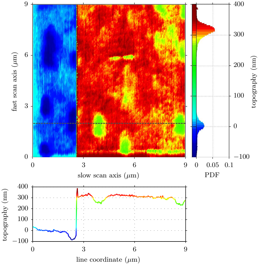
Figure 2.19 – ( 9\mu\text{m} \times 9\mu\text{m} ) topography image of a CD-R (recordable compact disk) sample acquired in contact mode. The mean plane on the sample has been subtracted to the raw image. The color scale, along with the normalized histogram (PDF) of the topography is shown on the right, and in the bottom graph we plot a profile corresponding the dashed line in the image. The artificial step, about 315 nm high, corresponds to an interference fringe hop during the scan.
