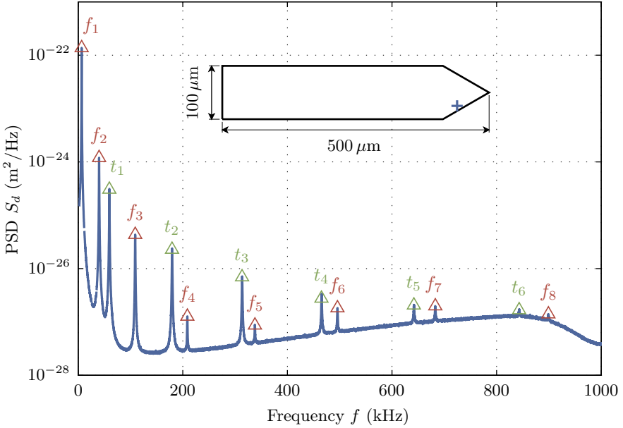
Figure 3.12 – Power spectrum density of thermal noise induced fluctuations on a NanoWorld Arrow TL-Au cantilever. This measurement corresponds to the sensing position indicated by a blue cross on the cantilever sketch. We notice 8 flexural ( f_1 to f_8 ) and 6 torsional ( t_1 to t_6 ) mechanical resonances that we study as a function of the spatial position on the cantilever.
