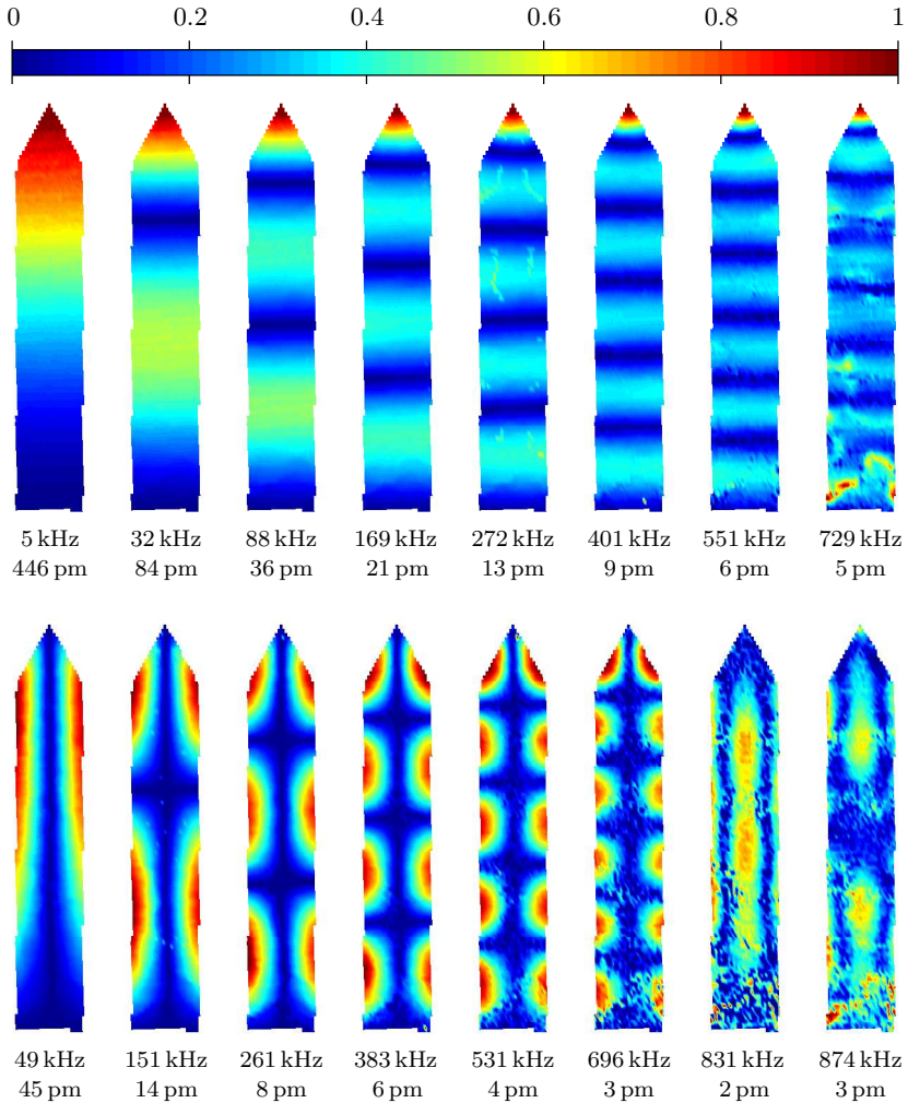
Figure 3.13 — Thermal noise mapping on a 100\ \mu\text{m} \times 500\ \mu\text{m} raw silicon cantilever. We extract from the PSD measured at each point the rms amplitude of 16 different modes, and plot those using a color coded amplitude map (color bar on top of the figure). The resonant frequency and full scale amplitude is given below each map. We easily identify 8 flexural modes and 6 torsional modes from these maps, plus two high frequency resonances of more complex spatial shape.
