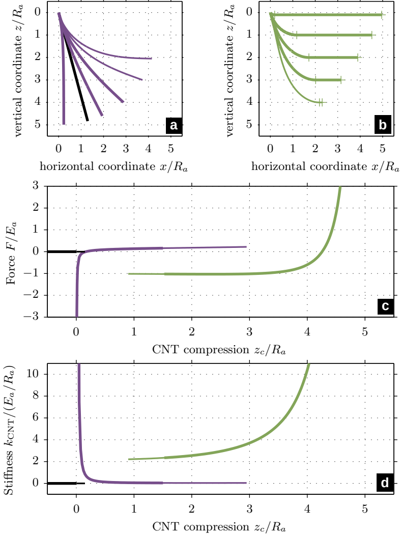
Figure 4.9 – Numerical integration of CNT compression for L = 5R_a and clamped origin in absorbed state. Fundamental and metastable states are respectively drawn as thick and thin lines. Shape for point contact (a) and adsorbed state (b). Force F (c) and dynamic stiffness k_{\text{CNT}} (d) as a function of compression. When cycling Z , the nanotube switches between straight shape (black), weakly bended state (purple), and adsorbed state (green), presenting large force and dynamic stiffness plateau except for the highest compressions, where F \rightarrow +\infty .
