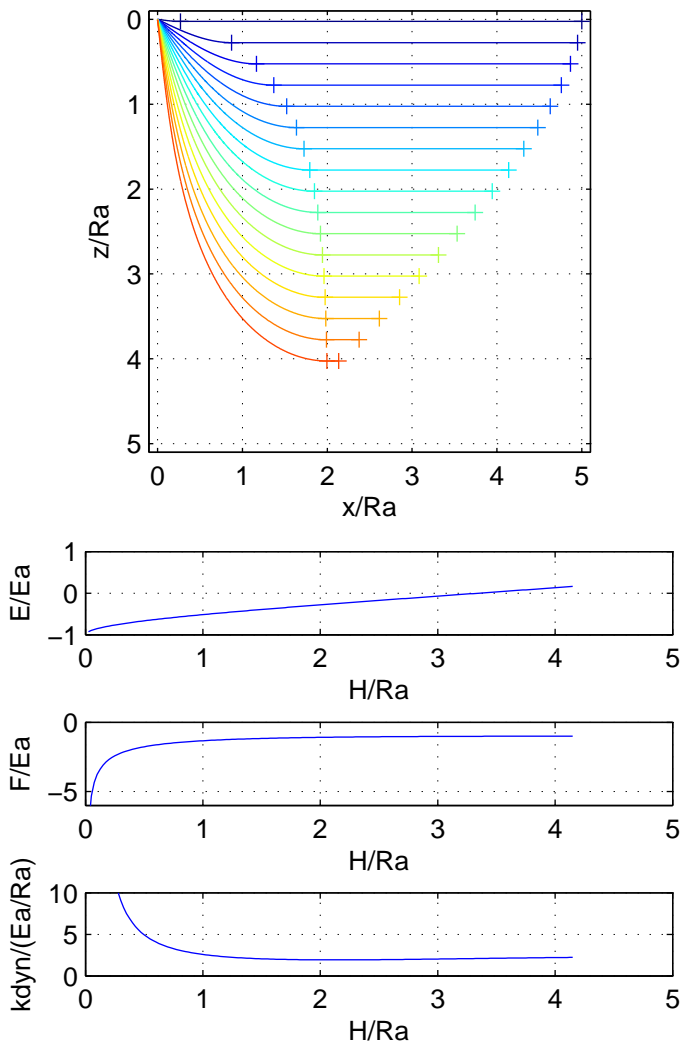
Figure C.1 – Output of script elastica.m : shape of adsorbed Elastica for various origin/substrate distances, and total energy, force and dynamic stiffness versus distance.
