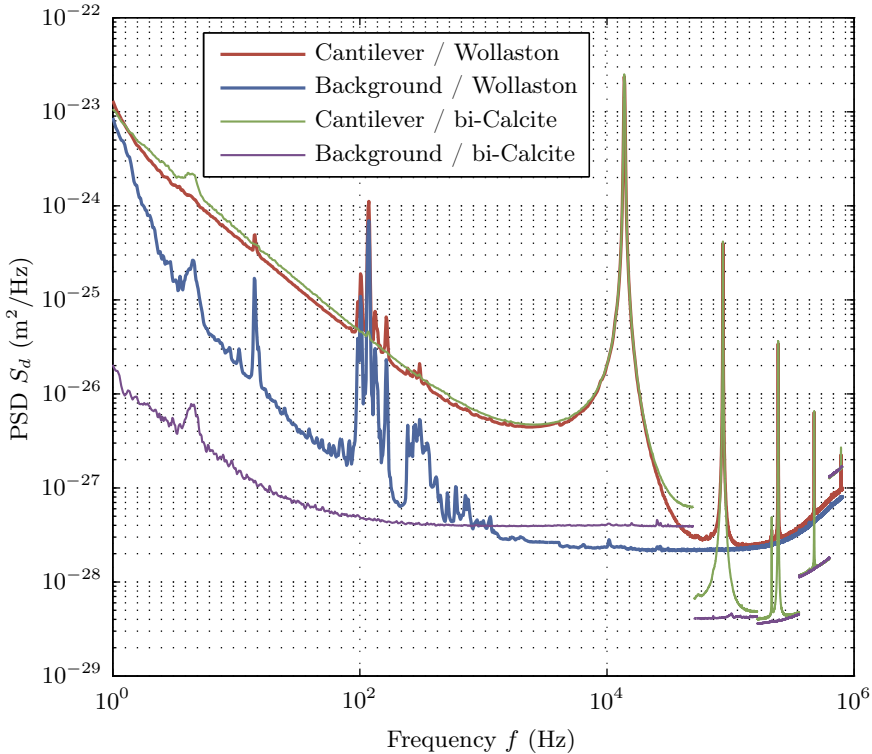
Figure 2.12 – Power spectrum density of deflection measured in the Wollaston and bi-calcite configurations of a golden coated cantilever and on a rigid mirror (background noise). The spectrums measured in the bi-calcite configuration have been corrected to take into account the real position of the laser beams on the cantilever: since the cantilever is longer ( 450\ \mu\text{m} ) than the beam separation ( 140\ \mu\text{m} ), the reference point is not static. A mode dependent correction has been considered.
