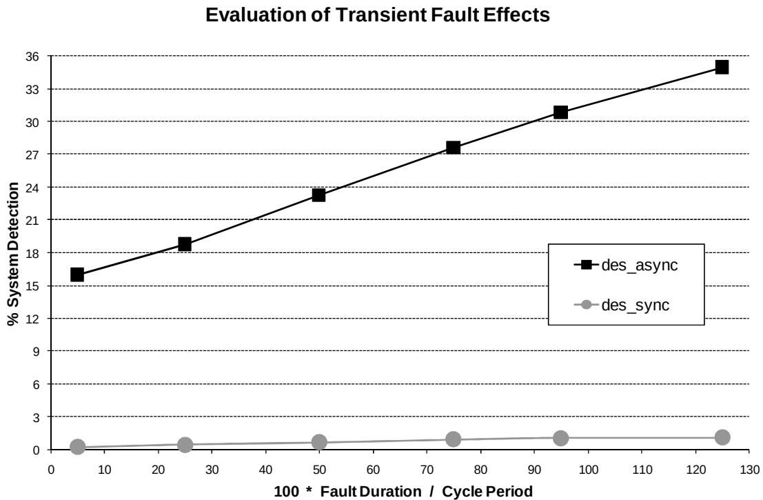
Figure 5.2: A case study on a DES crypto-processor: system's ability for detection in function of transient fault durations
