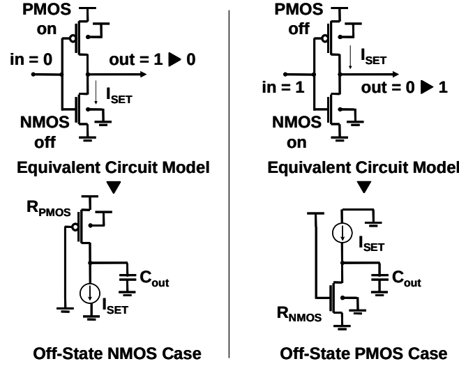
Figure 7.2: Modelling the perturbation-induced transient current I_{SET} that temporally discharges (off-state NMOS case) or charges (off-state PMOS case) the node out
