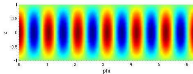
FIGURE 7.7 – \varepsilon = 10^{-1.5} k = 6
