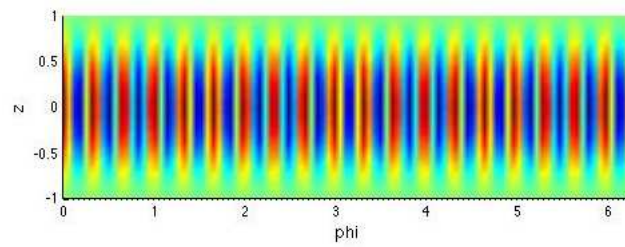
FIGURE 7.10 – \varepsilon = 10^{-3} k = 19
