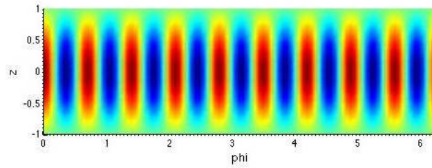
FIGURE 7.8 – \varepsilon = 10^{-2} k = 9
