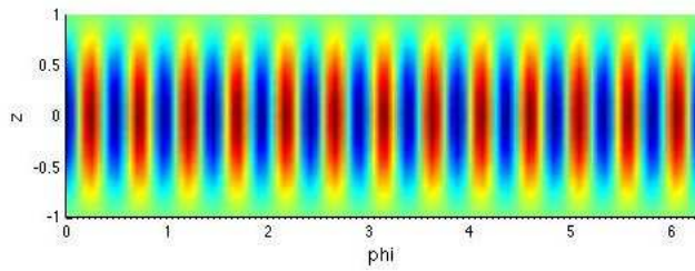
FIGURE 7.9 – \varepsilon = 10^{-2.5} k = 13
