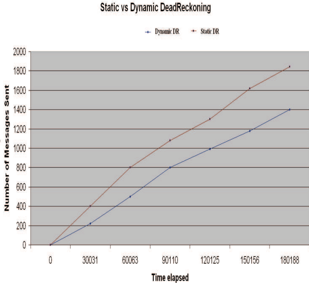
Figure 4.1.3: Number of messages sent in dynamic and static dead-reckoning
