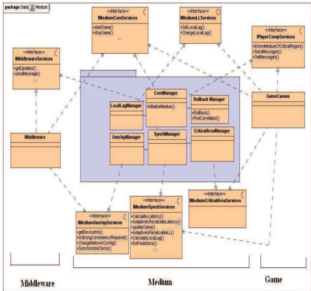
Figure 6.5.7: Detailed Architecture of the Synchronization Medium
