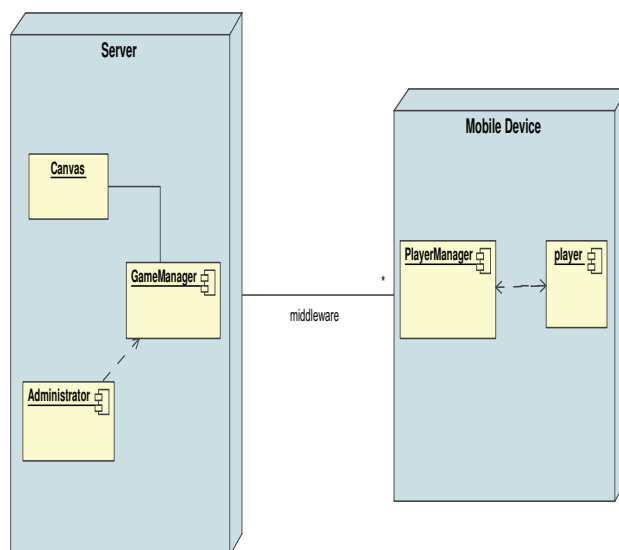
Figure 6.6.10: Deployment of Synchronization Medium in a client-server architecture
