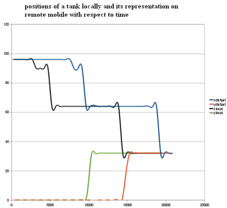
Figure 7.2.6: Position of a tank (local and distant) without any synchronization algorithm
