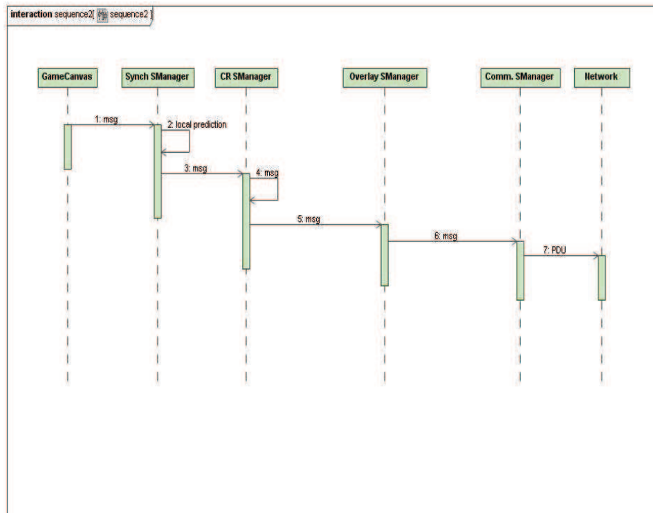
Figure 6.6.9: Message sending by Synchronization Medium
