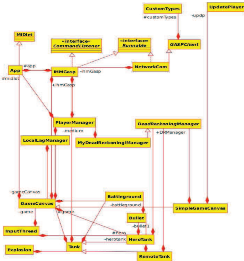
Figure 7.2.5: Class diagram of a multiplayer tank game using the medium
