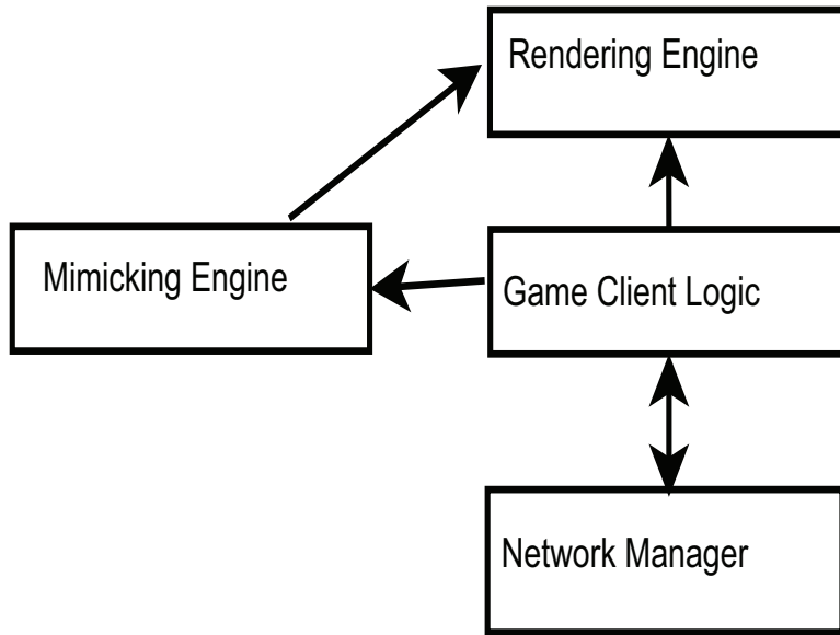
Figure 5.2.2: Client Side Modules for the Game
