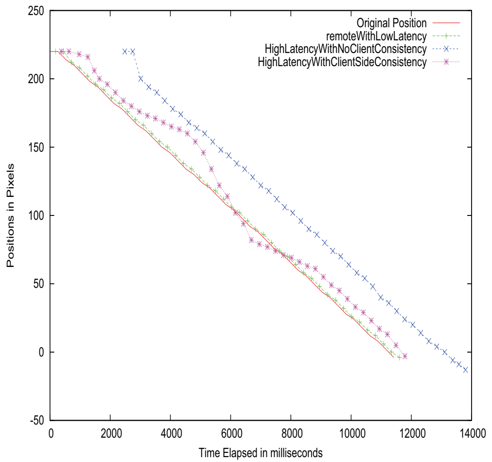
Figure 5.4.6: Comparison of client and server inconsistencies with high and low latency
