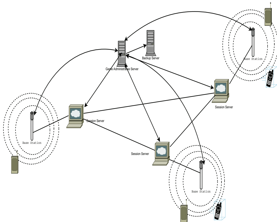
Figure 5.2.1: Session Server based Architecture for 3G mobile Gaming
