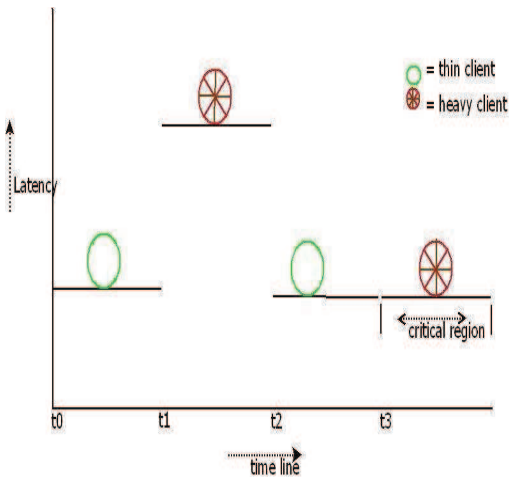
Figure 5.4.5: Dynamic adaptation of the game architecture during the run-time
