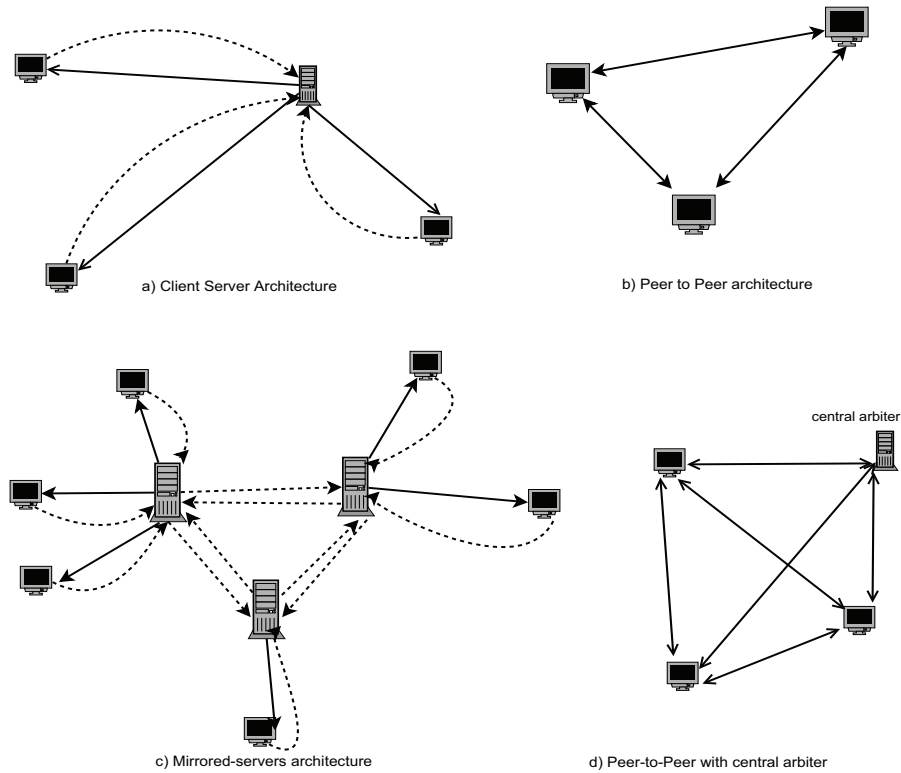
Figure 2.2.3: Different architectures for multiplayer games
