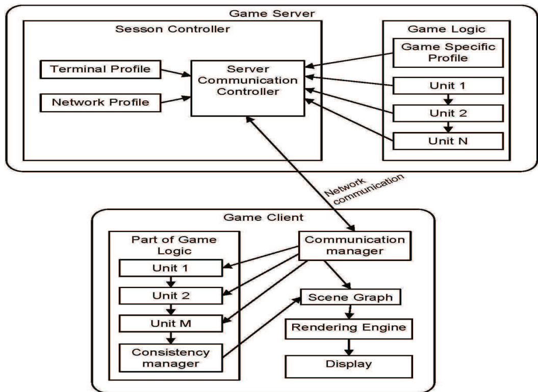
Figure 5.3.4: Hybrid architecture for client-server mobile multiplayer games
