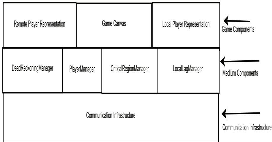
Figure 7.0.1: A Layered Approach to Synchronization Medium
