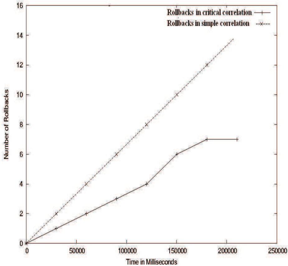
Figure 4.2.8: Rollbacks comparison as a function of time elapsed
