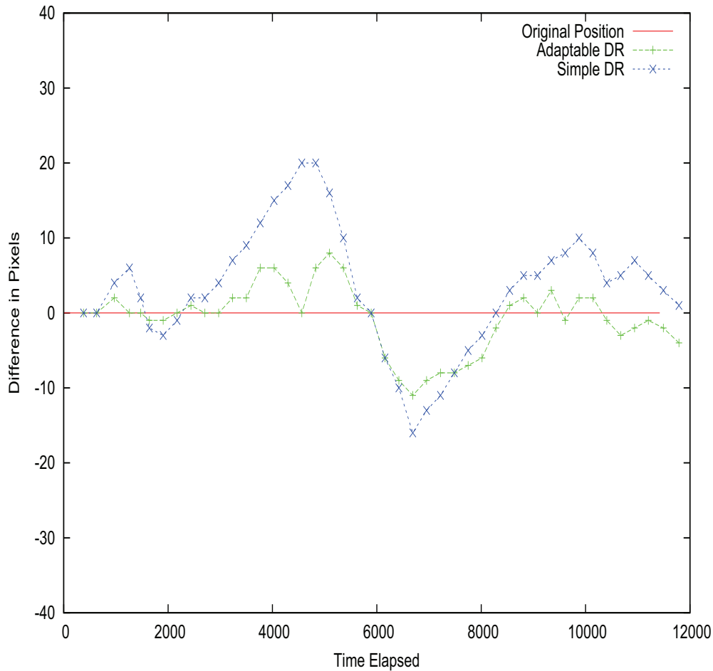
Figure 4.1.2: Adaptable vs Simple Dead-Reckoning
