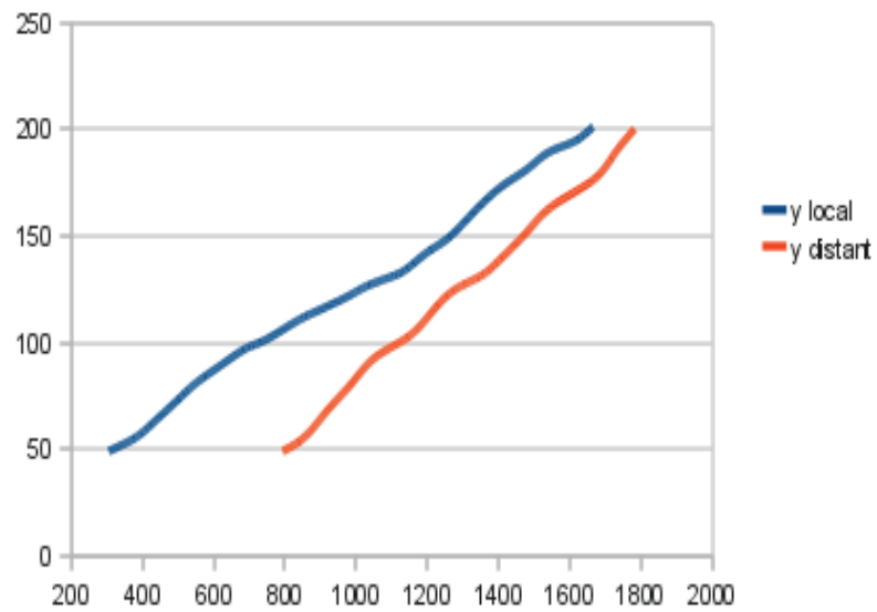
Figure 7.2.8: Position of a tank bullet (local and distant) using dead-reckoning algorithm
