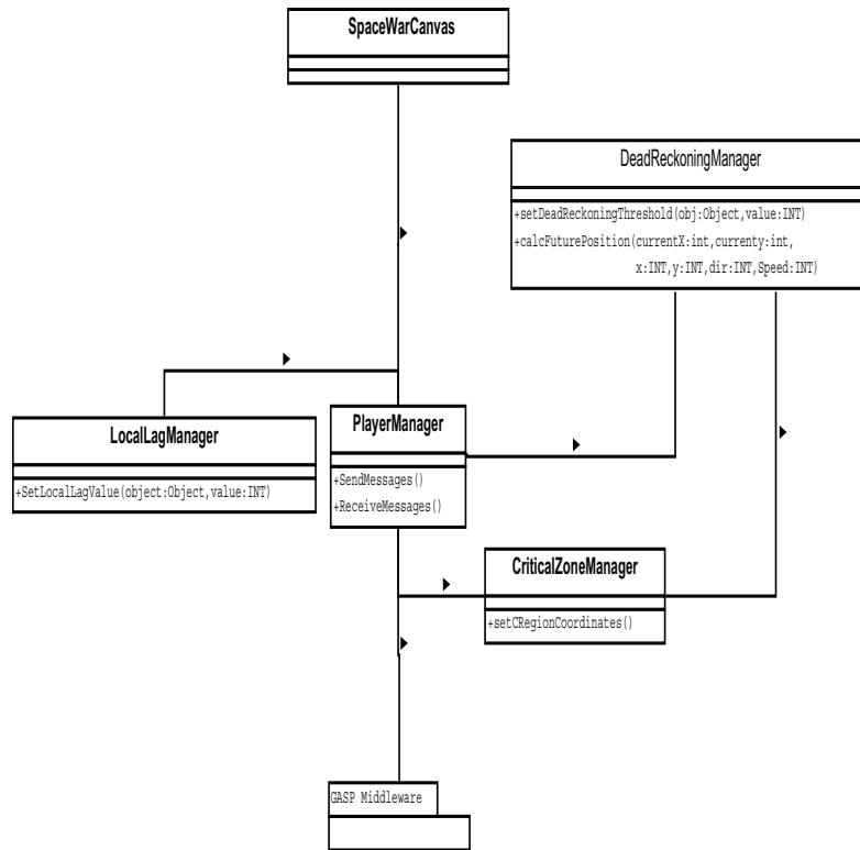
Figure 7.2.3: SpaceWar game using the medium
