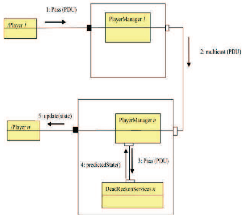
Figure 6.3.5: Dynamic view of message passing in case of Dead-reckoning algorithm
