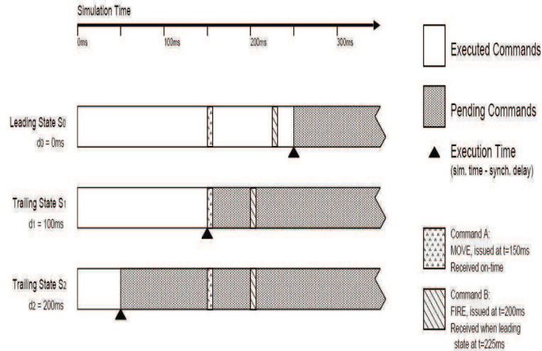
Figure 2.1.2: Trailing State Synchronization Algorithm, taken from (Cronin et al., 2002)
