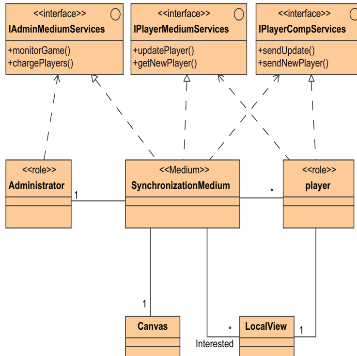
Figure 6.3.2: Abstract specification of Synchronization Medium
