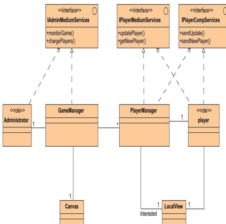
Figure 6.3.3: Introduction of role managers
