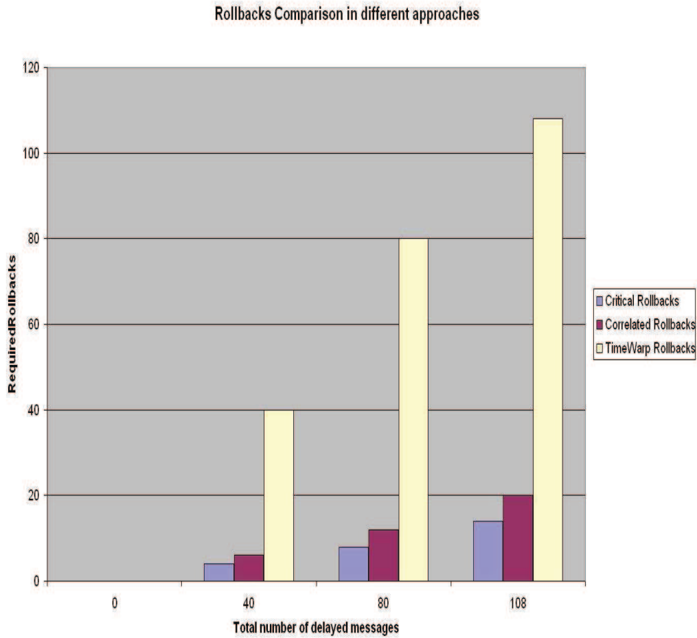
Figure 4.2.6: Rollbacks comparison in three different approaches
