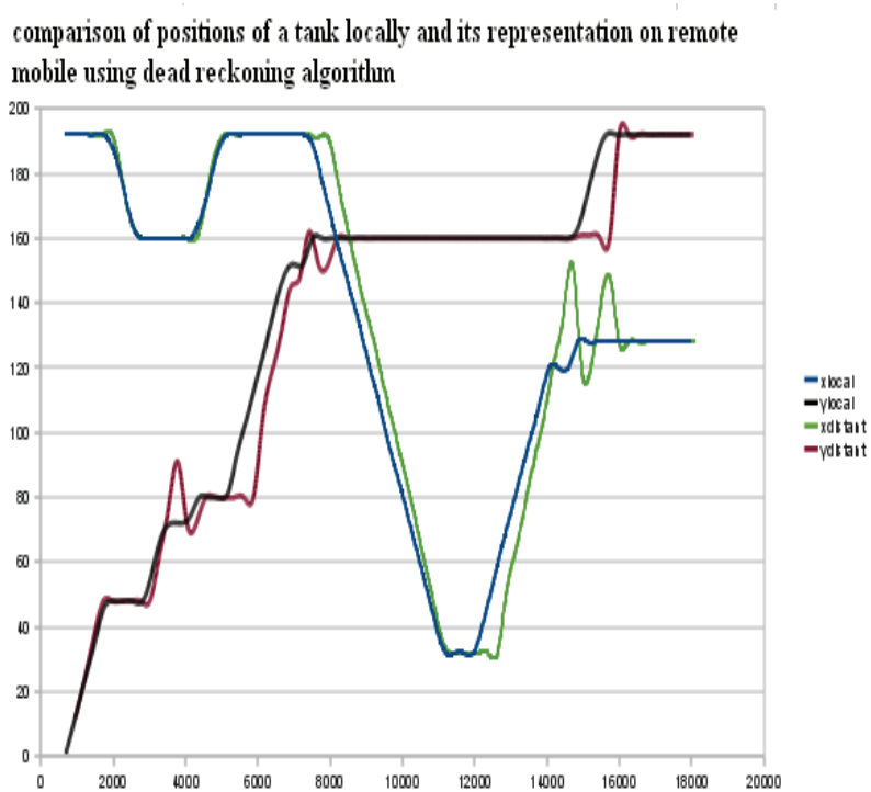
Figure 7.2.7: Position of a tank (local and distant) using dead-reckoning algorithm
