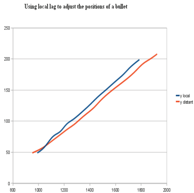
Figure 7.4.9: Position of a tank bullet at local and remote tank
