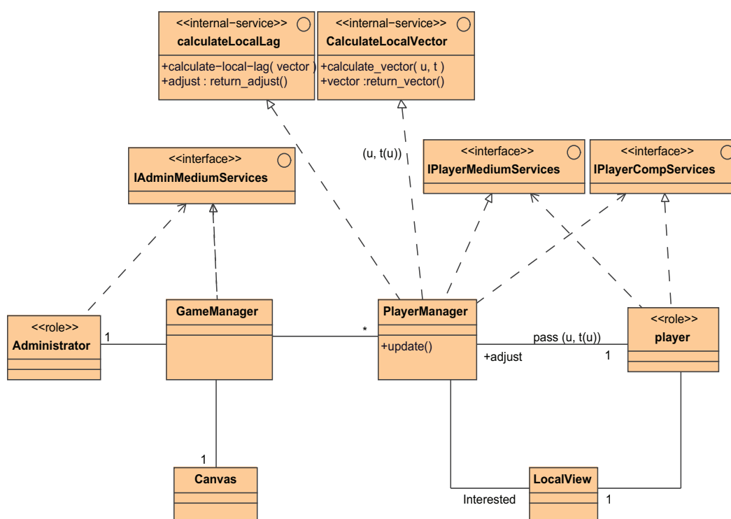
Figure 6.3.6: Synchronization Medium using PC
