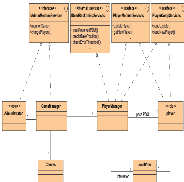
Figure 6.3.4: Synchronization Medium using dead-reckoning algorithm
