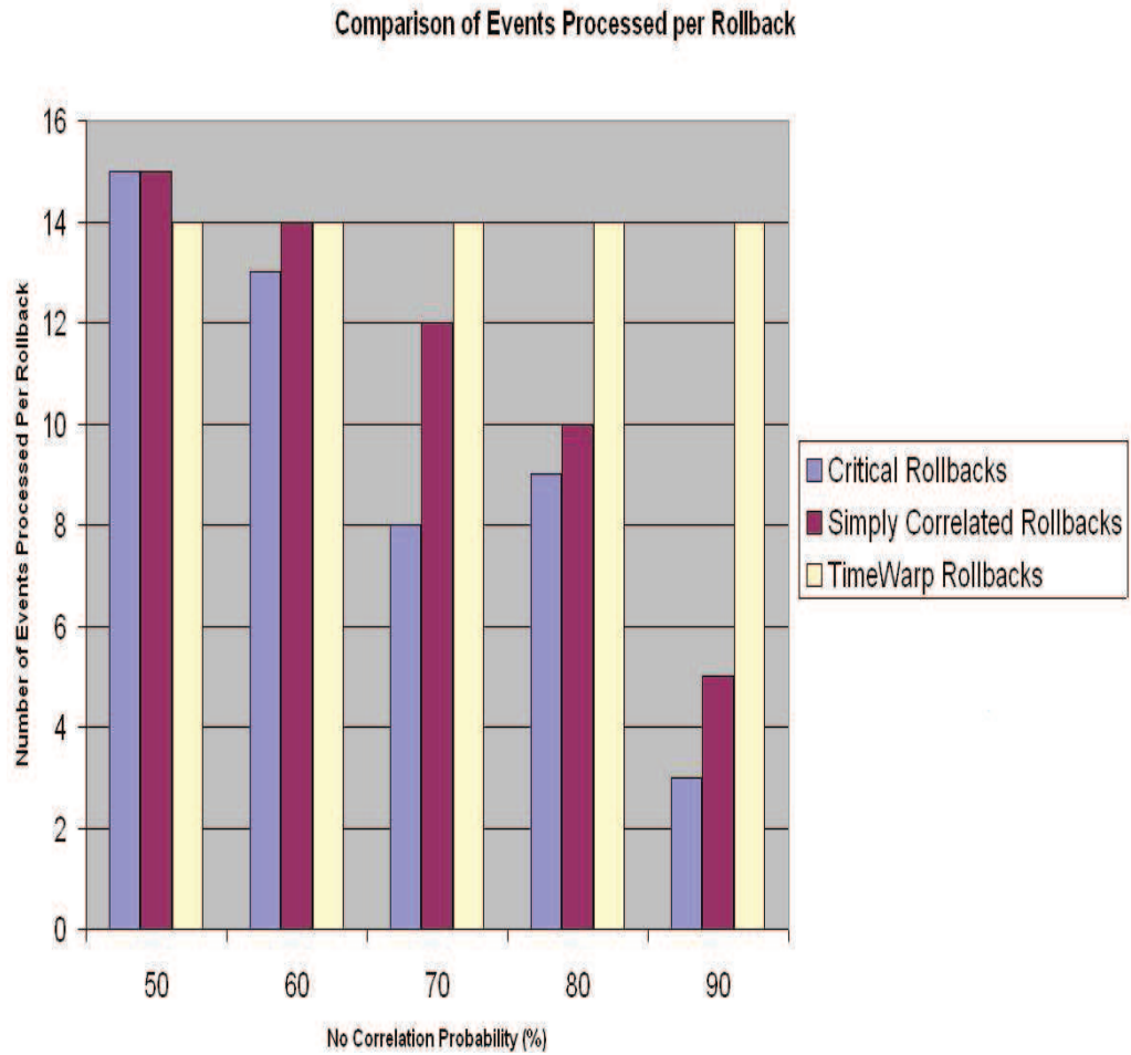
Figure 4.2.7: Comparison of events processed per rollback
