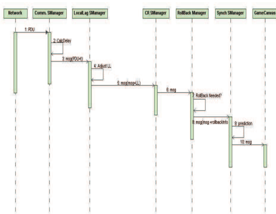
Figure 6.6.8: Message reception by Synchronization Medium
