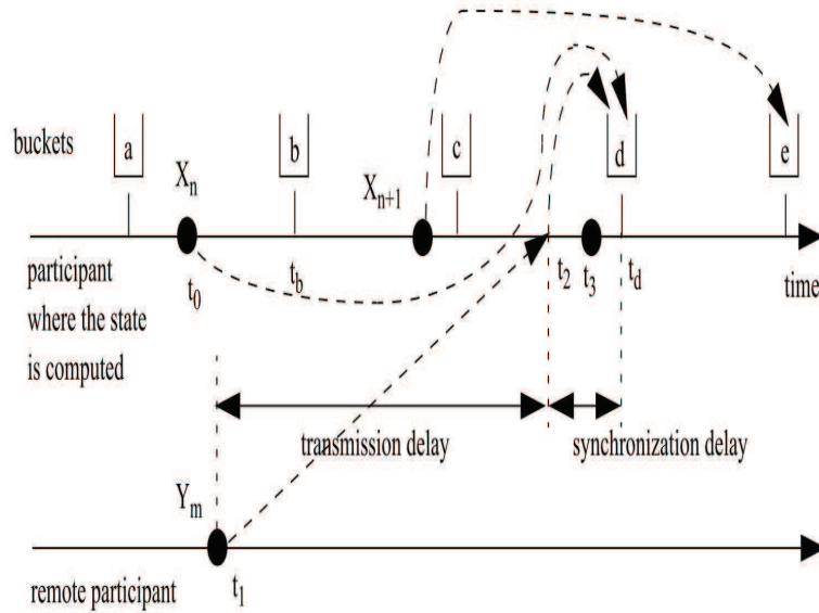
Figure 2.1.1: Bucket Synchronization Approach, taken from (Gautier and Diot, 1998)
