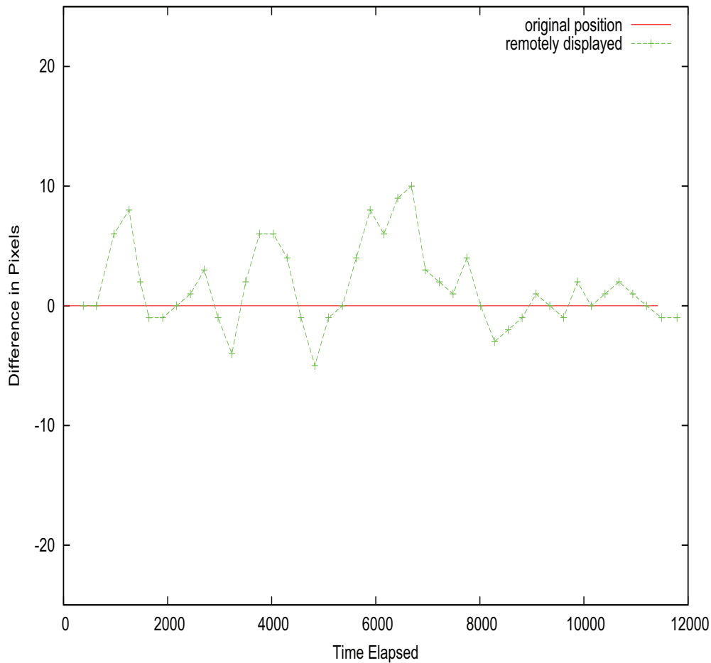
Figure 4.1.4: Consistency of the game using the Critical Region approach
