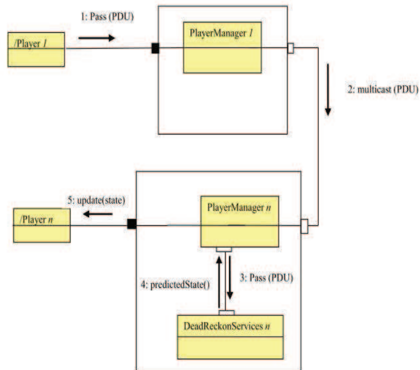
Figure 6.3.5: Dynamic view of message passing in case of Dead-reckoning algorithm
