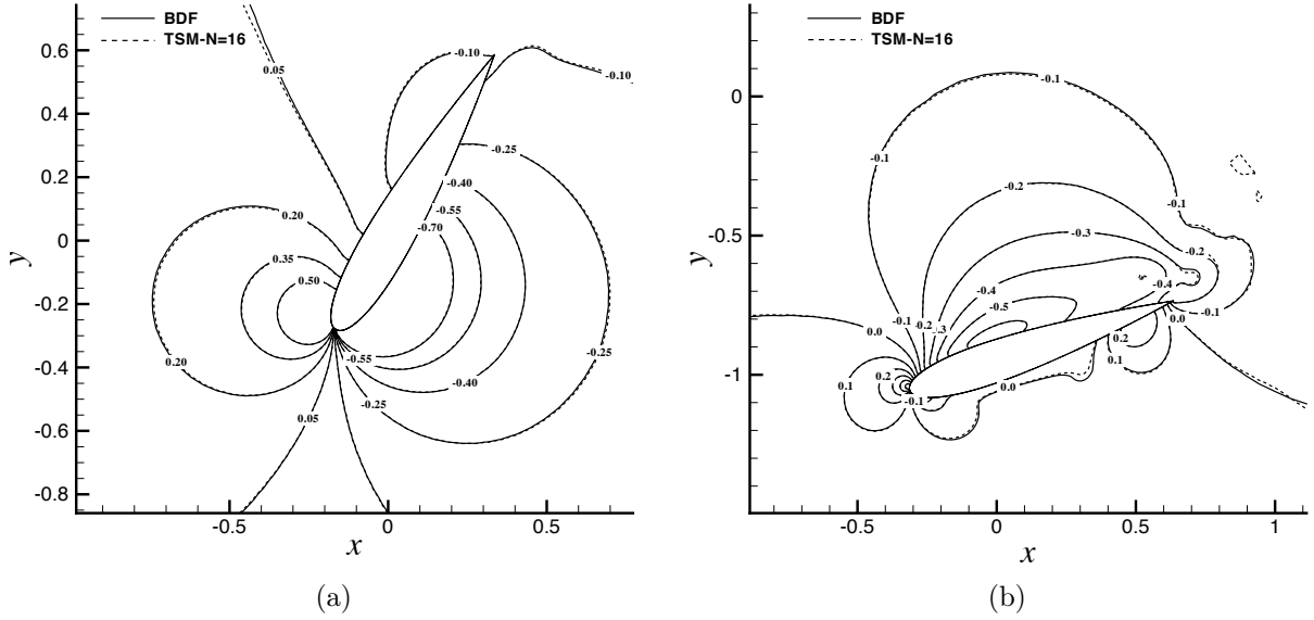
Figure 7.8: Flow problem PH. Reconstructed TSM pressure field ( N=16 ) at time t/T = 0.25 (a) and t/T = 0.45 (b).
