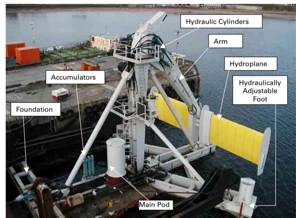
Figure 2.8: Stingray tidal turbine device [71]
